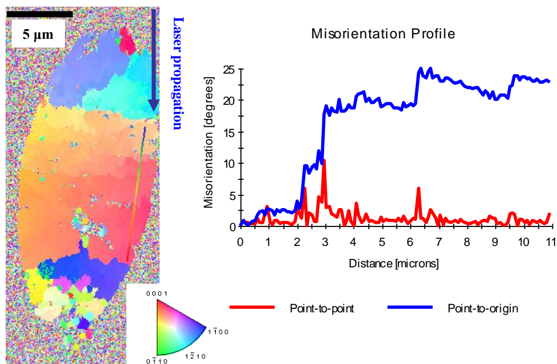
Figure 5.5: EBSD map (left) and the misorientation profile (right) along the left color line of cross section of the written lines below the glass surface 350 \mu\text{m} after cleaved, polished and etched with 10% HF for 2 mins. The curve “point-to-point” indicates the profile of the orientation
