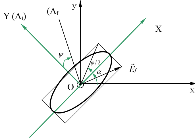
Figure A.4: Action of the \lambda/4 wave plate on elliptical polarization after the plate birefringence. A_i and A_f indicate the positions of the analyzer for the extinction before and after the introduction of the \lambda/4 waveplate, respectively.
