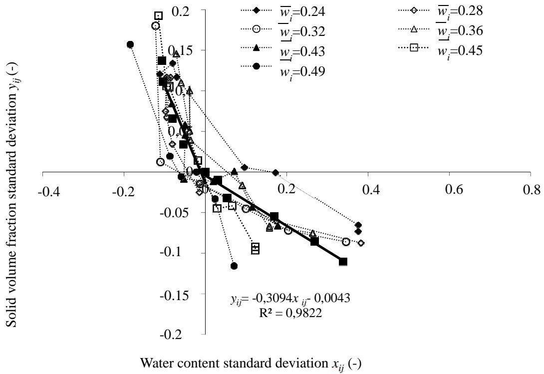
Figure IV.28. Solid volume fraction standard deviation of agglomerates according to their water content standard deviation.
