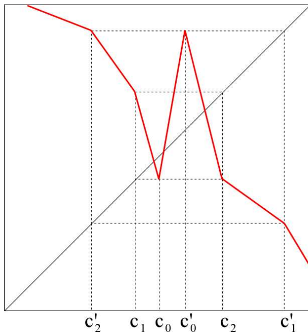
Figure 3.1: A continuous and piecewise affine map f_{\text{ana}}|_{\mathbb{R}} which realizes \mathcal{R}_{\text{ana}}
