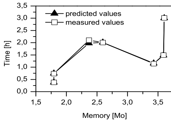
Figure 5.19: Computation time prediction for various simulations when TLM cells model dielectric media - the memory space required for storing 2^*X^*Y^*18^*8 bytes is smaller than the processor cache memory size.
