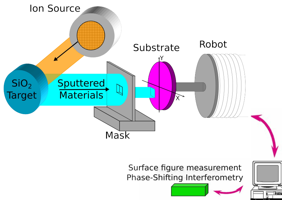
Figure 5.1: The corrective coating technique
