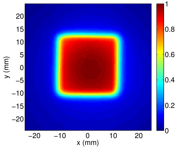
Figure 5.2: Normalized deposition imprints through a 21.5 mm square mask.
