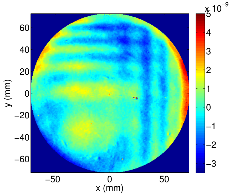
Figure 4.24: Surface figure of the curved surface (n°1) of ETM02 measured at LMA, piston, tilt, RoC removed with off-centered fringes. Flatness = 0.97 nm RMS.
