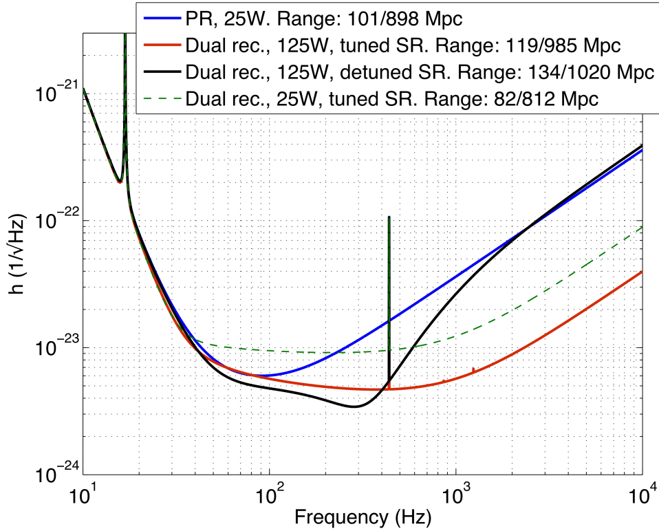
Figure 1.10: Advanced Virgo sensitivity for the different possible scenario in the Advanced Virgo configuration. In the legend, the inspiral ranges for BNS and BBH (each BH of 30 M_{\odot} ) in Mpc are reported, from [23].
