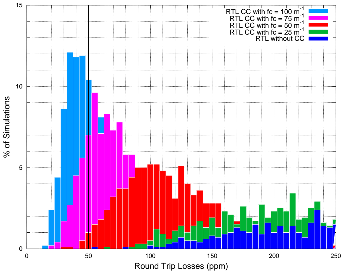
Figure 3.12: Histogram of the RTL in the Advanced Virgo cavity with original mirror surfaces flatness of 4 nm RMS and corrected with a frequency cut of 25 \text{ m}^{-1} , 50 \text{ m}^{-1} , 75 \text{ m}^{-1} and 100 \text{ m}^{-1} .
