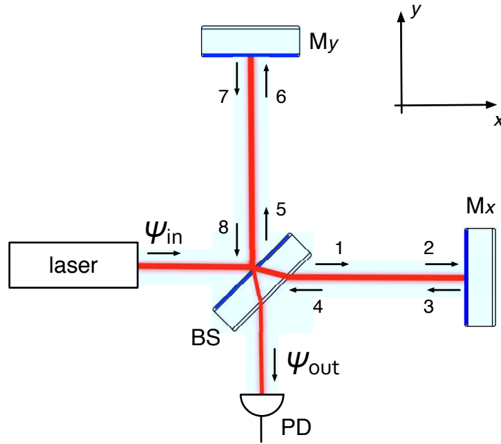
Figure 1.3: Optical scheme of the Michelson interferometer. The light field notation are reported as well as the different elements: the laser source, the beam splitter (BS), the two end mirrors (Mx and My) and the output photodiode (PD).
