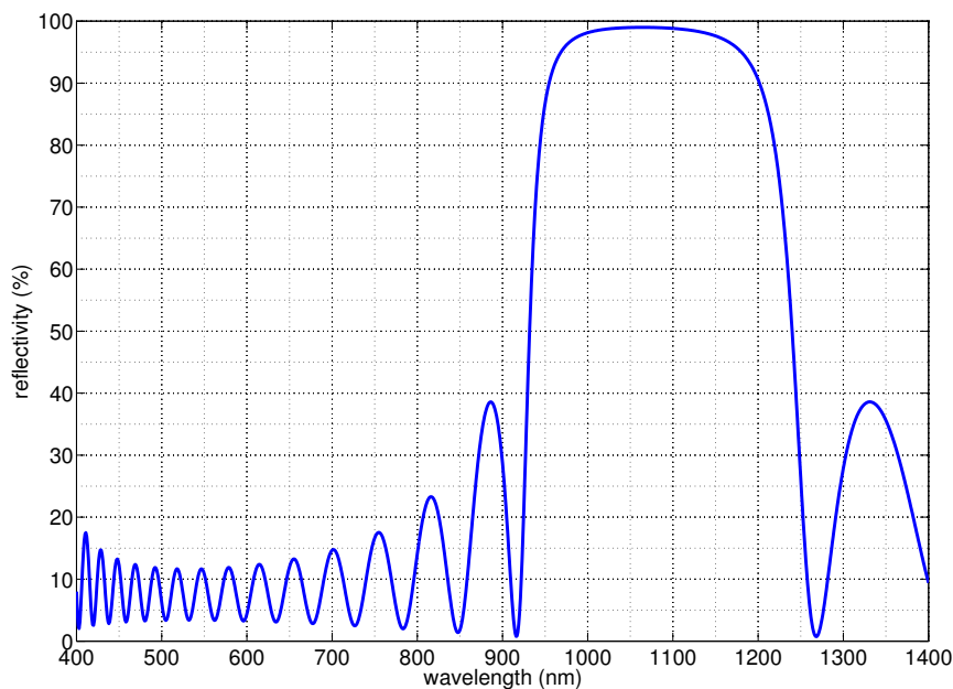
Figure 6.3: Reflectivity of a quarter-wave multilayer coating with 18 layers.
