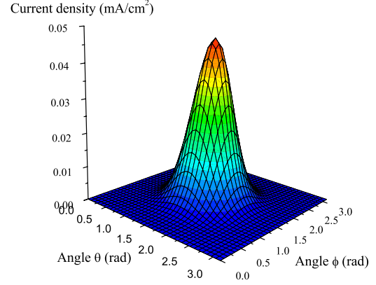
Figure 4.8: Reconstructed 3D ion current density distribution in the plume of the PPI thruster ( S_0 geometry, 300 V, 0.8 mg/s).
