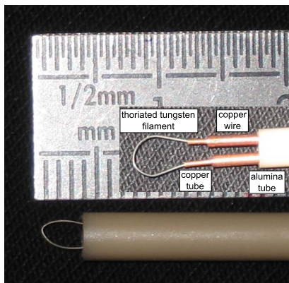
Figure 5.2: Picture of the emissive probe. Also shown are all the different elements necessary to built the probe.
