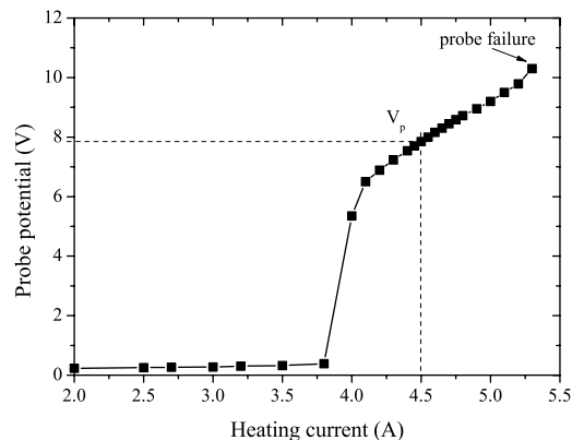
Figure 5.3: Emissive probe potential against the heating current in the far-field plume of the PPS ® 100-ML thruster.
