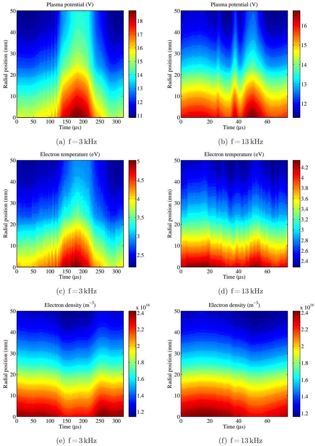
Figure 6.9: Evolution in time and space (radial direction) of V_p , T_e and n_e for the two different frequencies at 100 mm downstream thruster exit plane. The thruster is operated at U_d = 200 V, \dot{m}_a = 1.0 mg/s (Xe).
