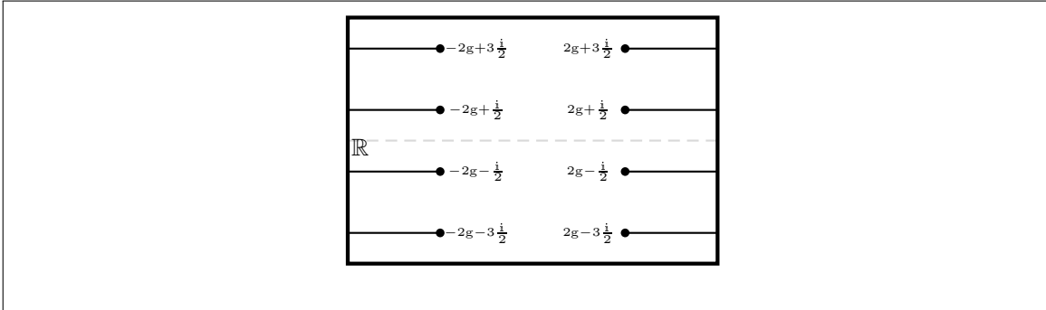
Figure IV.2: The cut structure of the function \mathcal{F} .
