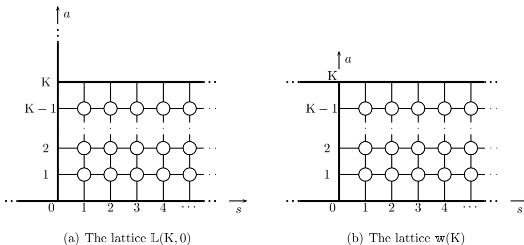
Figure III.3: The lattices \mathbb{L}(K, 0) and w(K) corresponding to the group GL(K)
