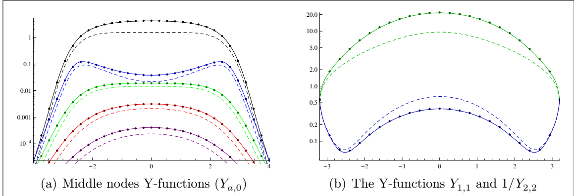
Figure IV.6: Numerical Y-functions for Konishi state at g = 1.6
