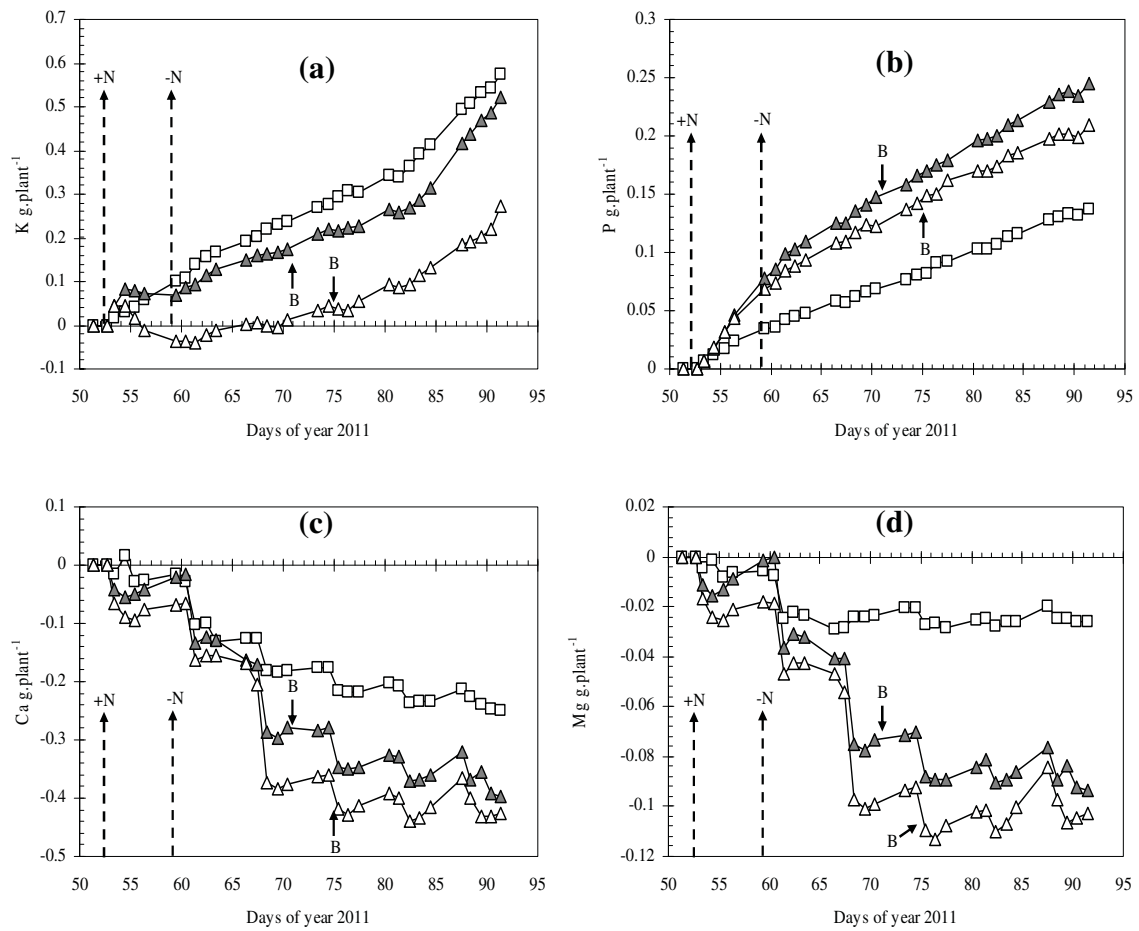
Fig. 3.34 : Cumulate potassium (a), phosphorus (b), calcium (c), and magnesium (d) uptake ( \text{g} \cdot \text{plant}^{-1} ) during experiment period 2011, in Control and Control/out (□), N-Pulse (△), and N-Pulse/out (▲) conditions. The arrows represent experiment started during supplying nitrate to N-Pulse and N-Pulse/out treatments (N+). On day 59 solution was changed to the solution without nitrate in N-Pulse and N-Pulse/out treatments (-N), respectively. First time of bud break for N-Pulse and N-Pulse/out treatments (B).
