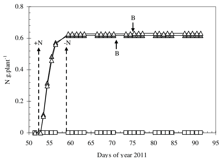
Fig. 3.33 : Cumulated nitrogen uptake ( \text{g.plant}^{-1} ) during experiment period 2011, Control and Control/-out ( \square ), N-Pulse ( \Delta ), and N-Pulse/-out ( \blacktriangle ). The arrow represents experiment start supplying nitrate to N-Pulse and N-Pulse/-out treatments (N+). On day 59 solution was changed to a solution without nitrate for N-Pulse and N-Pulse/-out treatments (-N), respectively. The first time of bud break in N-Pulse and N-Pulse/-out treatments (B).
