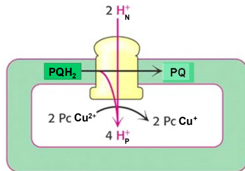
Figure 3.21 : Proton movement at Complex II
