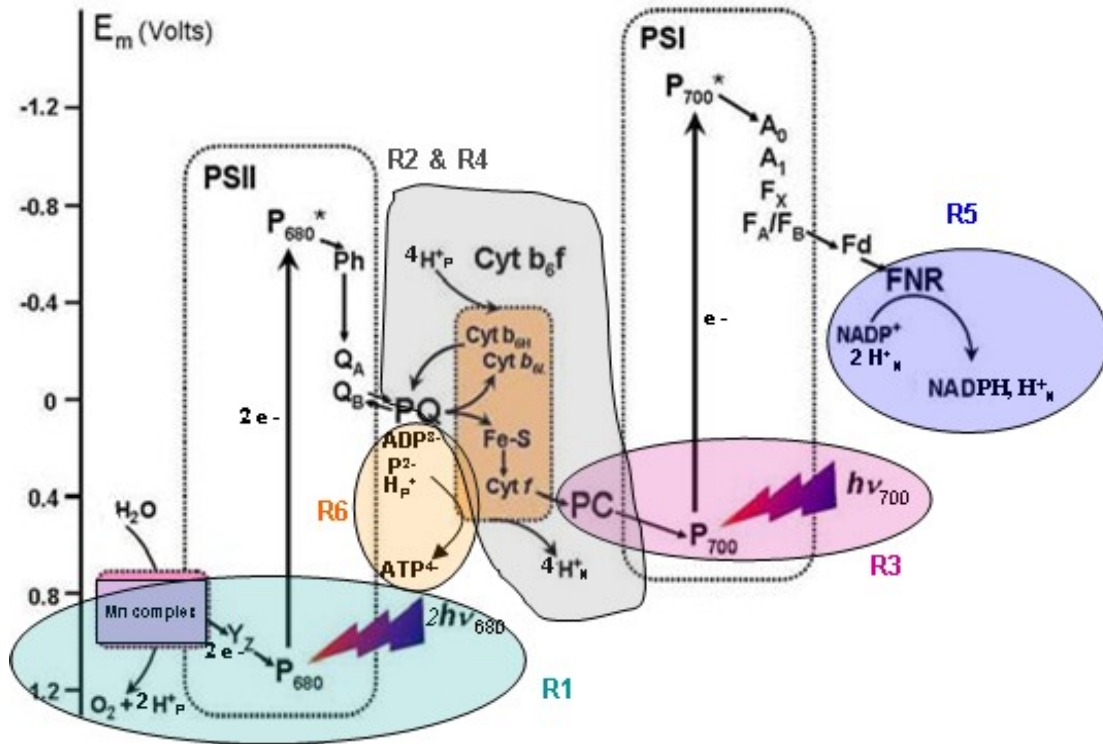
Figure 3.20: Z-scheme of photosynthesis Photosynthetic electron flow from H_2O to NADPH . The relative redox potentials show that P_{680} and P_{700} are highly oxidising. Their excited forms ( P_{680}^* and P_{700}^* ) of the reaction centre pigments are highly reducing and located in the upper part of the diagram. Electrons are transferred from water, through Y_Z to reduce P_{680}^+ . Further, P_{700}^+ is reduced by electrons from PSII, transferred via plastoquinol, through Cyt b_6f complex and plastocyanin (PC). (Picture is adapted from Feyziyev, 2010).
