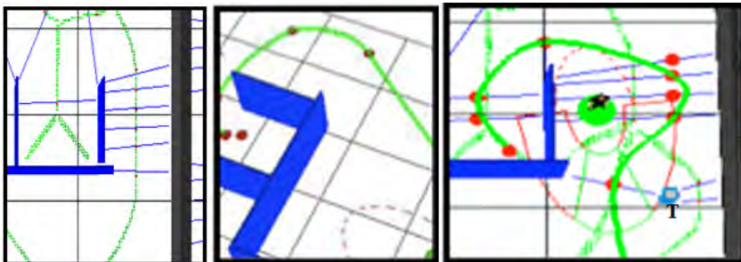
Figure 6.11: (a) Initial Voronoi Diagram and clearance (IBLs), (b) initial planned path, (c) during execution the updated clearance information and deviated path due to presence of previously unknown trash bin, marked as T.
