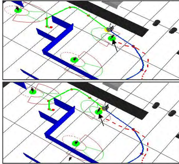
Figure 6.28: The human, indicated by black arrow, switching from behind to the left side of the robot to accompany the robot instead of following it. The robot did not show any reactive deviation in its path.
