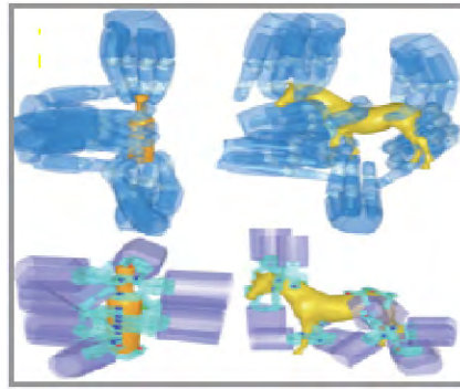
Figure 5.2: Subset of generated grasp set for objects of different shapes, for anthropomorphic hand (top) and for robot's gripper (bottom). (see [Saut 2012])
