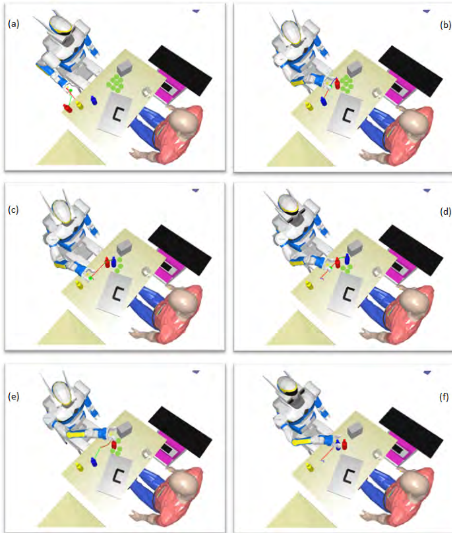
Figure 8.24: Demonstration of backtracking at geometric level to find a feasible solution for making two bottles (red and blue) accessible to the human. Maximum allowed effort level for both the agents is set as Arm\_Torso\_Effort . (a) The initial scenario, and the green circles show the autonomously found current candidate placement space. (b) Solution found for validating the first node of symbolic plan (see figure 8.22). (c)-(d) Failed to find a feasible path to make accessible second bottle, corresponding to second node of symbolic plan. Instead of returning with a fail message, the geometric layer backtracked to find alternate solution for previous actions, which might make the current action feasible. (e) By backtracking in candidate space of putting the first bottle, it found another placement for first bottle, by respecting the constraints. (f) With this new solution of making first bottle accessible, now the planner found a feasible placement for making second bottle also accessible to the human. Hence, returned a success for the entire plan to the symbolic layer.
