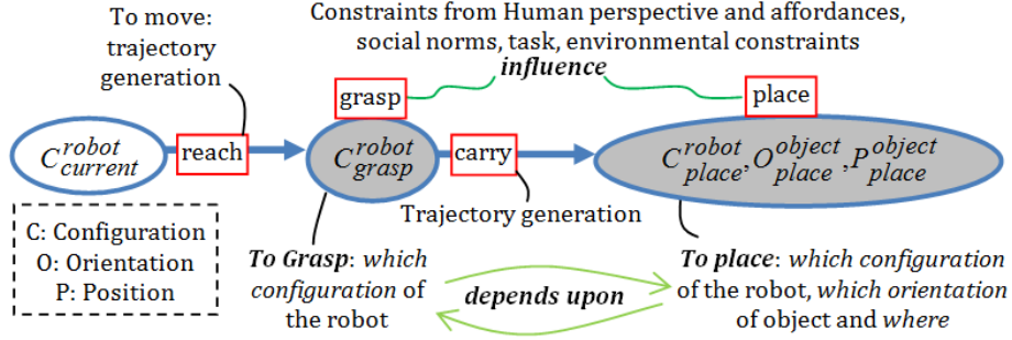
Figure 7.2: A typical pick-and-place task. It shows the requirement to synthesize C , O , and P components. It also shows different influencing components and inter-dependencies.
