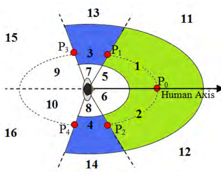
Figure 6.19: Different sub-regions, their IDs and the candidate passing by points (red circles) around the human.
