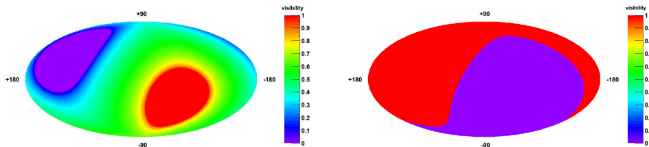
Figure 3.9: The visibility of ANTARES (left) and IceCube (right) in the Galactic Coordinates.
