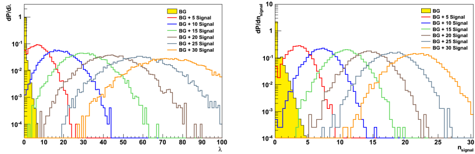
Figure 5.29: \lambda value distributions (left) and fitted numbers of events (right) of a source at declination = -25^\circ .
