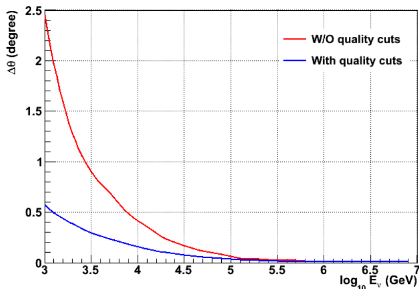
Figure 3.4: Median angular difference between the neutrino and the muon directions as a function of the neutrino energy. The red curve represents the up-going simulated neutrinos (seen by ANTARES) and the blue one represents those which respect the quality cuts optimized in Chapter 5.
