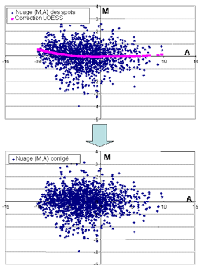
Figure 69: Correction LOWESS
