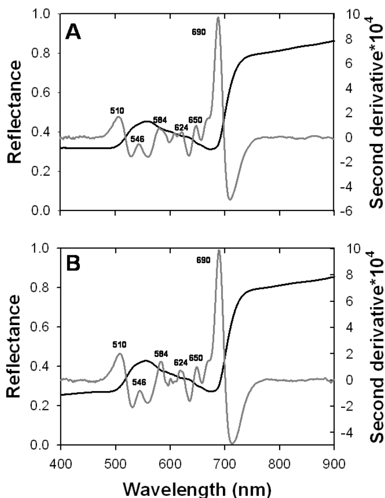
FIGURE 2.11 – A : Reflectance spectrum (black) and second derivative (grey) of un fouled leaves of Zostera noltii collected in the upper intertidal zone in July 2009. B : Reflectance spectrum (black) and second derivative (grey) of fouled leaves of Zostera noltii . Second derivative peaks show the position of the specific absorption bands of the leaves
