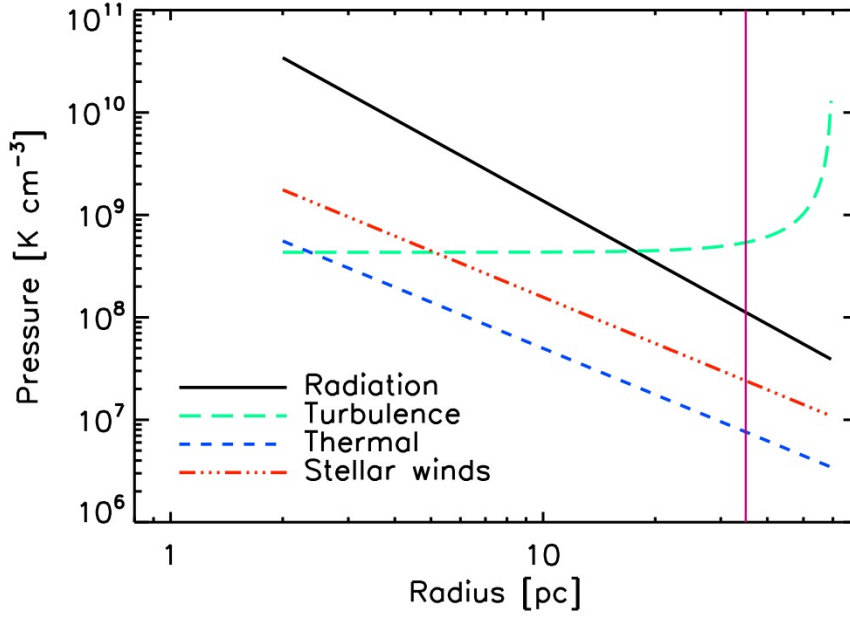
Figure 6.12: This figure illustrates the dependence of the different pressures on the radius of the GMC in SGMC 4/5. The black line corresponds to the radiation pressure, the green line to the turbulent pressure, the blue line to the thermal pressure and the red line to the thermal pressure of the X-ray emitting plasma (driven by stellar winds), respectively. The vertical line marks the radius measured from the Br \gamma emission of 35 pc.
