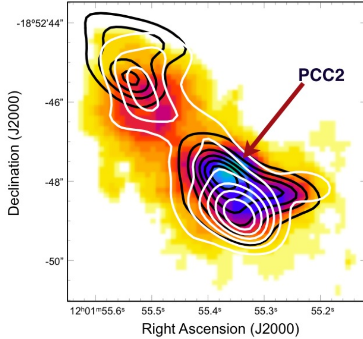
Figure A.6: The color image is the \text{H}_2 1 – 0 S(1) flux map from SGMC 1. Black and white contours are the \text{CO}(3-2) emission integrated in the velocity range 1300 - 1415 \text{ km s}^{-1} and 1415 - 1490 \text{ km s}^{-1} , respectively. I highlight PCC2.
