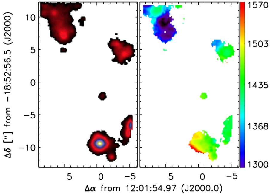
Figure 3.16: \text{Br}\gamma morphology and kinematics across the overlap region. It is observed that all SGMCs are associated with ionized gas.
