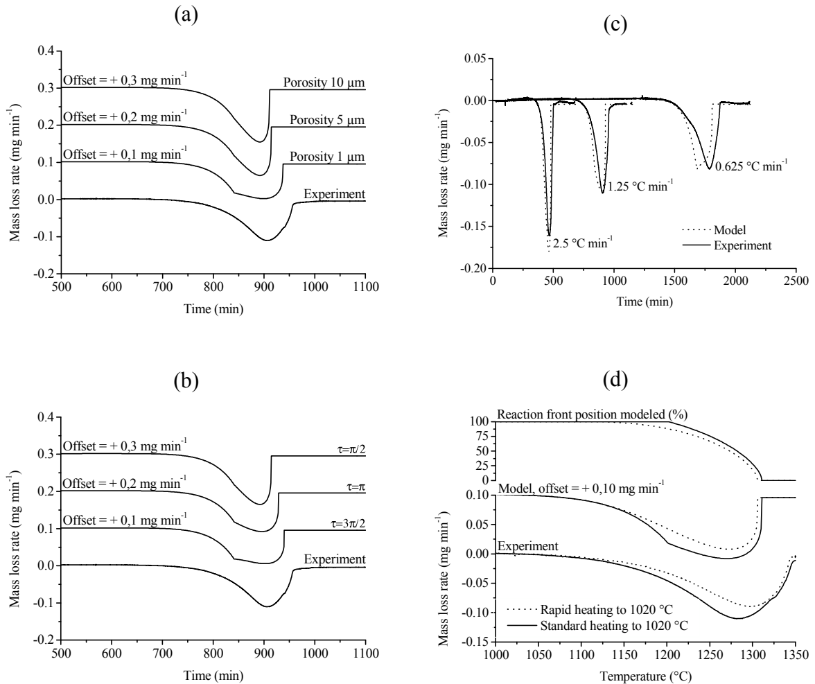
Figure III.9: Experimental and modeled rate of mass loss. Constant model parameters are p = 0.4 , e_{\text{SiO}_2} = 0.52 \text{ nm} , P_{\text{H}_2\text{O}}^{\text{zr}} = 1.8 \text{ Pa} , and z_f = 40 \text{ mm} . (a) Effect of the pore size for a heating rate of 1.25 \text{ }^\circ\text{C min}^{-1} and a tortuosity of \pi/2 . (b) Effect of the tortuosity for an heating rate of 1.25 \text{ }^\circ\text{C min}^{-1} and a pore size of 5 \text{ }\mu\text{m} . (c) Effect of the heating rate for a pore size of 5 \text{ }\mu\text{m} and a tortuosity of \pi . (d) Effect of the passive oxidation, occurring below 1020 \text{ }^\circ\text{C} , on the reaction front position and the rate of mass loss during the silica reduction. Above 1020 \text{ }^\circ\text{C} the heating rate is 1.25 \text{ }^\circ\text{C min}^{-1} . The pore size is 5 \text{ }\mu\text{m} and the tortuosity \pi .
