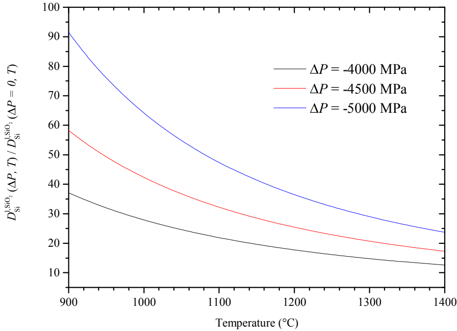
Figure IV.21: D_{\text{Si}}^{1\text{SiO}_2}(\Delta P, T) / D_{\text{Si}}^{1\text{SiO}_2}(\Delta P=0, T) as a function of the temperature for several pressure drops, \Delta P .
