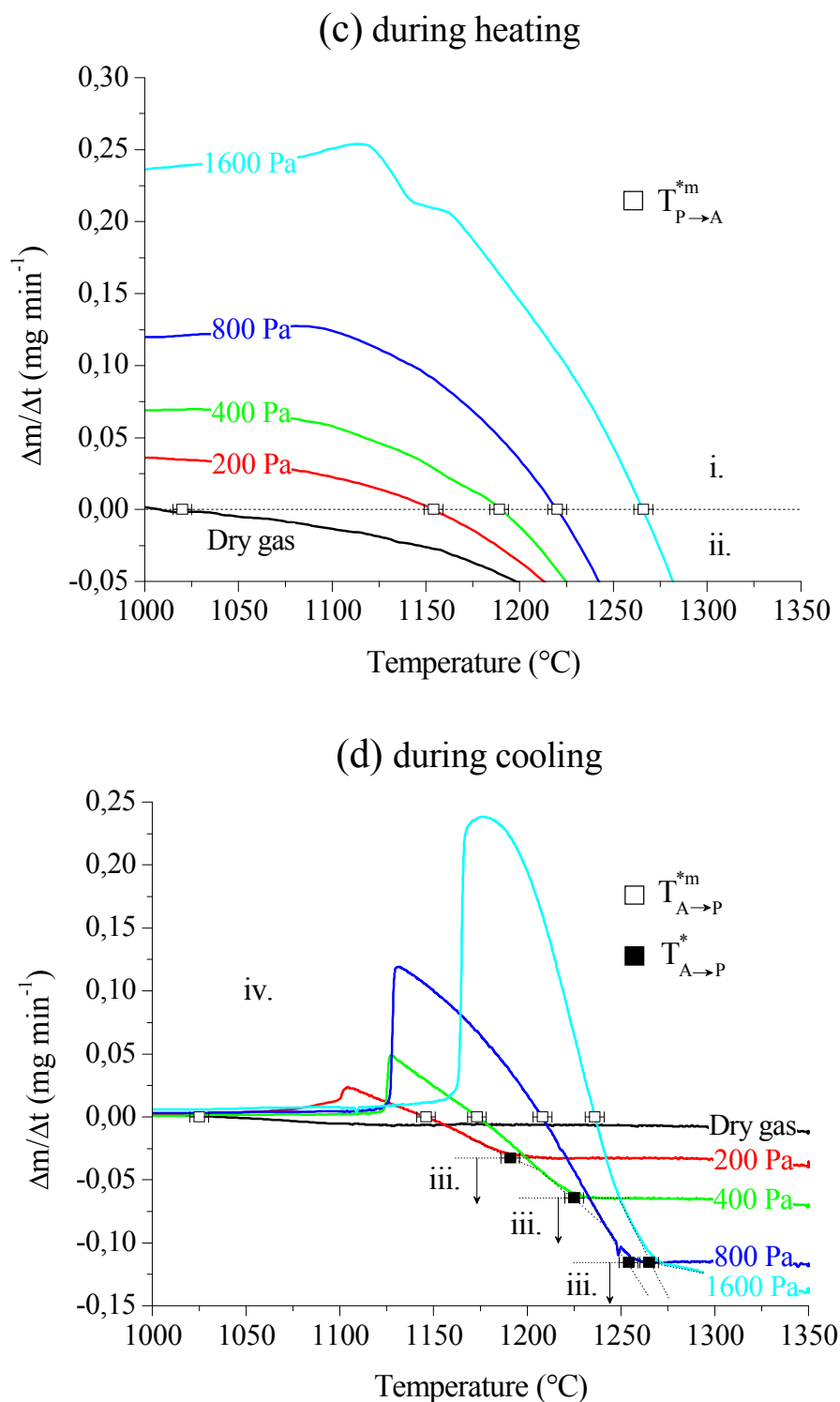
Figure V.7 (following): TGA curves of VF powder compacts under 2 l h -1 He-4mol.% H 2 atmosphere, dry or humidified ( P_{H_2O}^{Probe} = 200, 400, 800 and 1600 Pa). (c) Mass variation rate during heating (passive to active transition). (d) Mass loss rate during cooling (active to passive transition).
