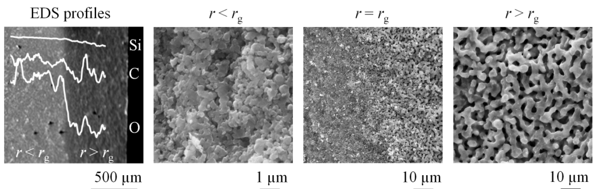
Figure IV.5: Grain coarsening position, r_g , and calculated reaction front position, r_r , as function of time for a silicon powder compact, heated up to 1350 °C with a heating rate of 1.25 °C \text{min}^{-1} and a holding time of 3 h under He-4 mol.% \text{H}_2 . EDS profiles and silicon micrographs for a sample quenched at t = 920 min, T = 1315 °C, are given at different positions from the grain coarsening front position.
