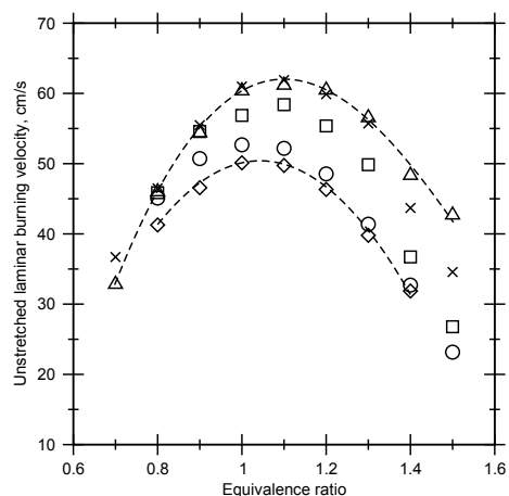
Figure X.3: Laminar burning velocities of ethanol/isooctane/air mixtures at atmospheric pressure and temperature of 373 K for different ethanol mole fraction \epsilon . Symbols: experiments, dashed lines: correlation for pure fuels. Triangles up: E100; cross: E85; squares: E50; circles: E20; diamonds: E0.
