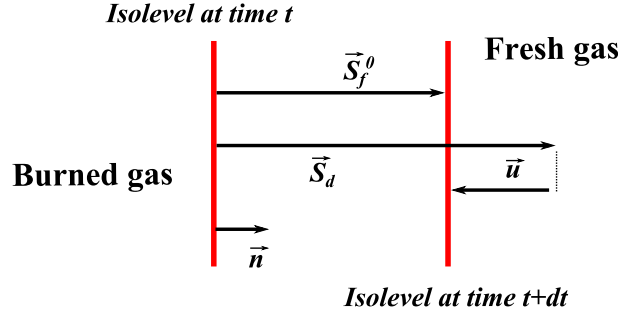
Figure II.5: Illustration of flame layers and corresponding velocities: absolute speed \vec{S}_f^0 , fresh gas velocity \vec{u} (“seen” by the isothermal considered), and displacement speed \vec{S}_d .
