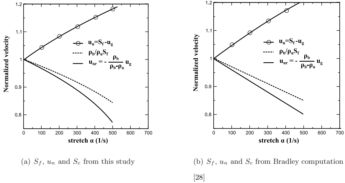
Figure IX.3: Comparison of S_f , u_n and S_c for a stoichiometric methane/air flame, P=0.1 MPa, T=300 K.
