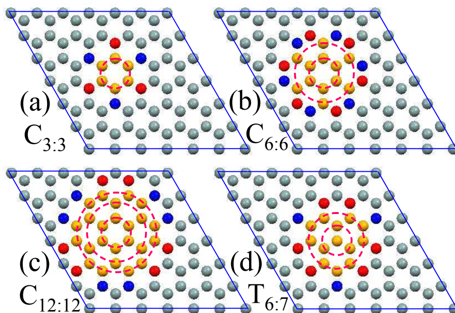
Fig. 6.1 : (a)-(c): Schematics of the calculated crystalline structures for balanced non-passivated circular shaped C_{3:3} , C_{6:6} and C_{12:12} GNM structures, respectively; (d) the same for unbalanced non-passivated triangular shaped T_{6:7} GNM structure. Edge carbon atoms are in blue and red color to represent A and B sites, respectively. For convenience, positions of removed atoms are indicated in orange.
