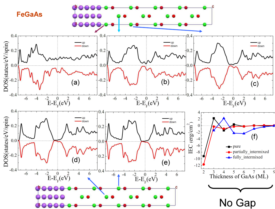
Fig. 2.18 : IEC for [\text{Fe}_5\text{GaAs}_x]_2 as a function of GaAs thickness and the density of states for different layers in GaAs barrier.
