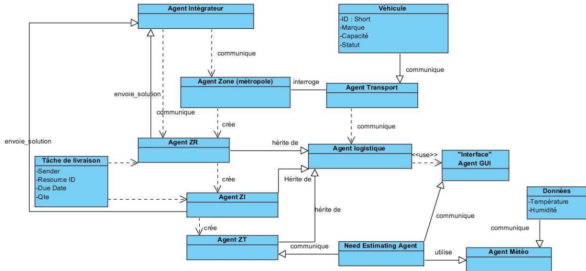
Figure III. 5 Architecture du système
