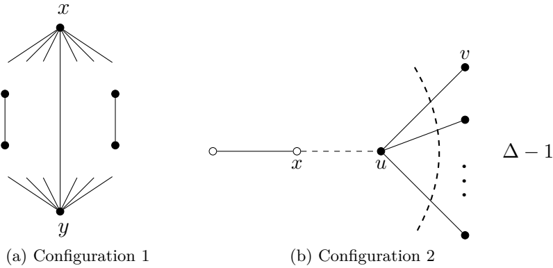
Figure 3.19: Forbidden configurations
