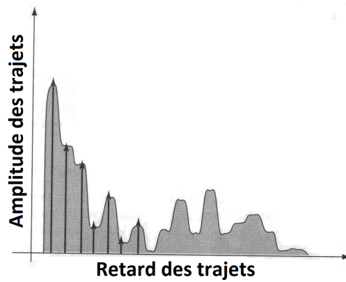
(c) P-rake
