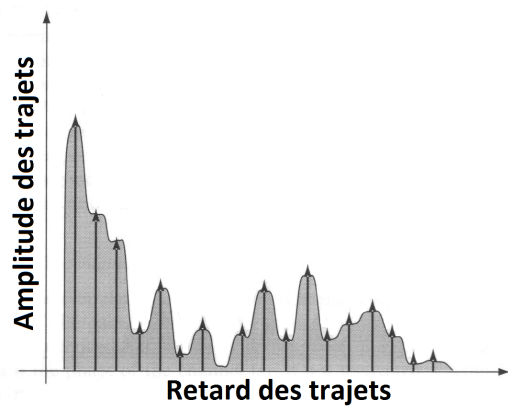
(a) A-rake
