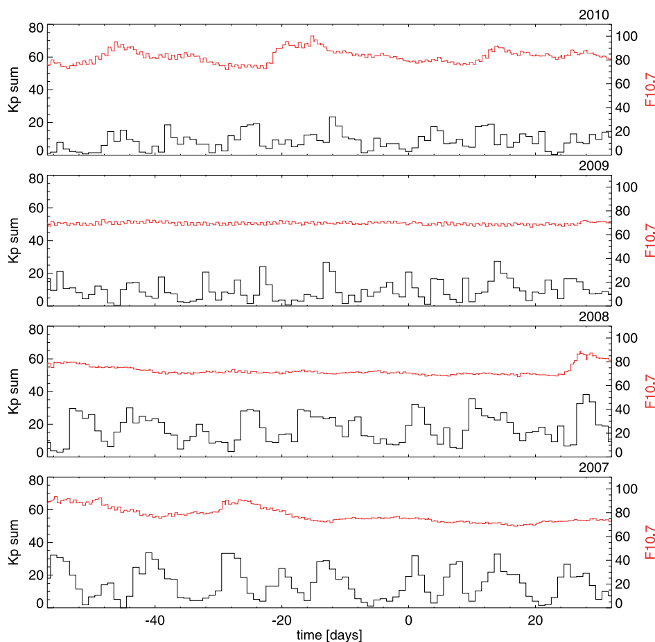
Figure 6. Representation of the sum of the Kp (black, left scale) and F_{10.7} (red, right scale) indices recorded during 4 years around the time of the M_w 8.8 Chile earthquake. Each panel is related to 1 year and represents the indices for each day from 1 January to 31 March. The day 0 on the x axis corresponds to 27 February each year (the day of the main shock in 2010). Kp data are from the Kyoto World Data Center, and F_{10.7} data are from the National Geophysical Data Center (NGDC) of the National Oceanic and Atmospheric Administration (NOAA).
