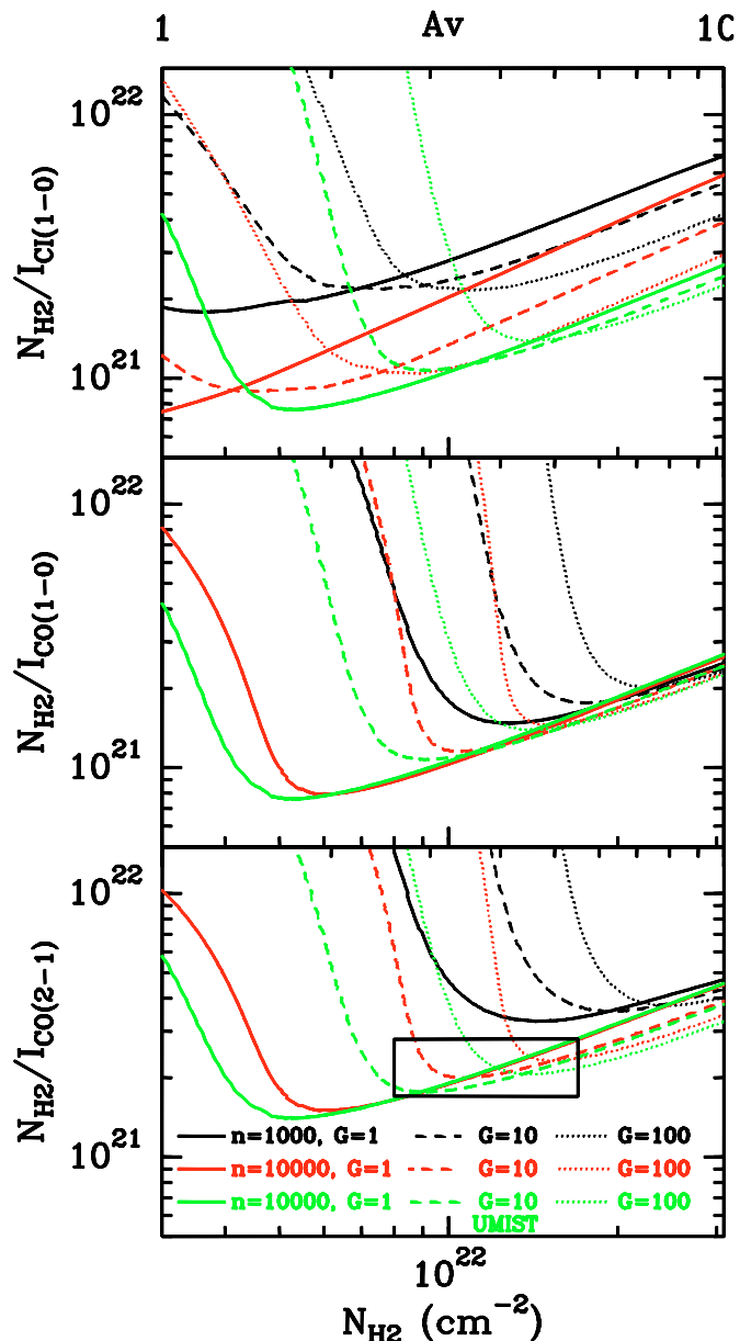
Fig. 9. Model N(\text{H}_2)/I_{\text{C}_1} (top) and N(\text{H}_2)/I_{\text{CO}} factors as a function of visual extinction A_v and H column density into the cloud. As the atomic Hydrogen skin is very thin even for the highest UV field used here, the clouds are essentially completely molecular so the depth is shown as \text{H}_2 depth not H. The x-axis extends beyond standard cloud column densities in order to show how a change in cloud structure with respect to Galactic clouds would affect the CO intensities. The expected range is roughly indicated by a box in the lower panel. While the UV field has little effect on the hydrogen, it has a major effect on the C + /C/CO transition.
