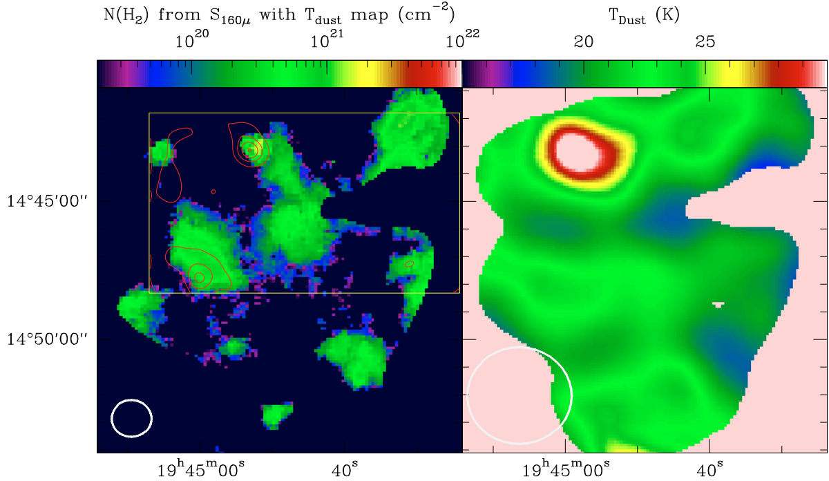
Fig. 8. H_2 column density map estimated from 160\ \mu\text{m} emission using the dust temperature map shown on the right ( left ), CO(2-1) intensity contours every (0.15\ \text{K km s}^{-1}) starting from (0.15\ \text{K km s}^{-1}) . Temperature map from 160\ \mu\text{m} Spitzer and 100\ \mu\text{m} IRAS data ( right ). The yellow rectangle is the region we have mapped in CO(2-1) with HERA. The beams for the NH_2 , CO and temperature are plotted in white.
