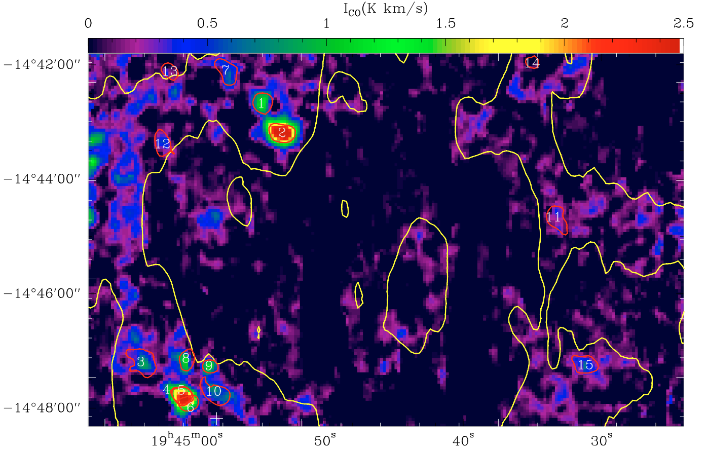
Fig. 6. CO(2–1) intensity map obtained using the masking method described in Sect. 6.1. The map unit is \text{K km s}^{-1} , the yellow H \alpha contour is at N(\text{H I}) = 10^{21} \text{ cm}^{-2} , the red contours are the half maximum levels of each cloud identified by eye, the numbers correspond to the ones in Table 2. The cross corresponds to (0, 0) offsets of the HERA CO(2–1) map.
