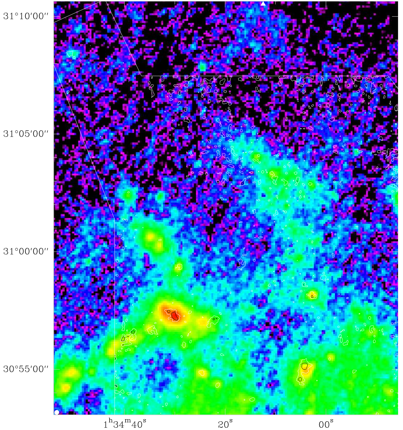
Fig. A.10. Northern part of Spitzer 70\ \mu\text{m} image with I_{\text{CO}} main beam contours of 1 (white), 2, 4 (black), 8 (blue) \text{K km s}^{-1} . The beam size is shown as a white dot in the lower left corner.
