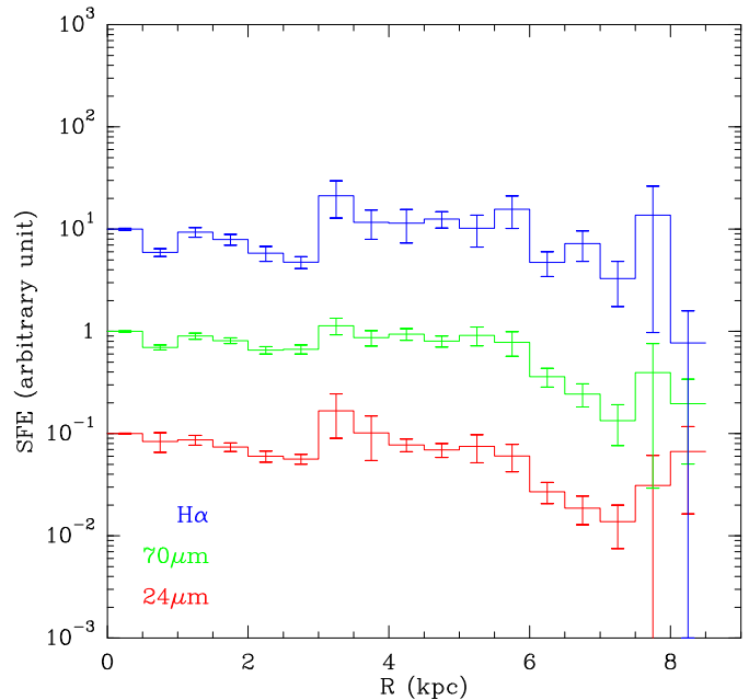
Fig. 9. Radial distribution of the SFE in arbitrary units, all of the curves are normalized to the central value and shifted by 1 decade along the vertical axis.
