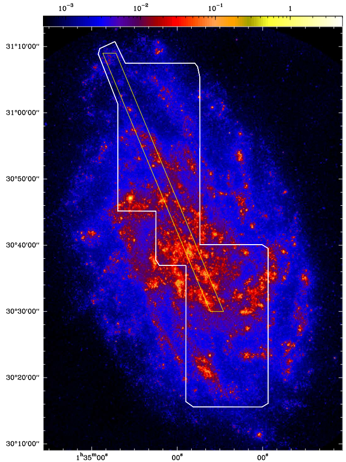
Fig. 1. The Local Group galaxy M33. This color image shows the GALEX FUV data that trace young stars and dust in the disk through attenuation. Overlaid are the observed fields (a) using the IRAM 30m Pico Veleta telescope in the CO(2–1) line (thick white outline) and (b) by HIFI/PACS instruments as part of the HERM33ES Herschel Key Program (thin yellow stripe).
