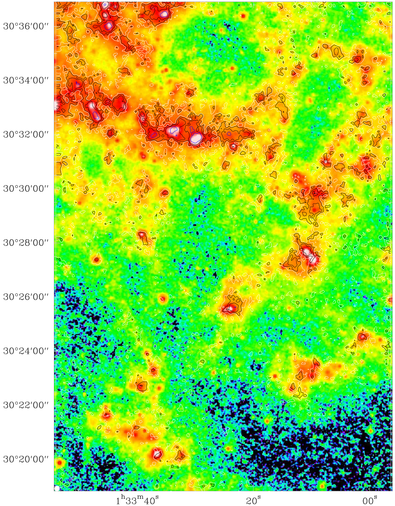
Fig. A.9. Southern part of Spitzer 24 \mu\text{m} image with I_{\text{CO}} main beam contours of 1 (white), 2, 4 (black), 8 (blue) \text{K km s}^{-1} . The beam size is shown as a white dot in the lower left corner.
