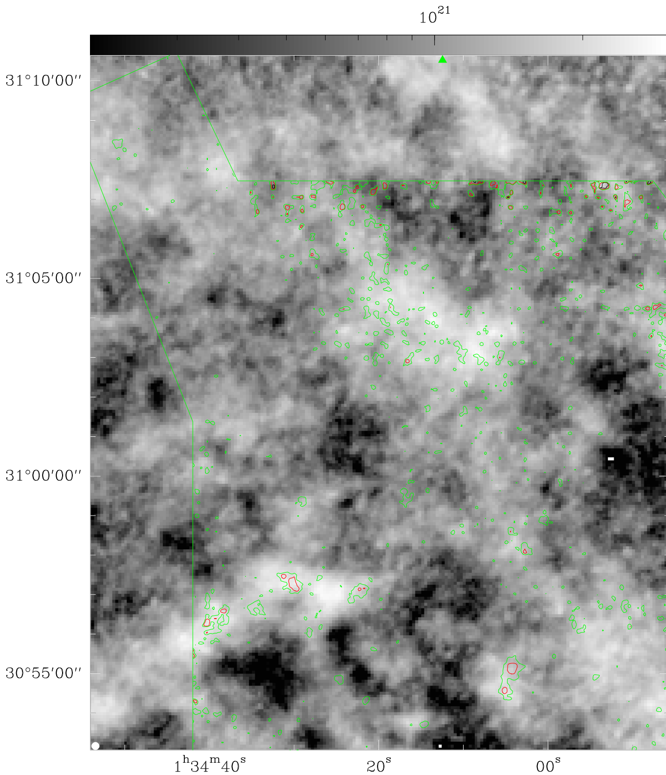
Fig. A.13. Northern part of VLA H I 21 cm integrated intensity image with I_{CO} main beam contours of 1 (green), 2 (red), 4 (black), 8 (blue) K km s -1 . The beam size is shown as a white dot in the lower left corner.
