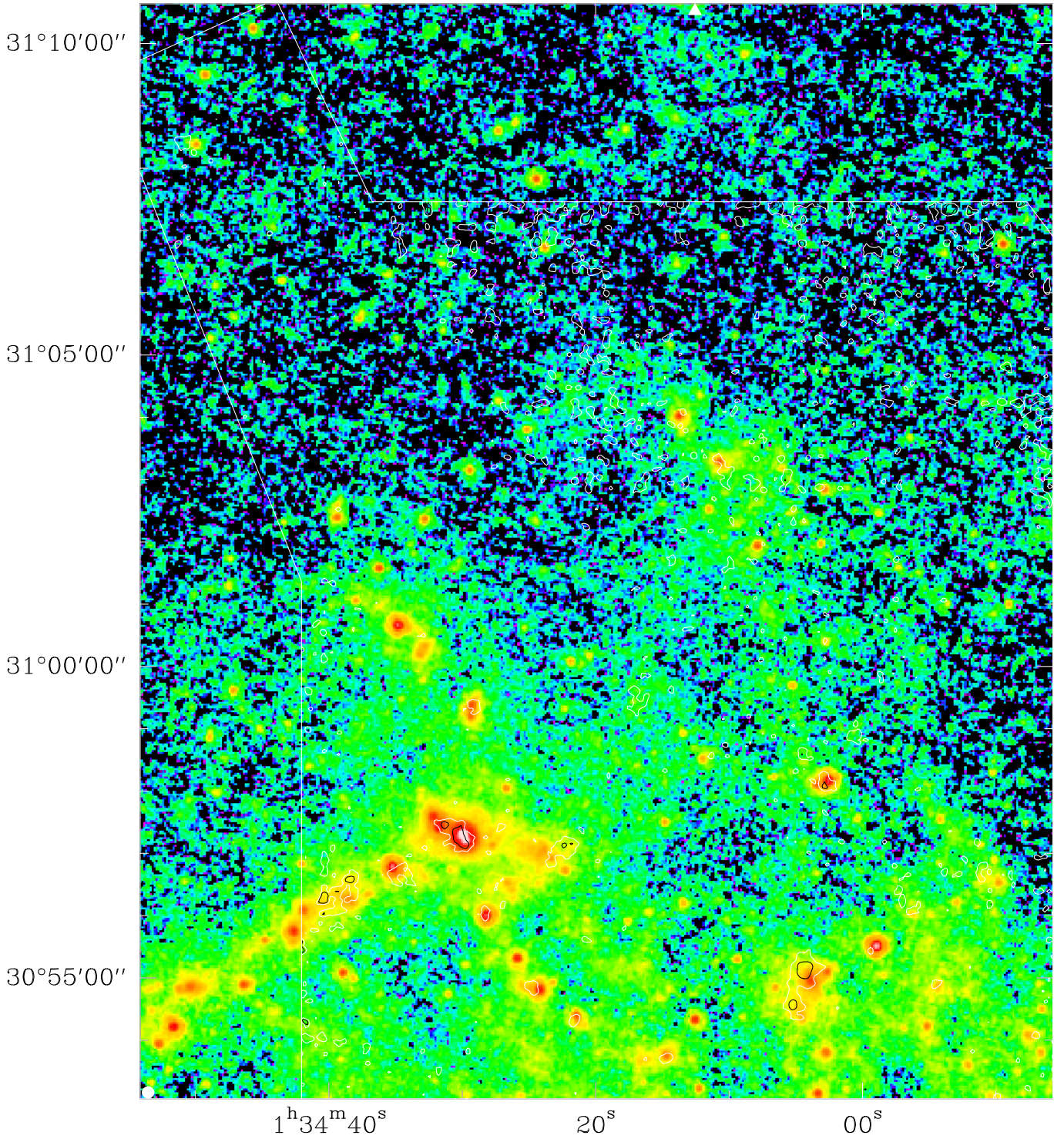
Fig. A.7. Northern part of Spitzer 24 \mu m image with I_{CO} main beam contours of 1 (white), 2, 4 (black), 8 (blue) K km s^{-1} . The beam size is shown as a white dot in the lower left corner.
