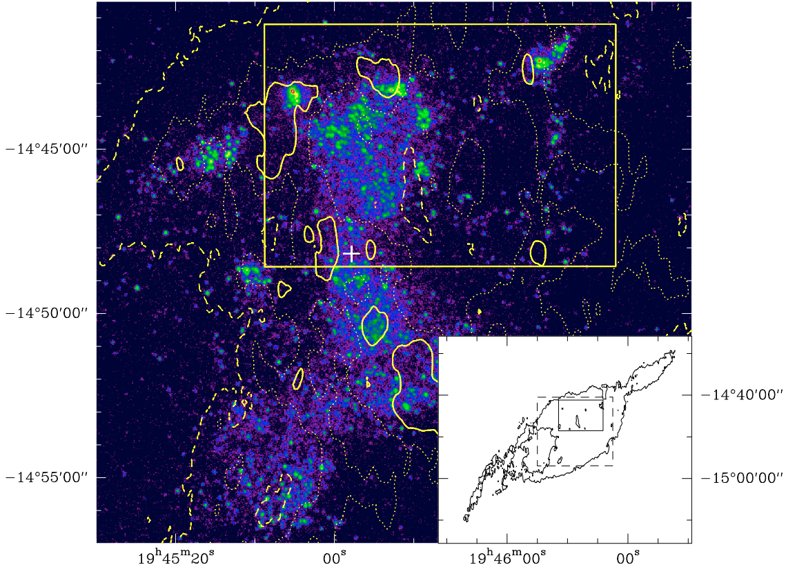
Fig. 1. Main image GALEX FUV filter image of NGC 6822. The yellow box indicates the area observed in CO. The dashed, dotted, and solid yellow contours indicate the H I column density at 12'' \times 42'' resolution from de Blok & Walter (2006b) at column densities of 0.5, 1, and 1.5 \times 10^{21} \text{ cm}^{-2} respectively. The white cross corresponds to (0, 0) offsets of the HERA CO(2–1) map. Bottom right HI contour at a column density of 0.5 \times 10^{21} \text{ cm}^{-2} . The dashed rectangle corresponds to the GALEX FUV map above, the solid line contour to the area observed in CO.
