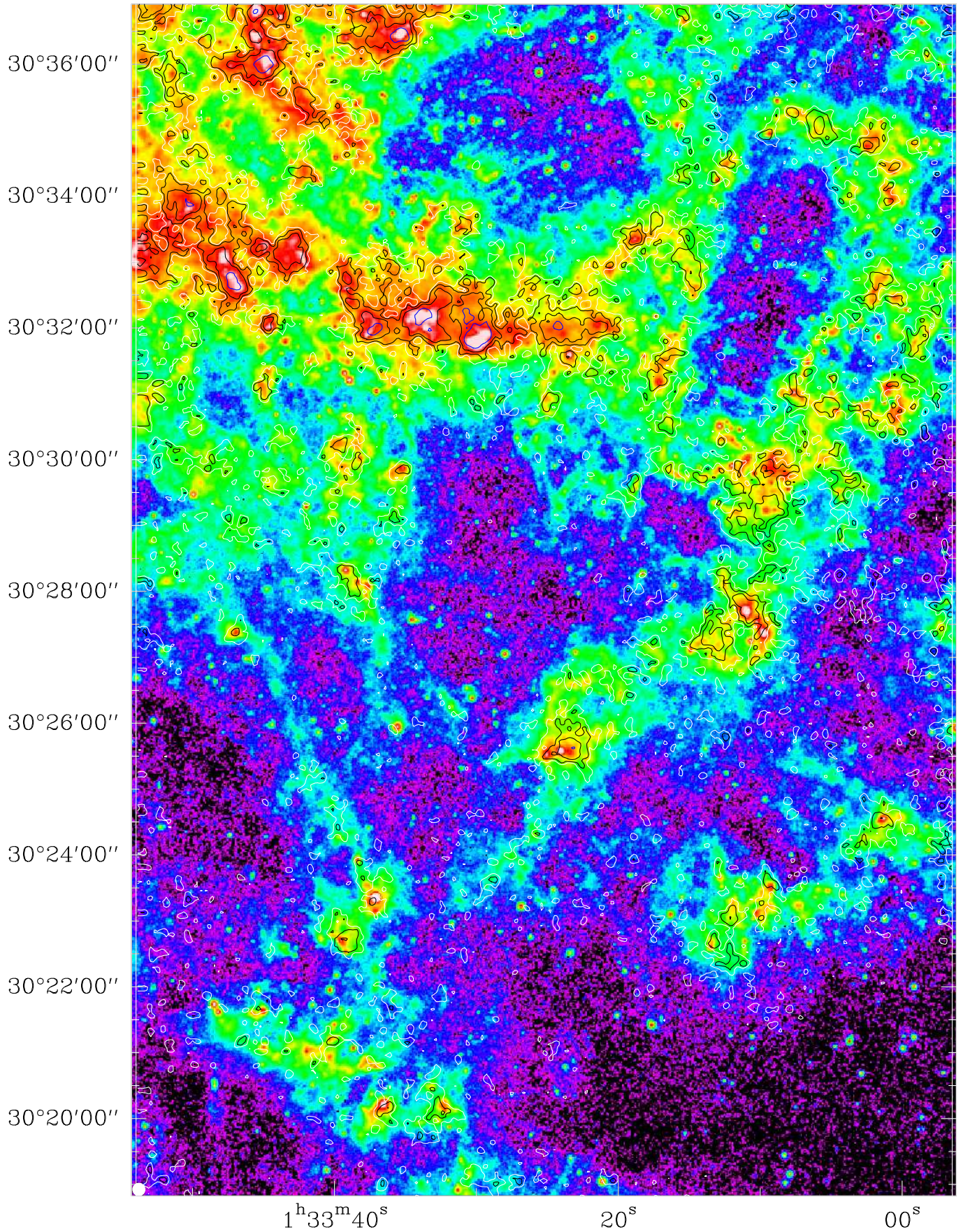
Fig. A.6. Southern part of Spitzer 8\ \mu\text{m} image with \text{I}_{\text{CO}} main beam contours of 1 (white), 2, 4 (black), 8 (blue) \text{K km s}^{-1} . The beam size is shown as a white dot in the lower left corner.
