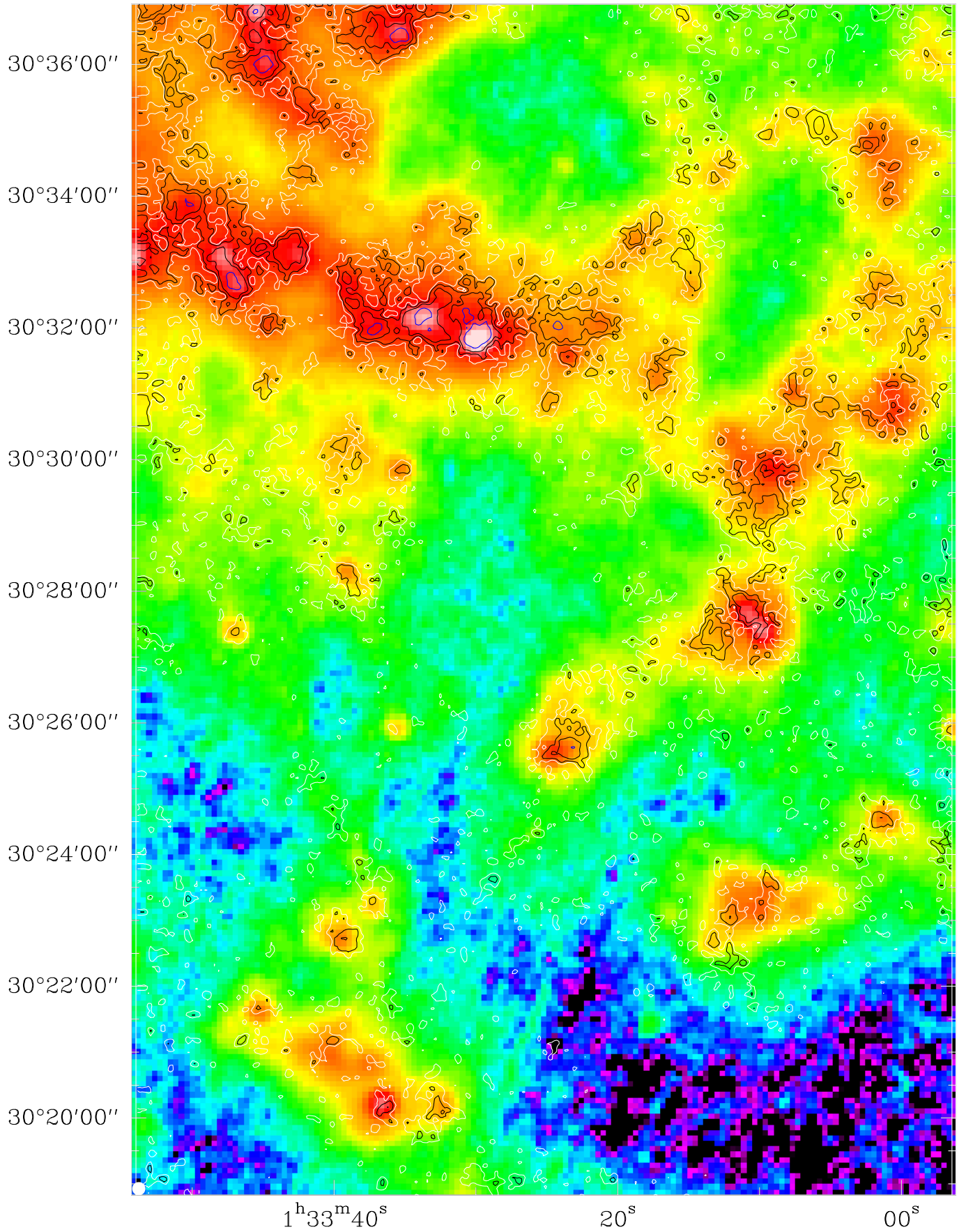
Fig. A.12. Southern part of Spitzer 70\ \mu\text{m} image with \text{I}_{\text{CO}} main beam contours of 1 (white), 2, 4 (black), 8 (blue) \text{K km s}^{-1} . The beam size is shown as a white dot in the lower left corner.
