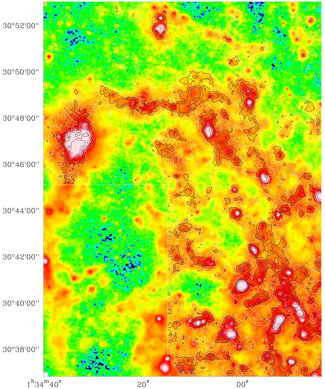
Fig. A.8. Center part of Spitzer 24 \mu\text{m} image with I_{CO} main beam contours of 1 (white), 2, 4 (black), 8 (blue) \text{K km s}^{-1} . The beam size is shown as a white dot in the lower left corner.
