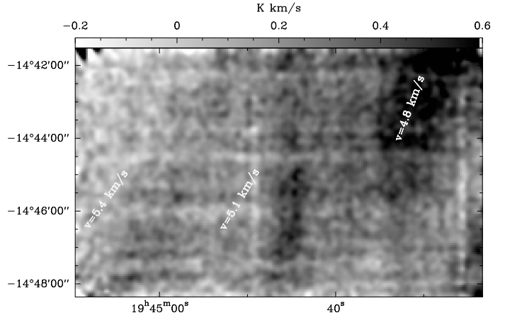
Fig. 13. \text{CO}(2-1) emission from the local molecular “cirrus” cloud along the line of sight to NGC 6822. Indicated on the figure are the velocities of the emission at 3 different positions.
