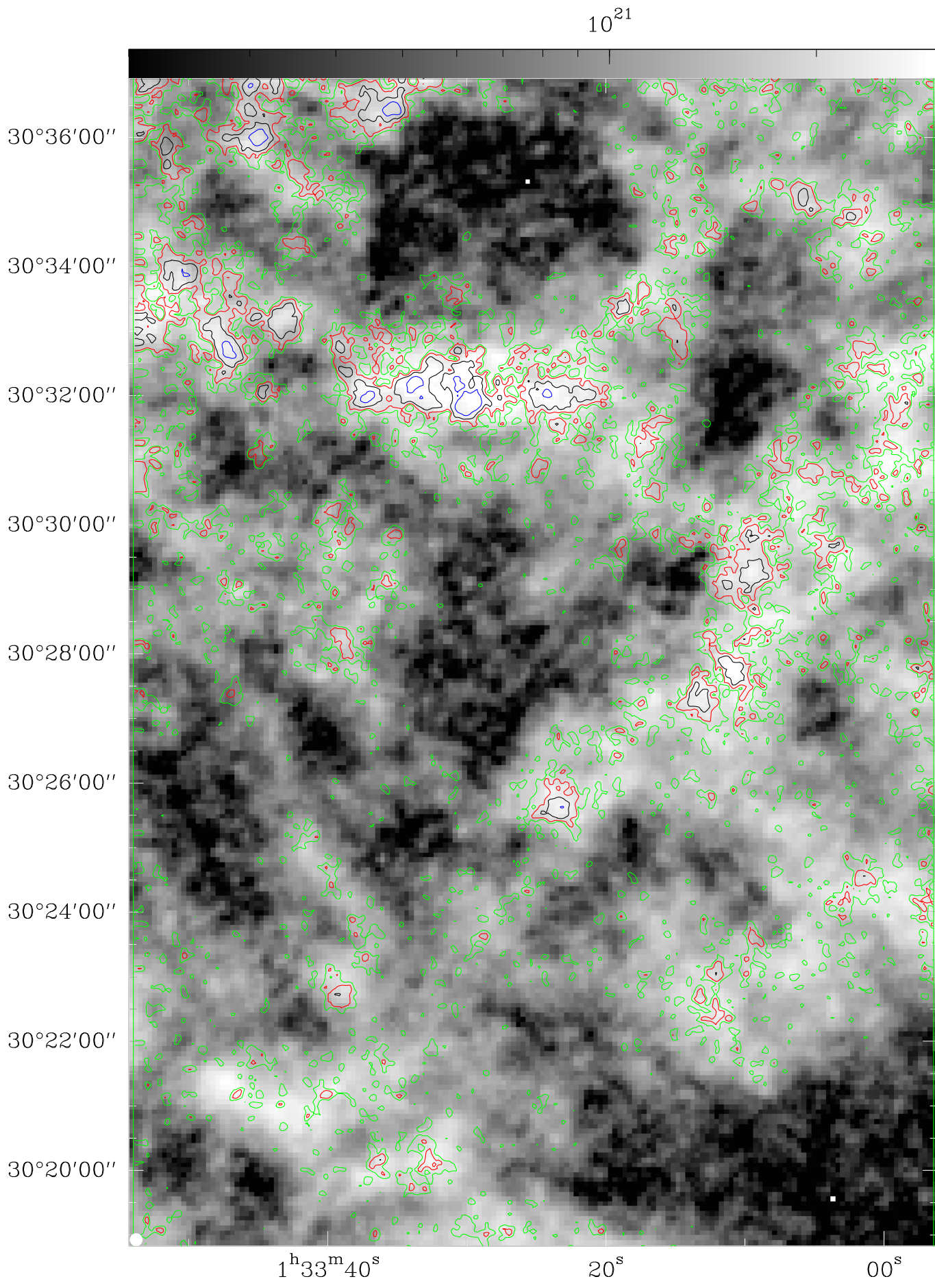
Fig. A.15. Southern part of VLA H I 21 cm integrated intensity image with I_{\text{CO}} main beam contours of 1 (green), 2 (red), 4 (black), 8 (blue) \text{K km s}^{-1} . The beam size is shown as a white dot in the lower left corner.
