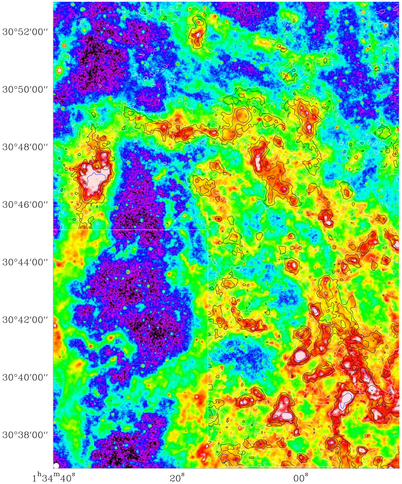
Fig. A.5. Center part of Spitzer 8 \mu\text{m} image with I_{CO} main beam contours of 1 (white), 2, 4 (black), 8 (blue) \text{K km s}^{-1} . The beam size is shown as a white dot in the lower left corner.
