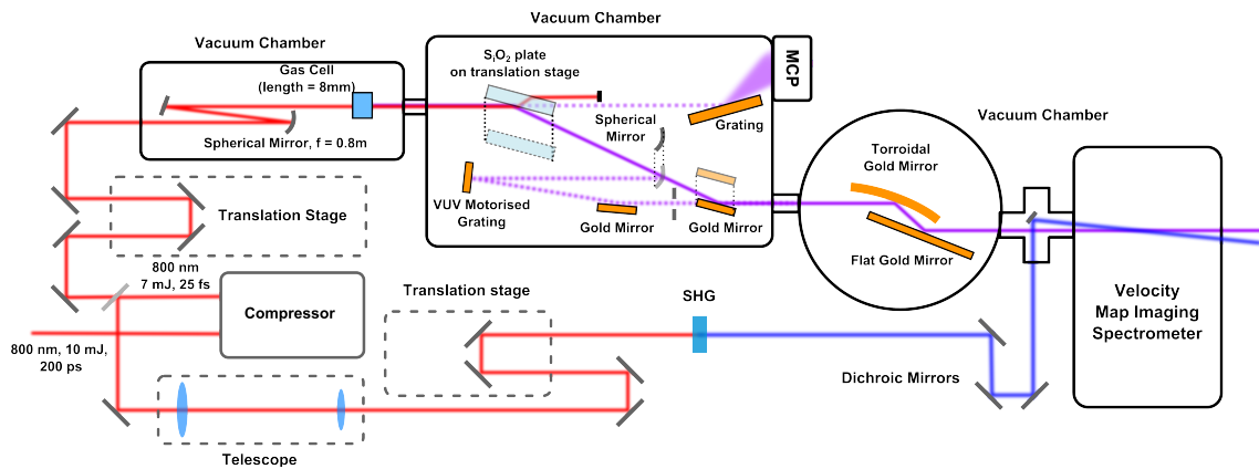
Figure 5.22.: Fs-VUV pump probe setup.
