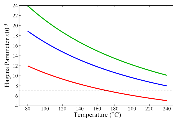
Figure 4.7.: Hagena parameter as a function of temperature for carbon dioxide at a backing pressure of 10 bar (red), 20 bar (green) and krypton at a backing pressure of 20 bar (blue).
