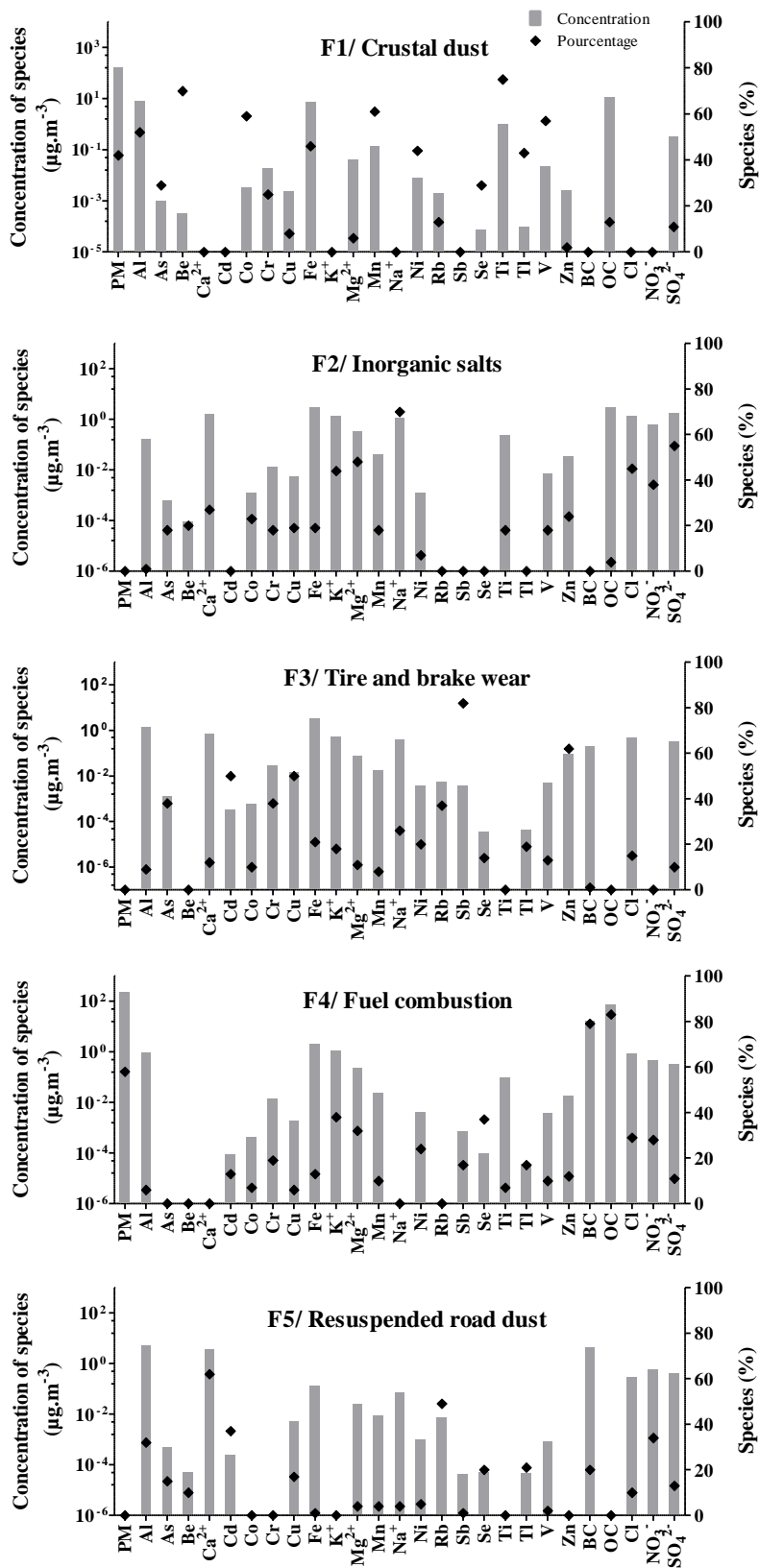
Figure 6: PM source profiles resolved from PMF ( \mu\text{g.m}^{-3} ) and species contributions (in %) for each source in Bamako.
