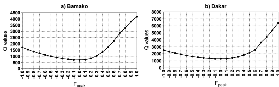
Figure 5: Plot of Q as a function of F_{\text{peak}} for the PM data set from Bamako (a) and Dakar (b).
