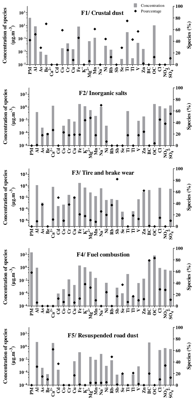
Figure 6: PM source profiles resolved from PMF (µg.m -3 ) and species contributions (in %) for each source in Bamako.
