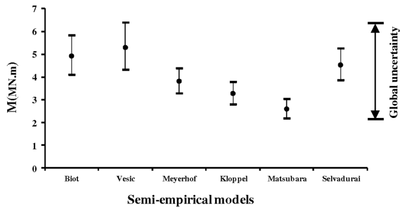
Figure 3-40: Global uncertainties for the a) Subgrade reaction modulus k_s , b) Maximum differential settlement \Delta and c) Maximum bending moment M by considering 95% confidence bound for each semi-empirical model with log-normal distribution ( E_s=2 MPa, E_c=20 GPa, \nu_s=0.3 , d=1.5 m, e=0.15 m, L=30 m, q=100 kN/m, CV_{E_s}=15\% , CV_L=10\% , CV_d=CV_{\nu_s}=CV_{E_c}=5\% ).
