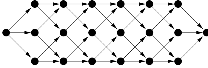
Figure 3.3: The "boloney" graph D_6
