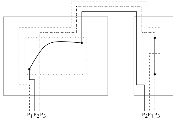
Figure 4.3: Illustration of the swaps made within two consecutive zones in the proof of Lemma 85.
