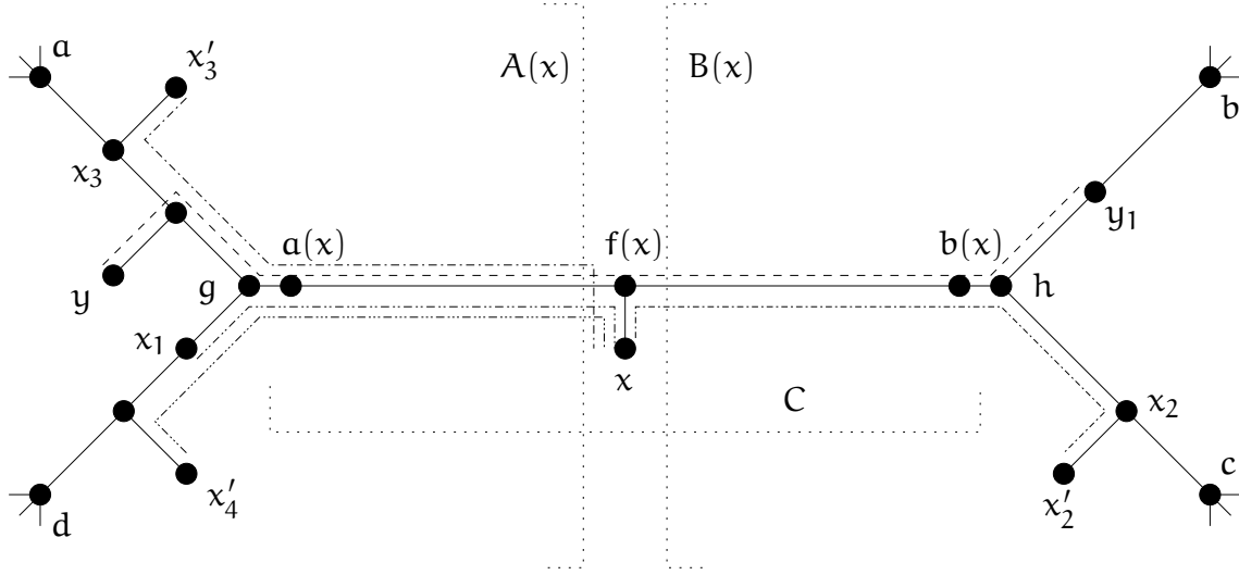
Figure 2.1: The nodes a, b, c, d are I_1 -nodes and g, h are I_3 nodes. C is a caterpillar, and x is an L_2 -leaf of C , with requests xx_1, xx_2', xx_3' and xx_4' . The closest quasi-R-neighbours of x are x_1, x_2 and x_3 . The leaf x has two wingspans: the path between x_1 and x_2 , and the path between x_3 and x_2 . Either of these wingspans contains the whole backbone of C , so x covers C . Similarly, yy_1 is a request, so the L_2 -leaf y , which does not belong to the caterpillar C , covers C as well.
