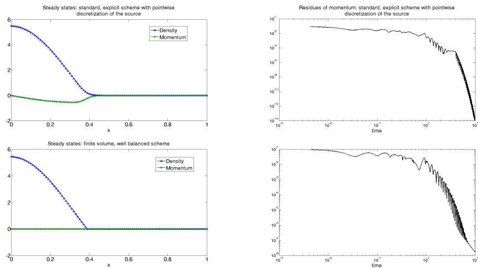
Figure 7.8: On the left: Density and momentum profiles at steady state for system (7.1.1) in the case P(\rho) = \varepsilon\rho^2 and \varepsilon = D = a = b = L = 1 , \chi = 50 obtained by: (at the top) a finite difference scheme based on the relaxation technique with centered in space approximation of the source (6.2.8); (at the bottom) a finite volume method with Suliciu relaxation solver and well-balancing (6.3.11). On the right: corresponding residues of the momentum.
