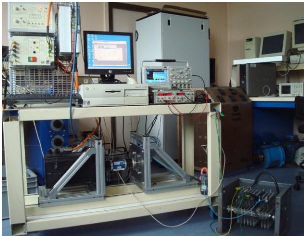
Fig. 4.9. The test bench for the small AFIPM machine in generator mode with resistive load.
