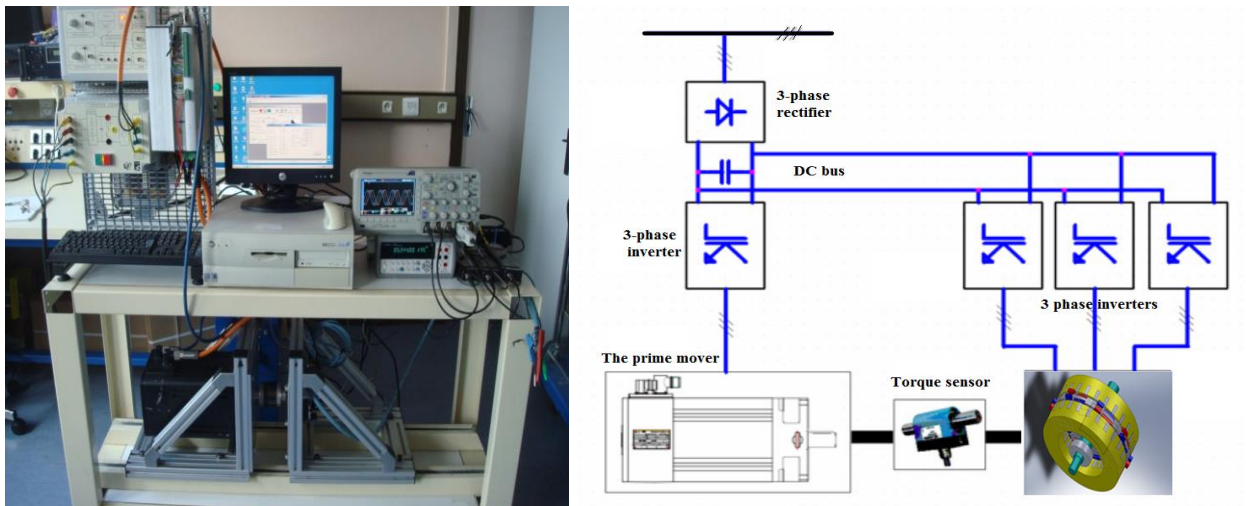
Fig. 4.1. Experimental set-up.
