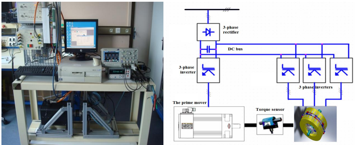
Fig. 4.1. Experimental set-up.
