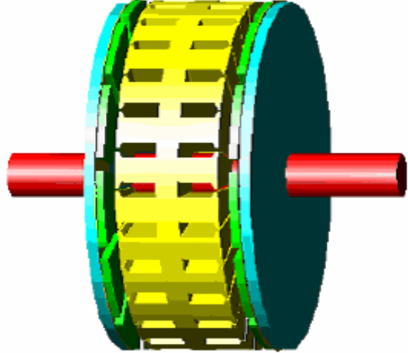
Fig. 1.2. Small single-stator-double-rotor AFPM machine topology. (after [2])
