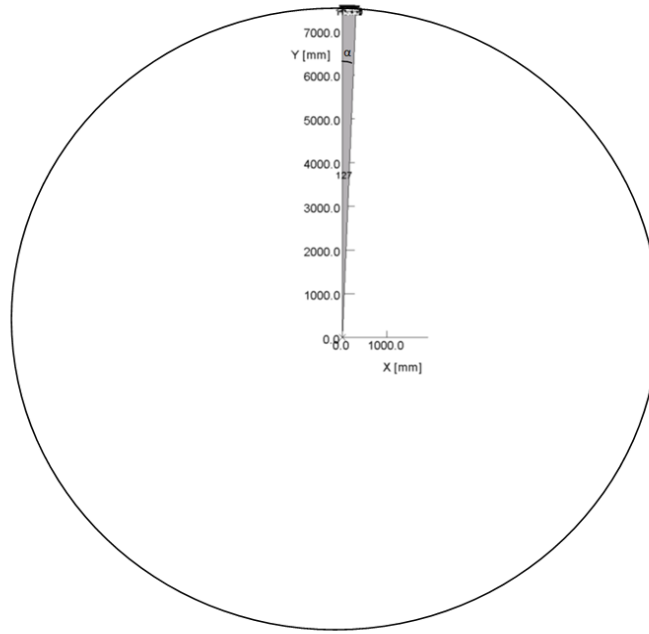
Fig. 3.31. AFIPM machine symmetry considered for 2D FE simulations.
