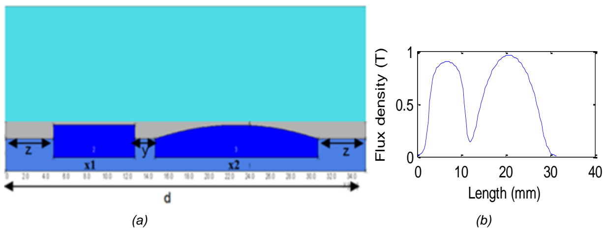
Fig. 3.36. (a) One-pole representation of the AFIPM machine topology; (b) flux density distribution for a half-period.
