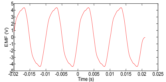
Fig. 10. Analytically-computed open-circuit (no-load) back-emf signal.
