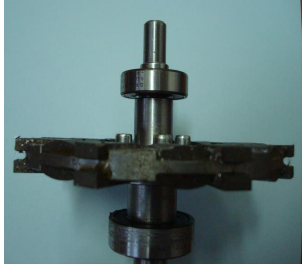
Fig. 1.7. Photograph of the PM-rotor assembly, the rotor shaft and the two bearings of different size.
