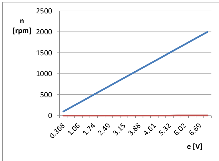
Fig. 4.8. Rotor speed vs. back-emf.
