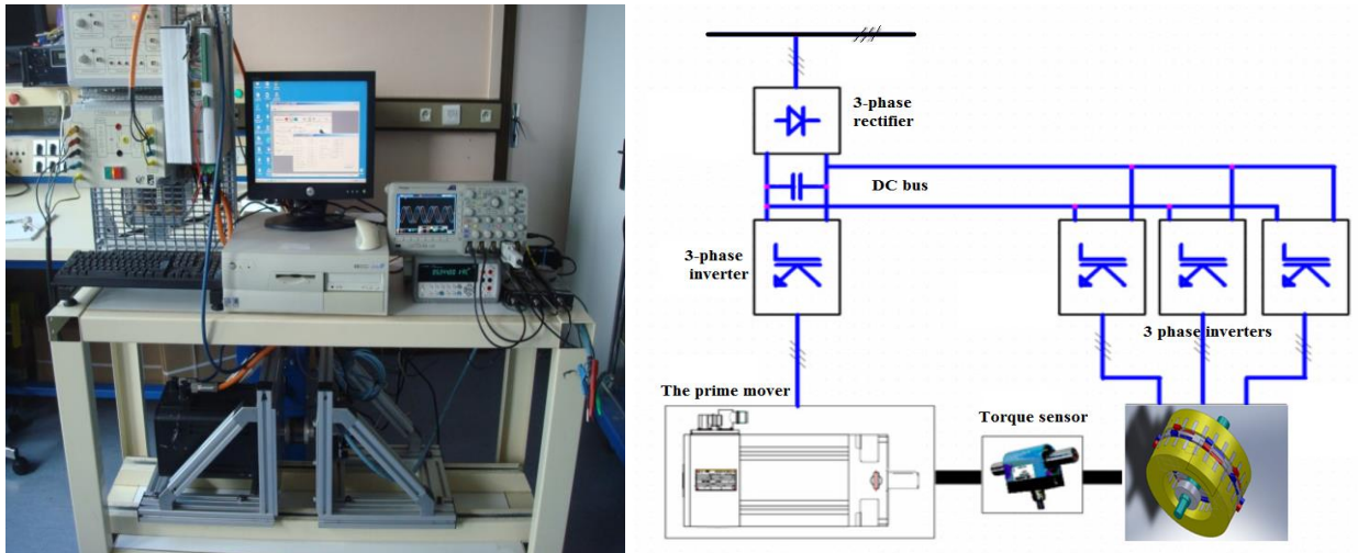
Fig. 4.1. Experimental set-up.
