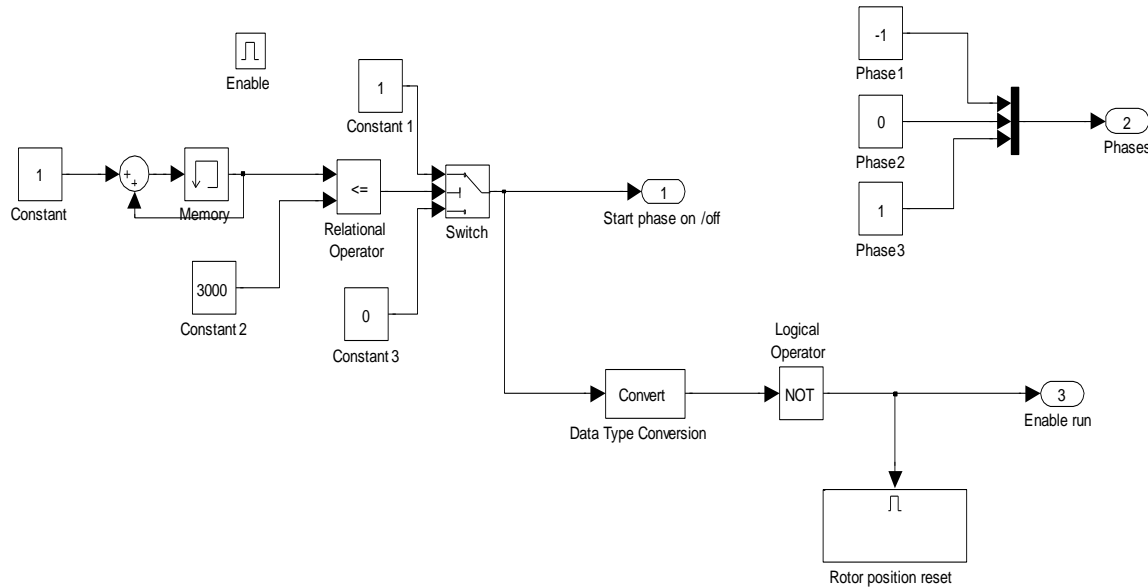
Fig. 4.16. "Start" sub-program
