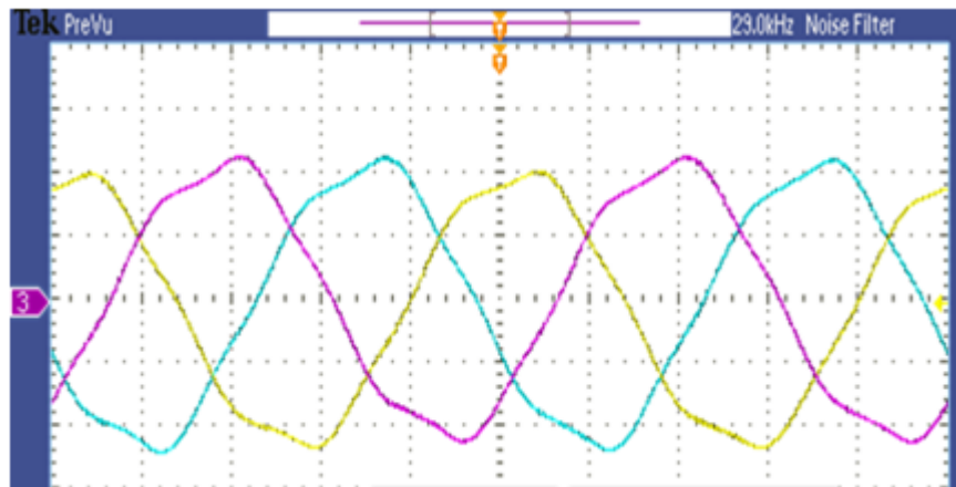
Fig. 4.2. Experimental open-circuit (no-load) back-emf waveforms of the three armature-phases.
