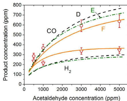
Figure 7. Hydrogen and carbon oxide concentration produced per current pulse in the discharge volume of the UV510 reactor. Lines correspond to model predictions, see text.
