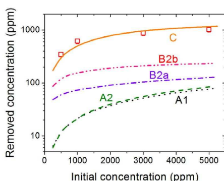
Figure 4. Acetaldehyde concentration removed per current pulse in the discharge volume of the UV510 reactor. Lines correspond to model predictions for different simplified kinetic schemes described in the text.
