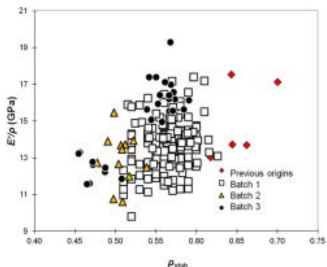
Fig.4.7. Relationship between specific modulus ( E'/\rho ) and \rho_{stab} (stabilized specific gravity measured after 3 weeks at 20^{\circ}\text{C} \pm 2 and 65\% \text{ HR} \pm 5 ) for all the specimens ( N^{\circ} : 207).
