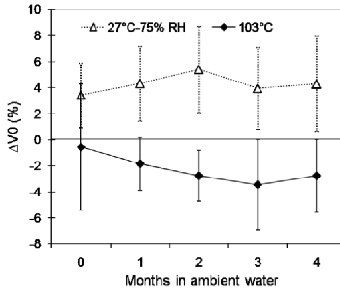
Fig.5.9 Changes in oven- dried volume ( \Delta V_0 %) for long- time water treatment specimens, after prefect drying ( 103^\circ\text{C} ) and one month in 27^\circ\text{C} and 75% RH. N°:12 each \times 5=60 total.
