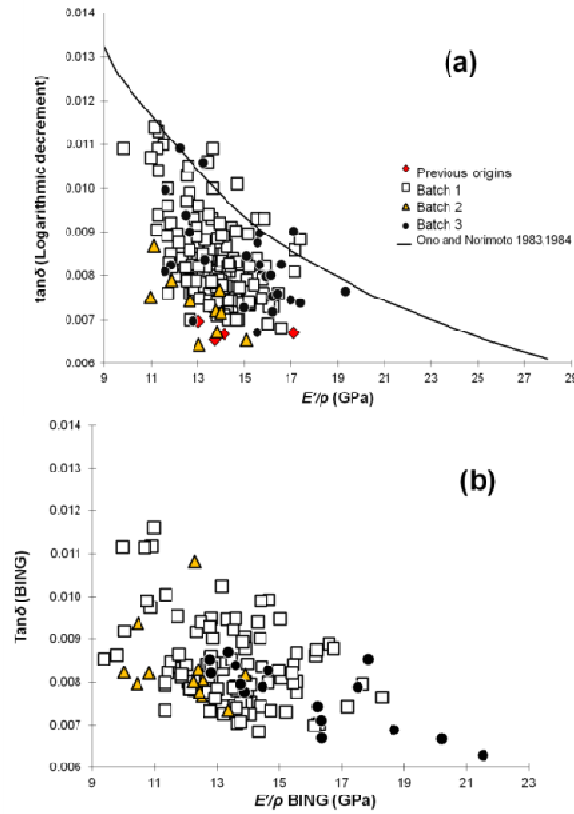
Fig.4.3. relationship between \tan\delta by logarithmic decrement (a) and \tan\delta by BING (b) method and their corresponding E'/\rho , note that BING test was not done for all the specimens and thus, the number of specimens is lower ( N^\circ : 143).
