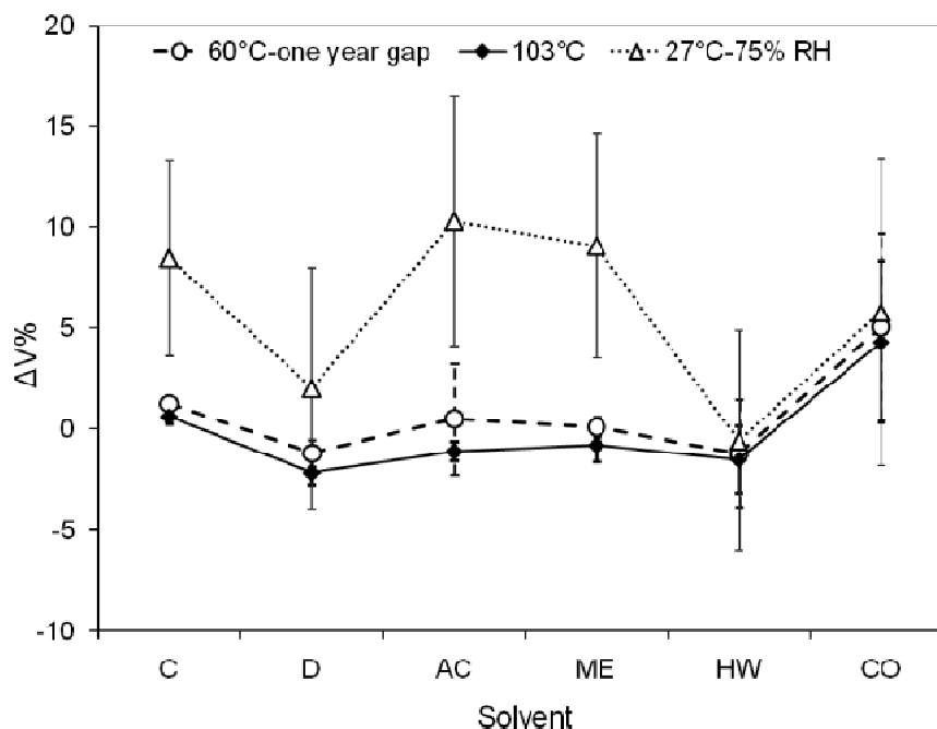
Fig.6.20. Variations in volume ( \Delta V\% ) for shrinkage specimens after second time of quasi anhydrous drying with one year gap, complete drying ( 103^\circ\text{C} ), and one month in 27^\circ\text{C} and 75% RH. C: Controls/no-chemical treatment, D: Dichloromethane, AC: Aceton, ME: Methanol, HW: Hot water, CO: Complete extraction/specimens submitted to successive extraction after last treatment (HW). N^\circ : 18 in each group of treatment.
