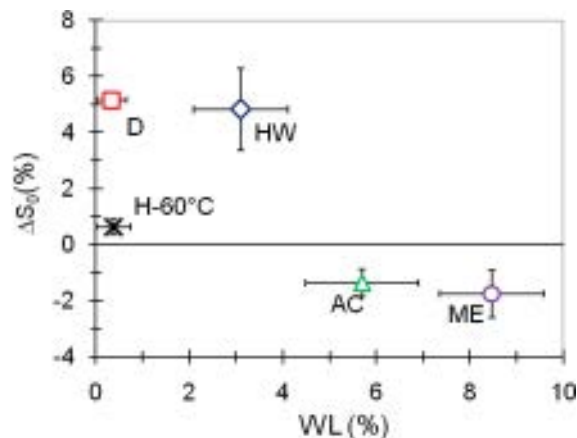
Fig.6.11. Variations in oven dry \Delta S_0 (%) – based on 103°C drying- and weight loss (WL%) for shrinkage specimens submitted to independent extractions. value for H is that of 60°C drying.
