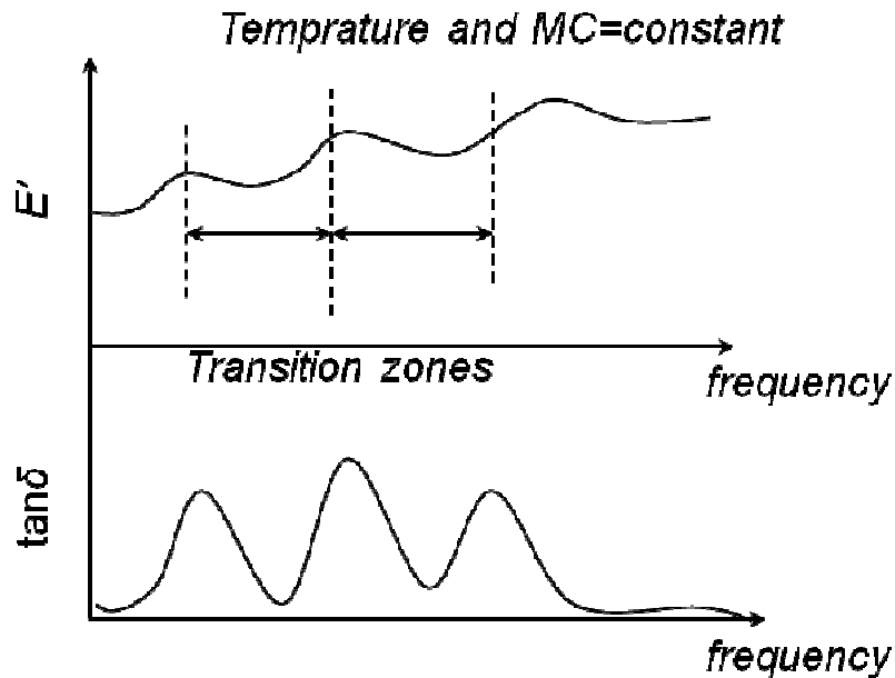
Fig.2.9. Illustration transition zones for modulus and \tan\delta in a constant moisture content (MC) and temperature conditions.
