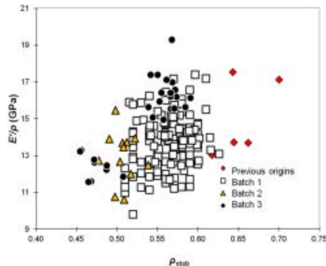
Fig.4.7. Relationship between specific modulus ( E'/\rho ) and \rho_{stab} (stabilized specific gravity measured after 3 weeks at 20^\circ\text{C} \pm 2 and 65\% \text{ HR} \pm 5 ) for all the specimens ( N^\circ : 207).
