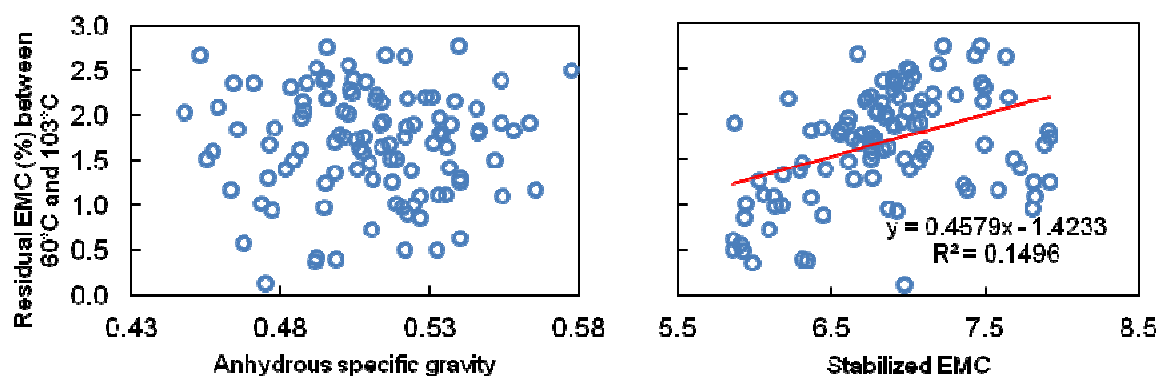
Fig. 3.6: Residual MC (%) (Between MC after 48 hrs in 60°C and MC obtained after 48hrs in 103°C) against anhydrous specific gravity and stabilized EMC (air dried %).
