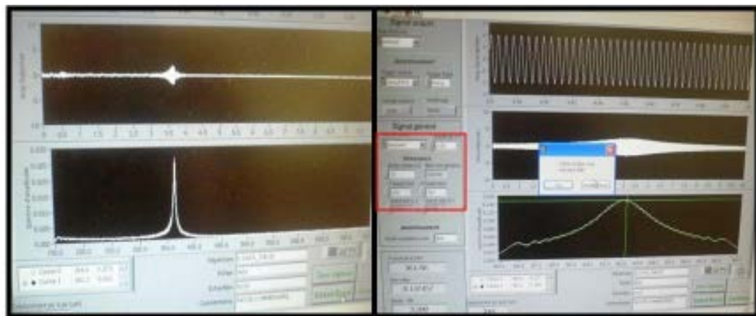
Fig.3.12. the visualization of detected resonance frequency which would result in calculating Q^{-1} based on bandwidth of half power. In second photo the red window shows the place for changing the setting of parameters.
