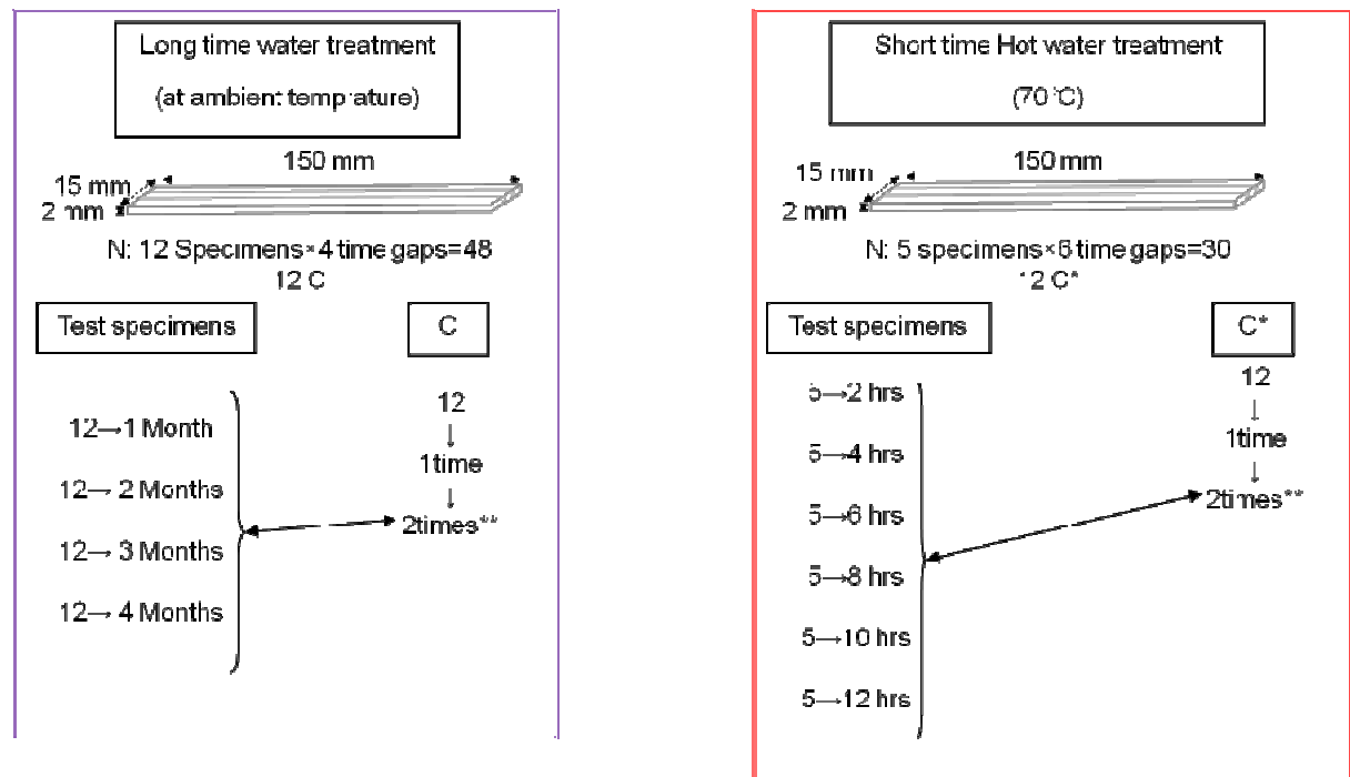
Fig.5.1. General protocol for hygro- thermal treatments
