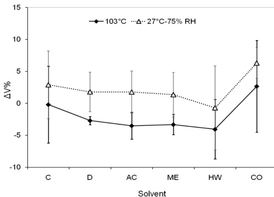
Fig. 6.21. Variations in volume ( \Delta V\% ) for vibrational specimens after 103^\circ\text{C} drying, and one month in 27^\circ\text{C} and 75% RH. N°:12 for each treatment, except for HW : 5 specimens for this treatment.
