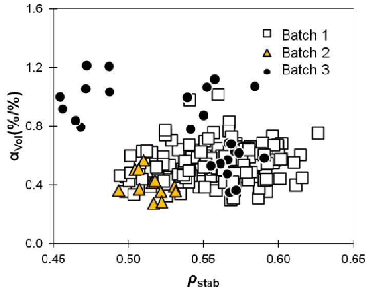
Fig.4.12. Volumetric swelling coefficient ( \alpha_{vol} = S_{vol}/MC \text{ \%/\%} ) and \rho_{stab} relationship for three batches.
