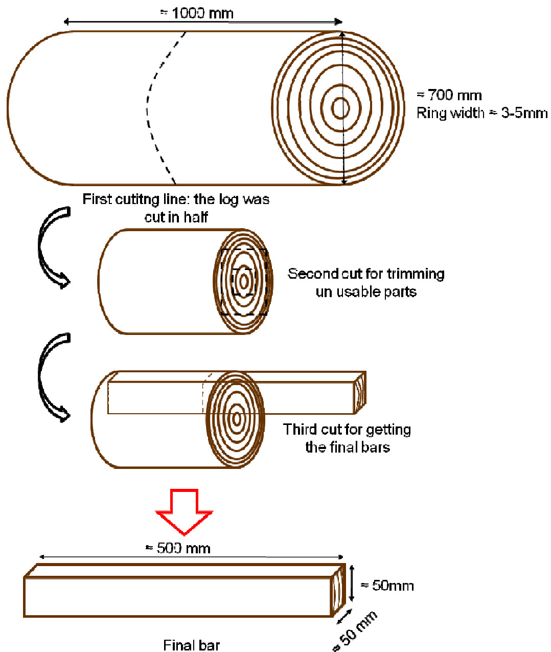
Fig.3.1. Schematic of cutting wood bars from original log in Iran
