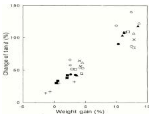
Fig. 2.10. Changes in \tan\delta_L in Sitka spruce in function of impregnation of simple phenolic. The crosses are indicators of specimens treated with Resorcinol (from Sakai et al. 1999).
