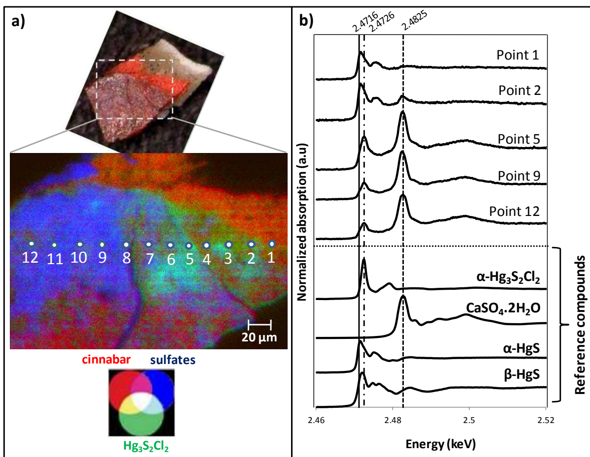
Figure 2.4.: a) RGB composite of three S\text{-}K_{\alpha} intensity maps representing sulfur acquired at 2.4716 keV (cinnabar, red), 2.4726 keV ( \text{Hg}_3\text{S}_2\text{Cl}_2 compounds, green) and 2.4825 keV (sulfates, blue), corresponding to the dashed rectangle in the visible image of sample Ru-A; b) \mu\text{-XANES} spectra of some of the twelve points in the map in a) compared to spectra of reference compounds (metacinnabar, cinnabar, gypsum, corderoite).
