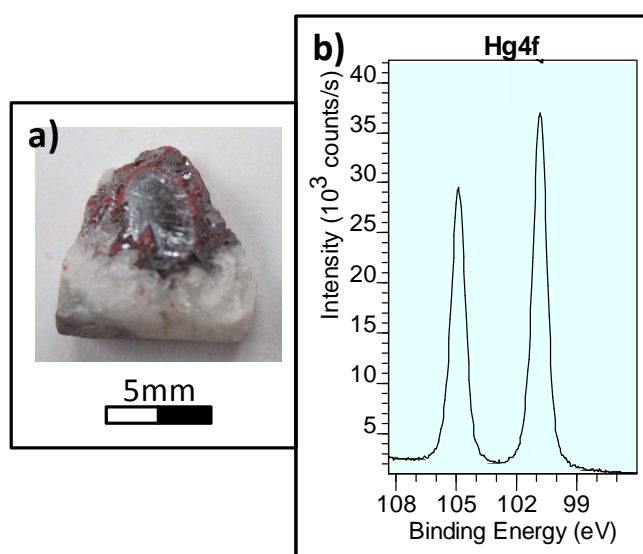
Figure 4.2.: a) Photograph of a darkened cinnabar ore from China analyzed by XPS; b) XPS spectrum obtained at the \text{Hg}_{4f} binding energy.
