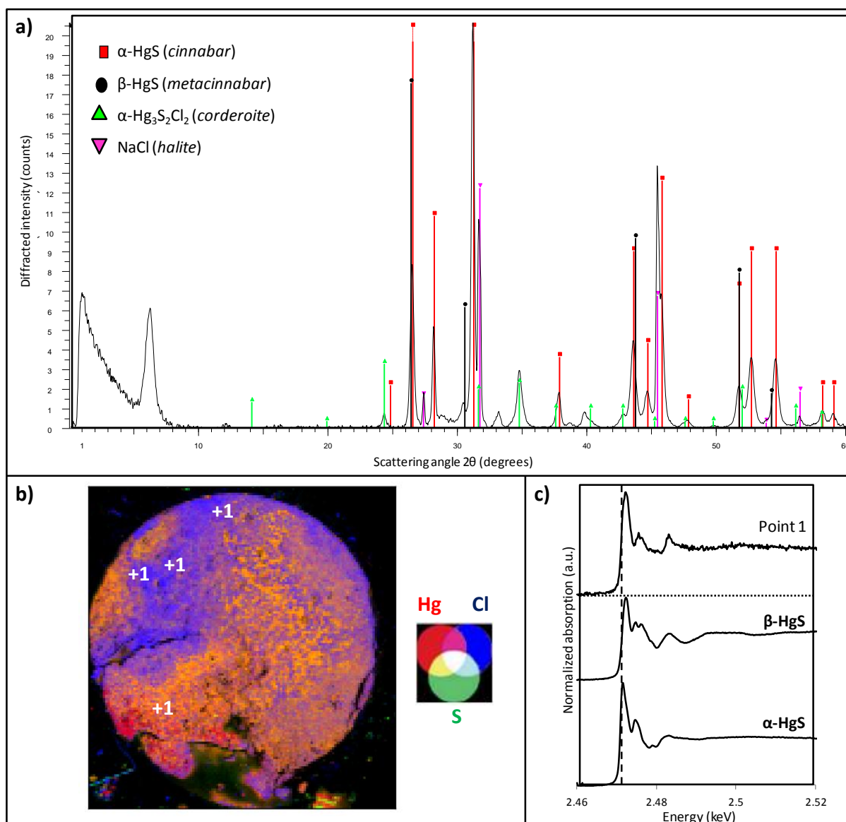
Figure 3.25.: Results of analyses obtained from sample P-NaCl/vermilion-light-NaOCl-closed: a) Diffraction pattern obtained in reflection mode compared to reference files ( \alpha -HgS in red, \beta -HgS in black, \alpha -Hg 3 S 2 Cl 2 in green and NaCl in pink); b) RGB composite of three \mu -XRF maps acquired at 2.9 keV showing the distribution of mercury (red), sulfur (green) and chlorine (blue); c) S K-edge XANES spectrum from position 1 shown in (b), compared to reference spectra of \alpha -HgS and \beta -HgS.
