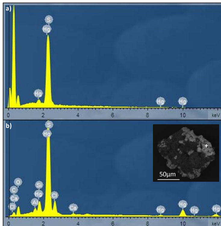
Figure 1.10.: SEM-EDX analyses of few microns resolution showing spectra of (a) vermilion ( \alpha -HgS, Prolabo) and (b) a corderoite rock ( \alpha -Hg 3 S 2 Cl 2 , Galerie Minéralogique de L’Ecole des Mines) (the BSE image shows the localization of the point where the analysis was made).
