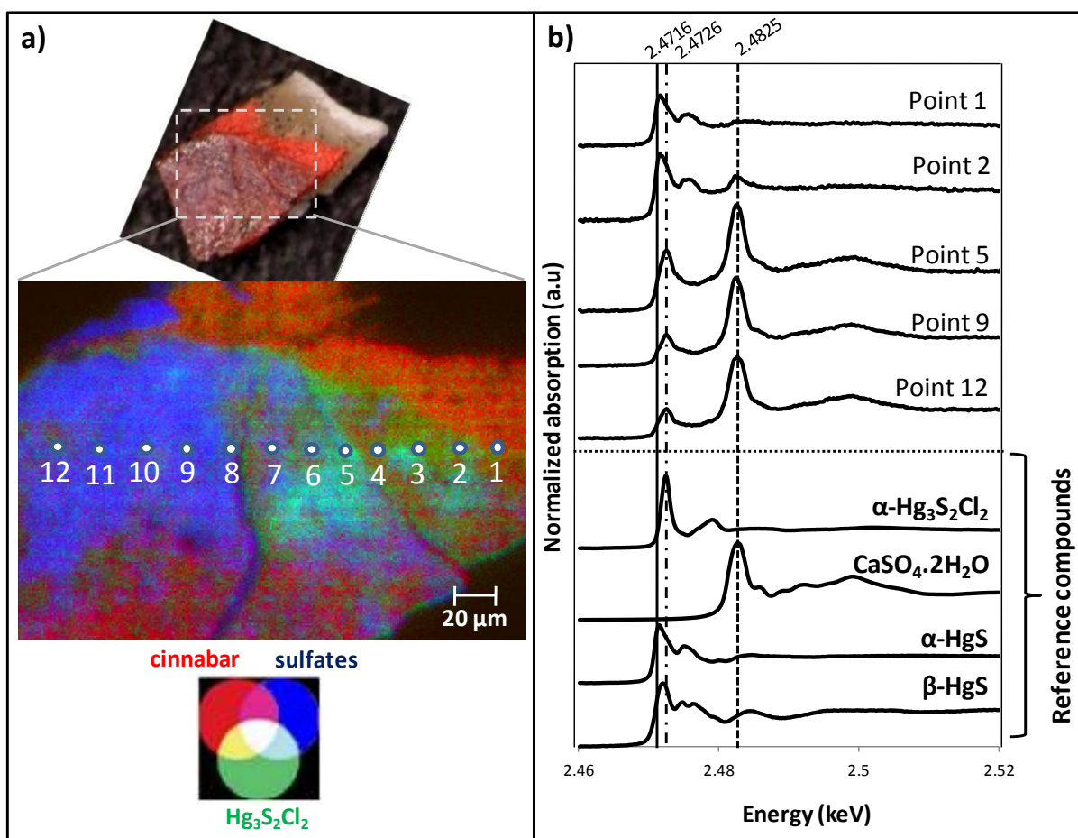
Figure 2.4.: a) RGB composite of three S-K \alpha intensity maps representing sulfur acquired at 2.4716 keV (cinnabar, red), 2.4726 keV ( \text{Hg}_3\text{S}_2\text{Cl}_2 compounds, green) and 2.4825 keV (sulfates, blue), corresponding to the dashed rectangle in the visible image of sample Ru-A; b) \mu -XANES spectra of some of the twelve points in the map in a) compared to spectra of reference compounds (metacinnabar, cinnabar, gypsum, corderoite).
