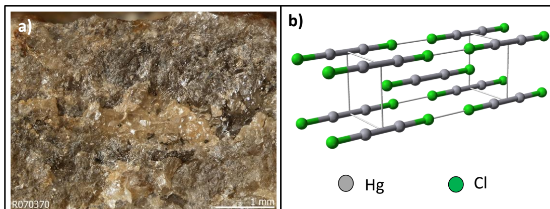
Figure 1.5.: a) Visible image of a calomel ore [ http://rruff.info/ ]; b) crystal structure of Hg_2Cl_2 [ http://en.wikipedia.org/wiki/ ].
