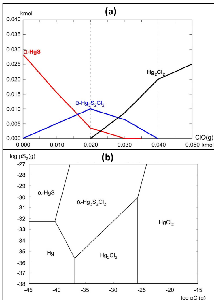
Figure 4.10.: a) Thermodynamic simulation of reactions occurring during artificial ageing experiments when adding ClO_{(g)} to \alpha -HgS (s) at 25°C; b) Diagram of Hg-S-Cl phases stability vs. the fugacities of S_{2(g)} and Cl_{(g)} at 25°C.
