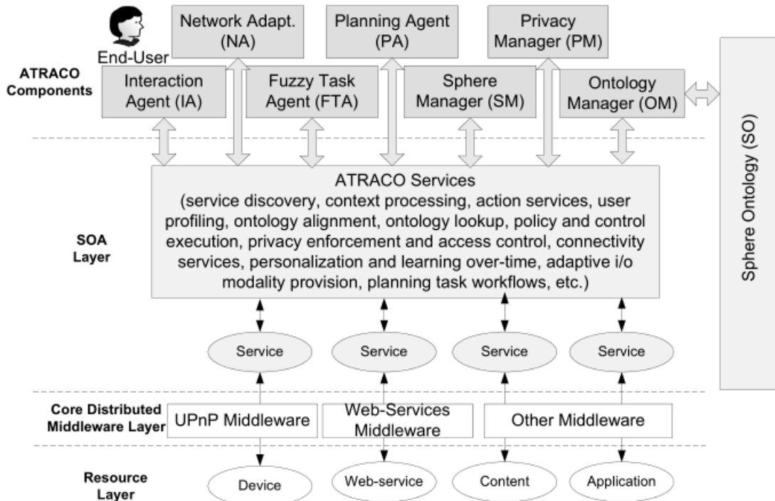
FIGURE 27 - L'ARCHITECTURE SYSTEME ATRACO, EXTRAIT DE (GOUOMOPOULOS ET AL. 2010)
