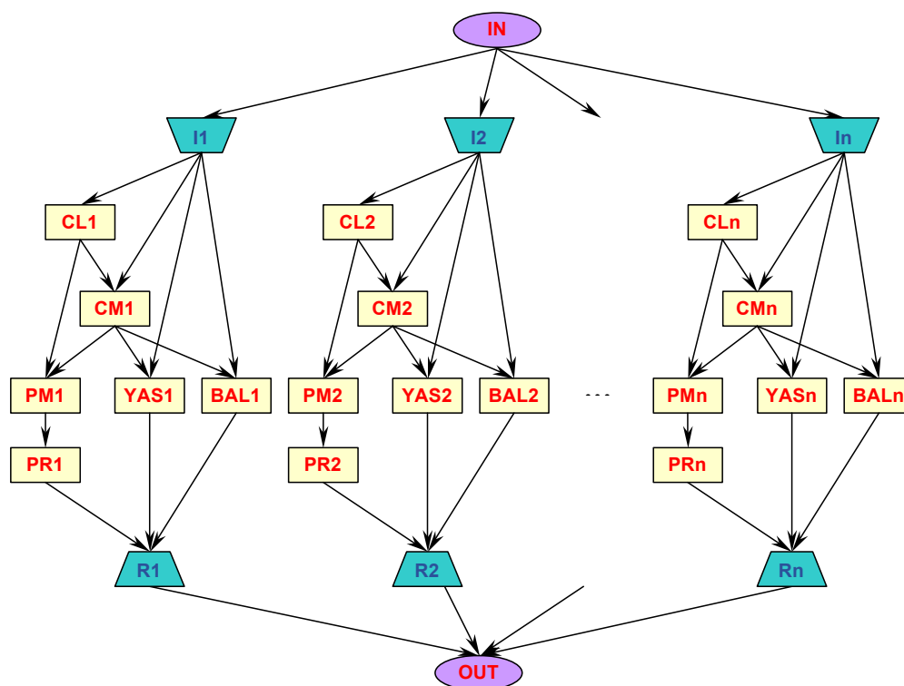
Figure 2.4: DAG jobs of the Bronze Standard application for n inputs
