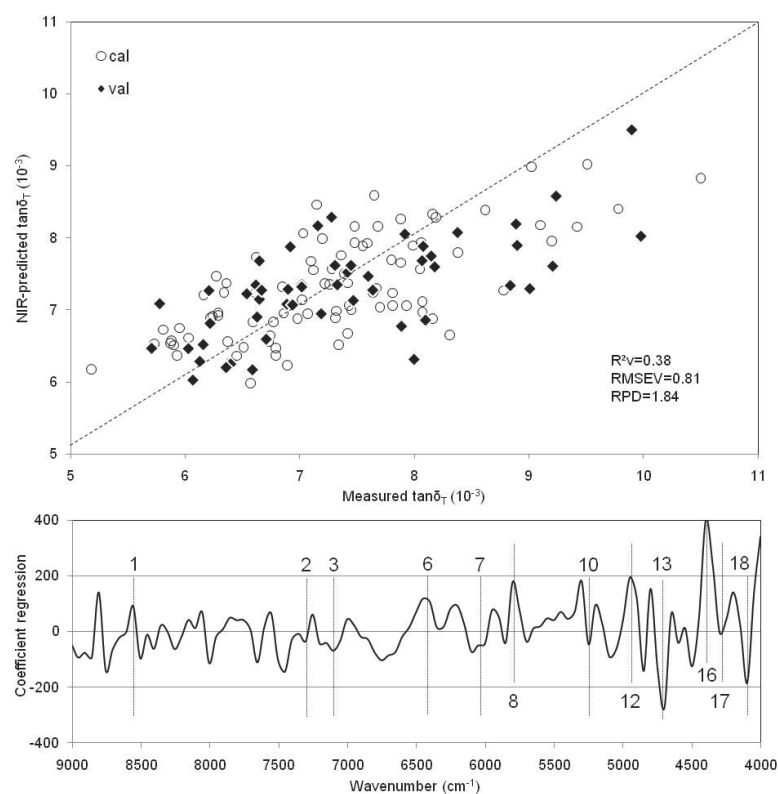
Figure 6. NIR-predicted versus measured values plot for loss tangent ( \tan \delta_T ) based on the first derivative of NIR spectra for both training (open circles) and test sets (filled rhombs) and regression coefficients for PLS model predicting \tan \delta_T .
