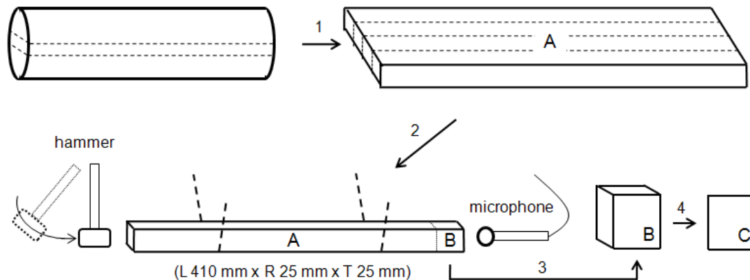
Figure 1 - Procedure of sampling. Clear wood specimens were cut from central boards (A). Dynamic tests for determining E , E/\rho and G followed by static tests for MOR were performed in each specimen. After testing, a small sample measuring 25 mm \times 25 mm \times 25 mm (B) was removed from intact wood for \rho measurement, and a 2 mm section sample (C) for XRD measurements.
