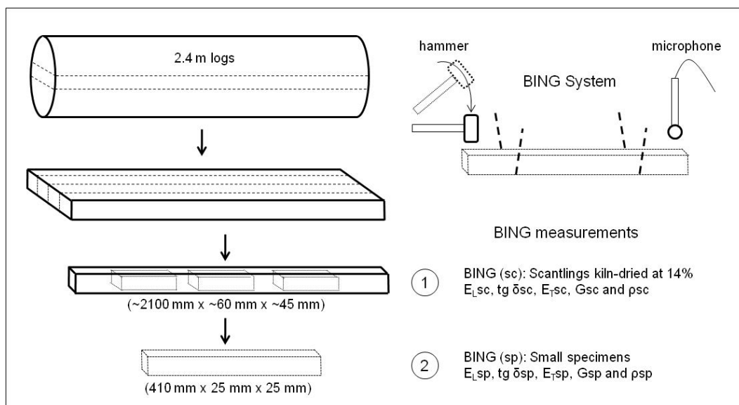
Figure 1 - Procedure of sample preparation and acoustic measurements.
