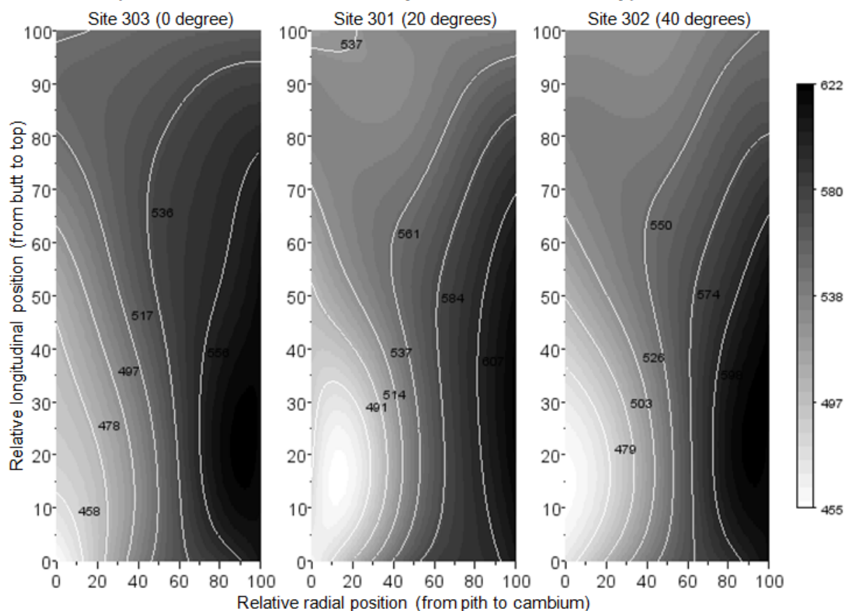
Figure 39 - Spatial variation of wood basic density ( \text{kg m}^{-3} ) in Eucalyptus urophylla x grandis trees
