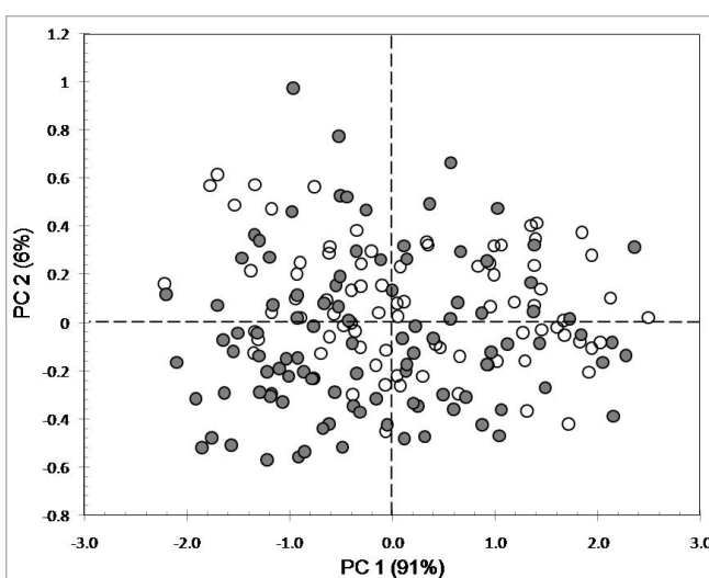
Figure 2. Two-dimensional scatter plot of scores for PC1 and PC2 from principal component analysis (PCA) of the original NIR spectra of data set 1 (grey circles) and data set 2 (white circles).
