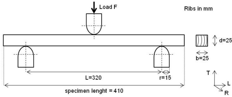
Figure 17 - Schema for three-point statistic bending test
