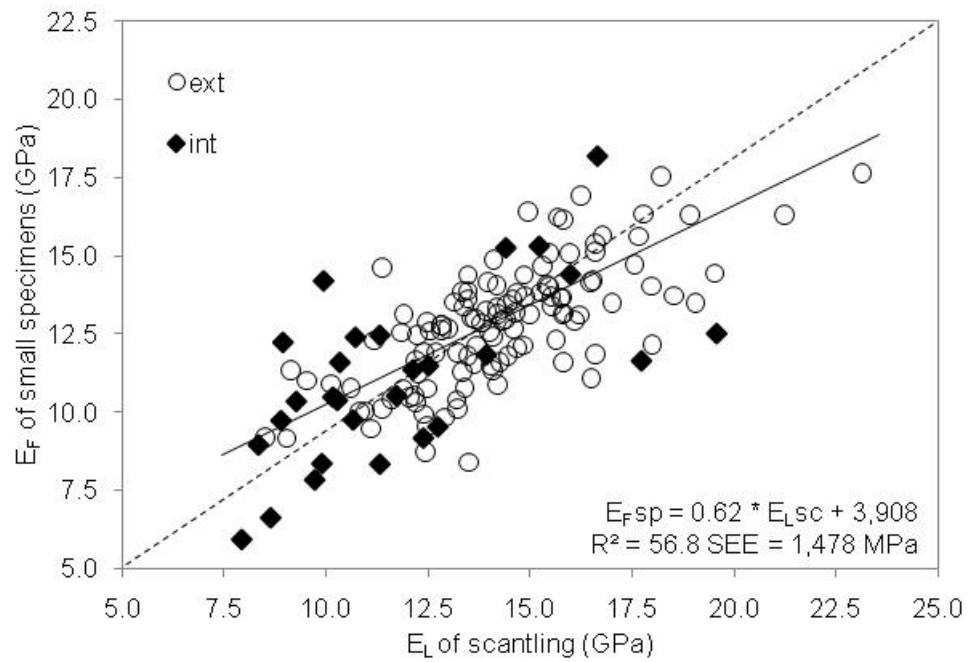
Figure 3 - Correlation between the modulus of elasticity in longitudinal test of scantlings ( E_{Lsc} ) and the averaged modulus of elasticity by beam in flexural test of small specimens ( E_{Fsp} ) of Eucalyptus grandis x urophylla . The scantlings sampled from extern or intern regions of the logs are represented by open circles and full rhomb, respectively.
