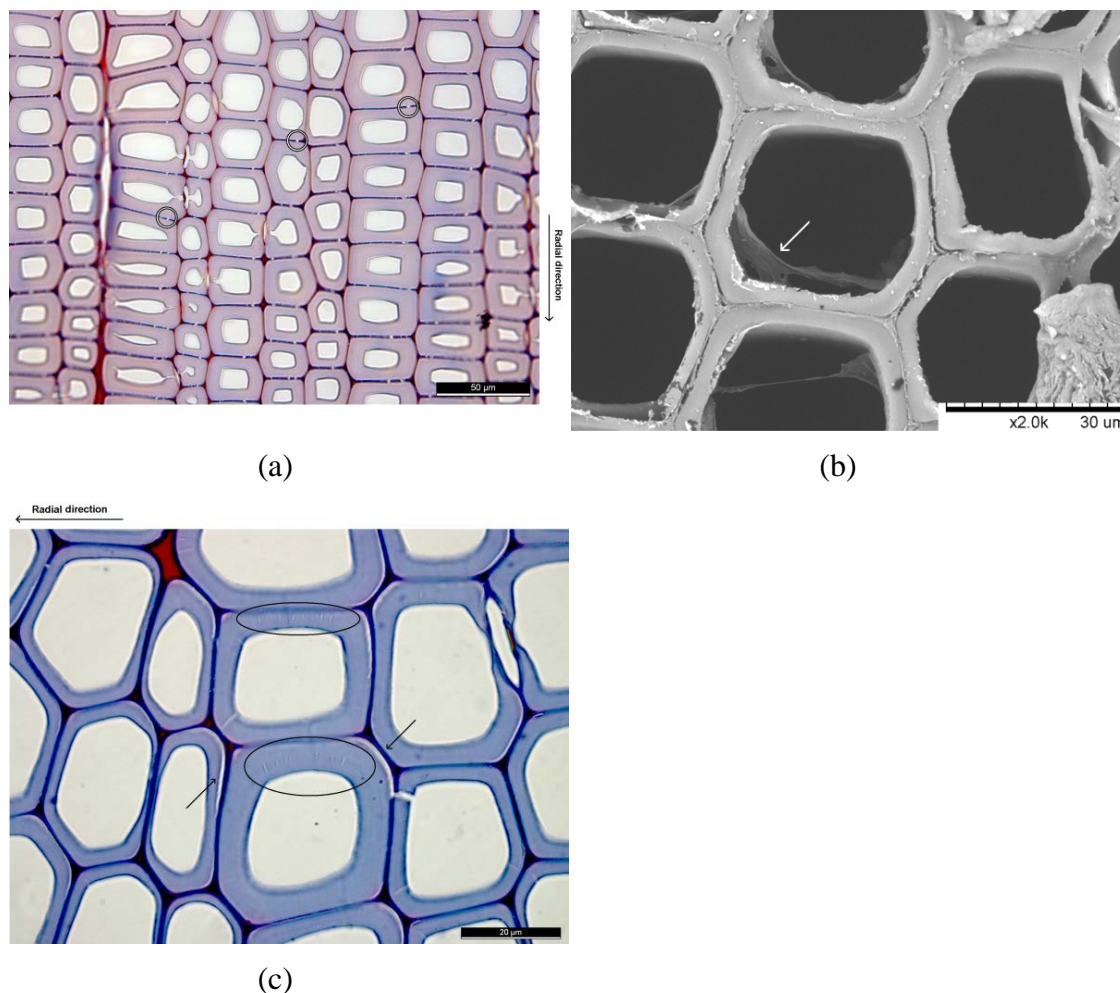
Figure 3.9: Optical and scanning electron micrographs. a) Optical micrograph of 200-year-old aged wood. Punctual degradations are visible in the middle lamella (circled). b) Scanning electron micrograph of 500-year-old aged wood. Delamination of the S3 wall from the secondary wall is visible (arrow). c) Optical micrograph of 200-year-old aged wood. Delamination between the middle layer and the secondary wall (arrows) and radial cracking in the secondary wall (circled) are visible.
