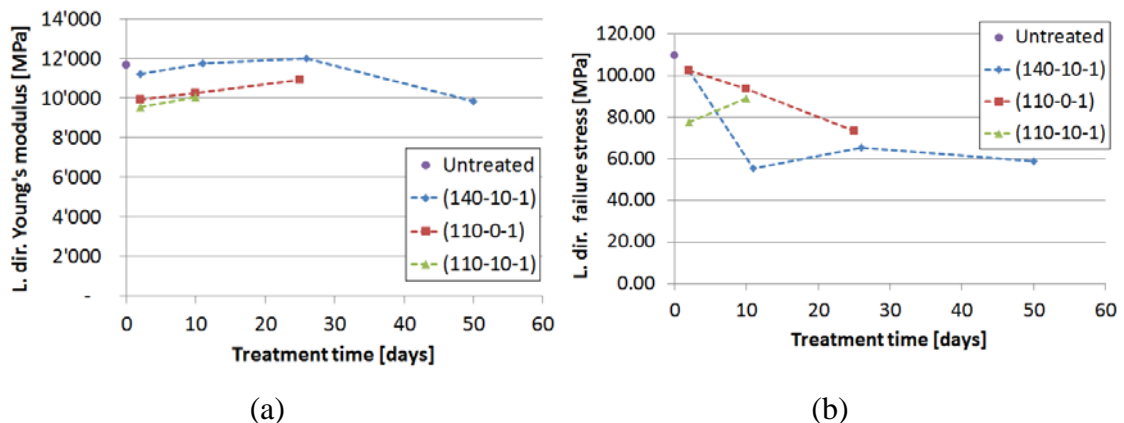
Figure 3.19: Longitudinal Young's modulus in (a) and longitudinal failure stresses in (b) of non-aged and thermally aged samples by TH treatments.
