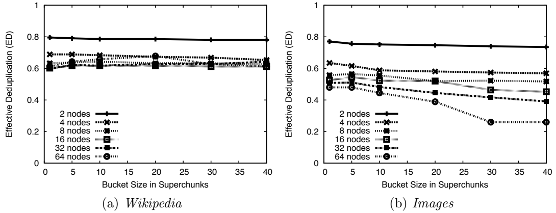
Figure 2.11: Effective Deduplication (ED) for both datasets for different bucket and cluster sizes.
