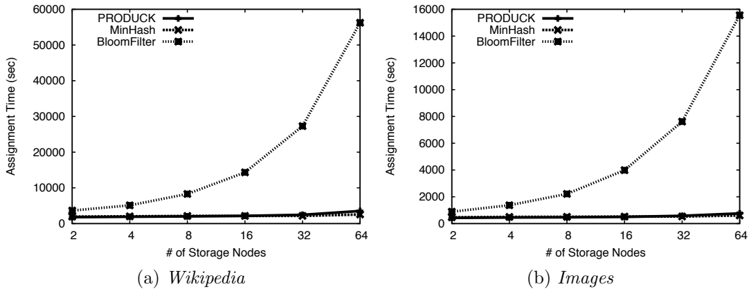
Figure 2.9: Assignment Time (AT) in seconds for all datasets for PRODUCK, BLOOM-FILTER and MINHASH as a function of the cluster size.
