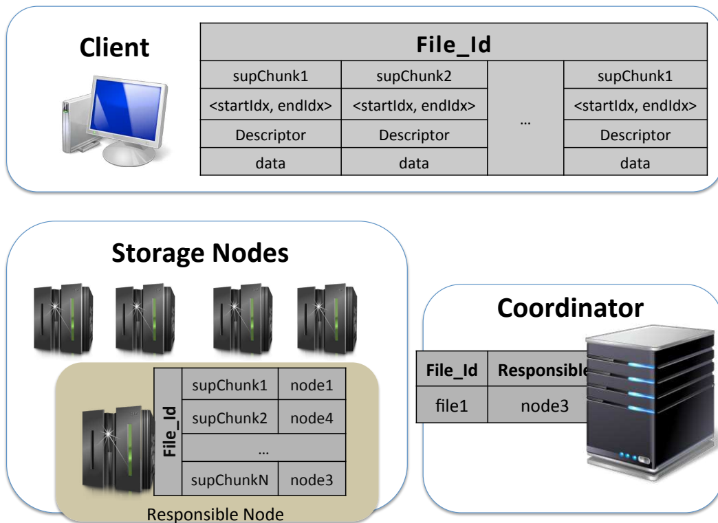
Figure 2.5: System Architecture
