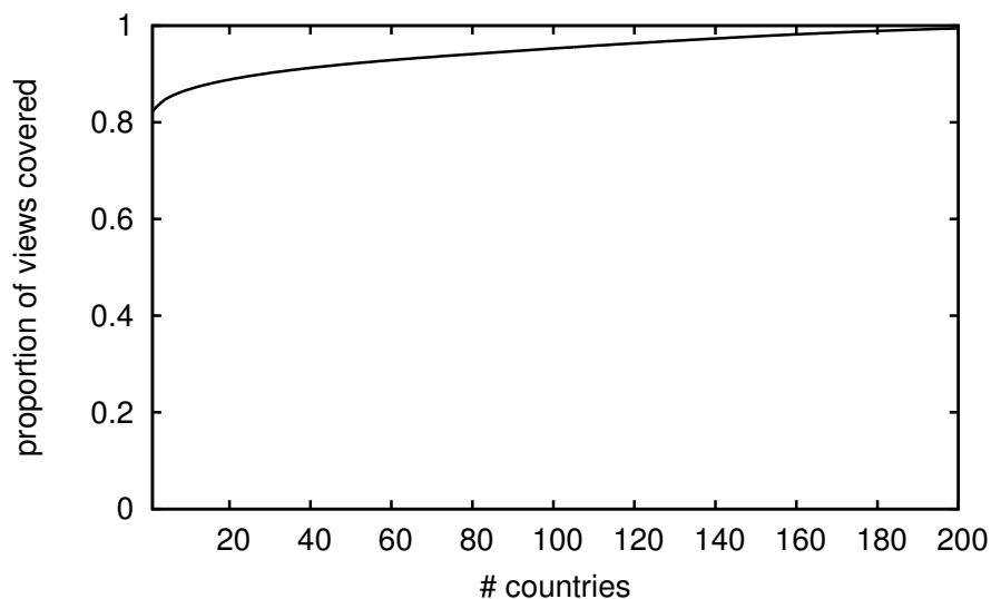
Figure 3.7: Views covered by placing replicas of a video V in top-countries of the VSV of V 's first related video, normalized by the number of views covered when using V 's actual VSV.
