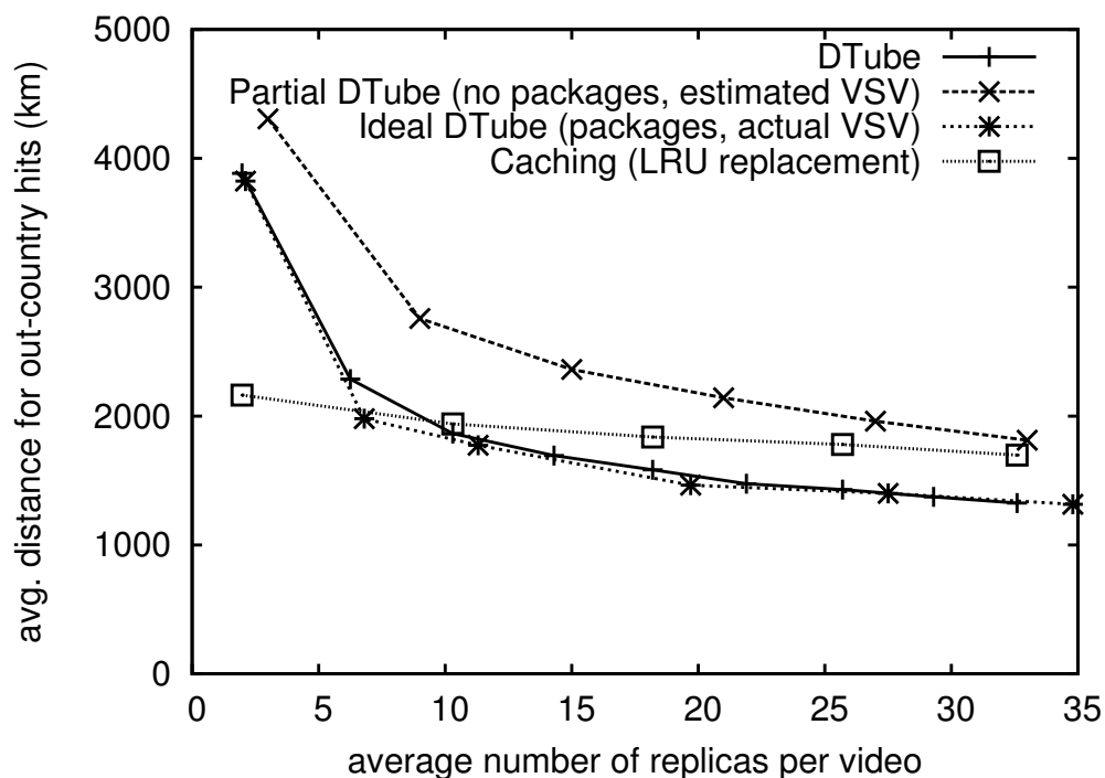
Figure 3.10: Average distance to storage node for out-country requests with DTUBE and caching.
