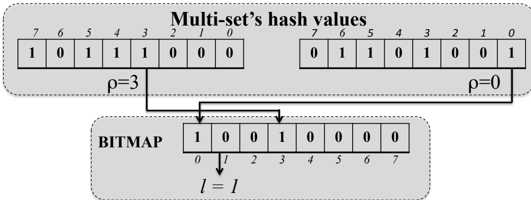
Figure 2.6: PCSA multi-set cardinality estimation.
