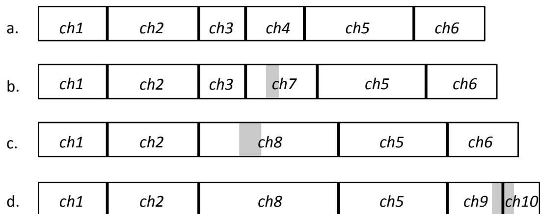
Figure 2.3: Chunks of a file after various modifications. Gray regions are the modifications while the vertical lines are the chunk boundaries.
