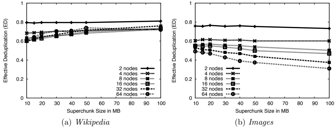
Figure 2.10: Effective Deduplication (ED) for both datasets for different superchunk and cluster sizes.
