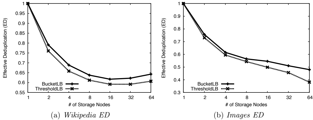
Figure 2.13: Effective Deduplication (ED) for both datasets for two load balancing strategies (i) our bucket -based one, here called BucketLB , and (ii) the one from [DDL + 11], namely ThresholdLB , where the storage load of a node is not allowed to deviate by more than 5% from the average load in the system.
