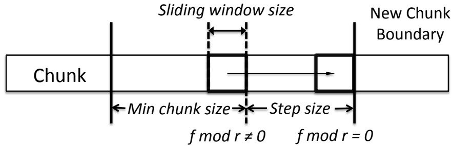
Figure 2.2: Content-Based Chunking Principles.
