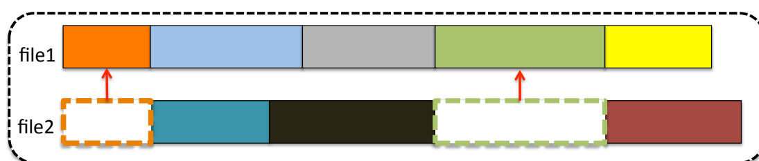
Figure 1.4: Deduplication Example
