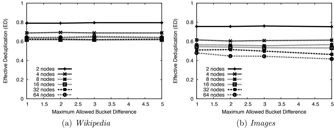
Figure 2.12: Effective Deduplication (ED) for both datasets for different values of maximum allowed bucket difference between the most and the least loaded nodes and across different cluster sizes.
