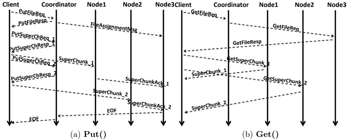
Figure 2.7: Messages exchanged during storing and retrieving a file in PRODUCK.
