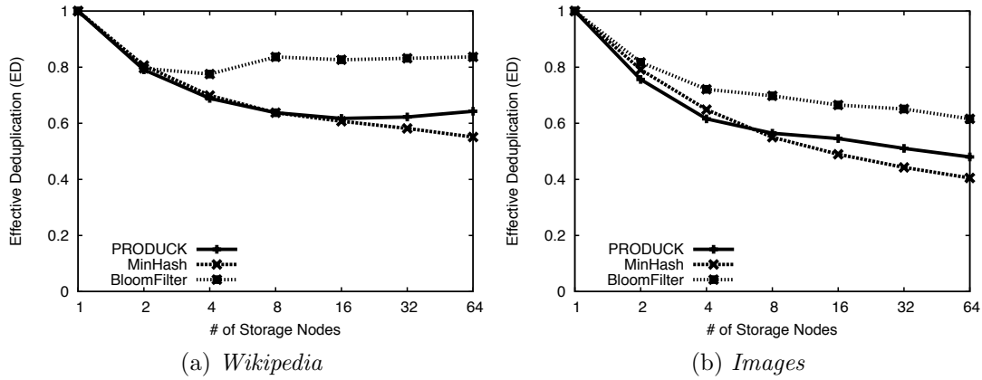
Figure 2.8: Effective Deduplication (ED) for all datasets for PRODUCK, BLOOM-FILTER and MINHASH as a function of the cluster size.
