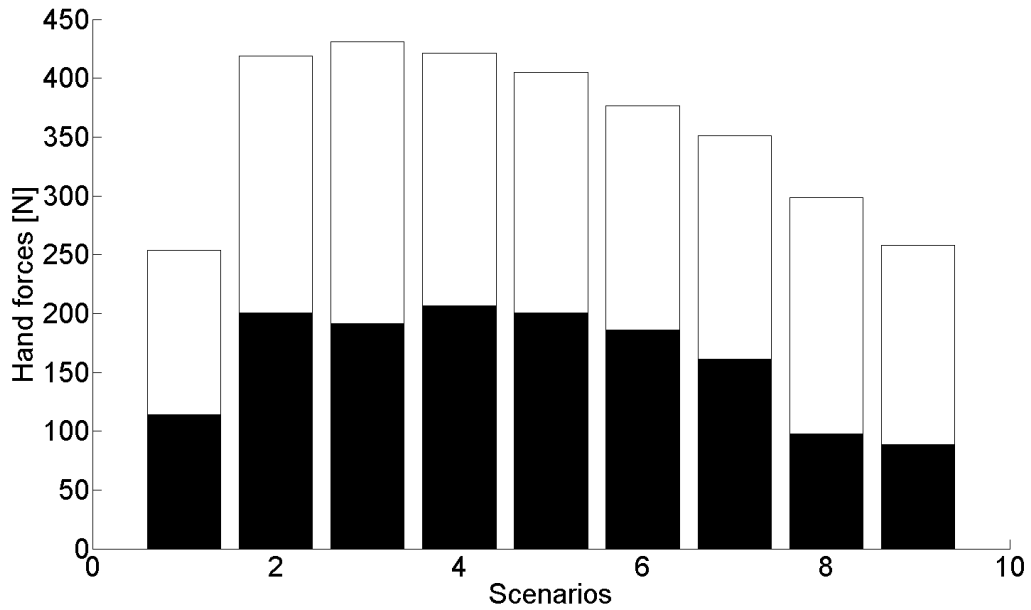
(a) Mean (black) and maximal (white) values of trailing hand forces for all optimization scenarios.
