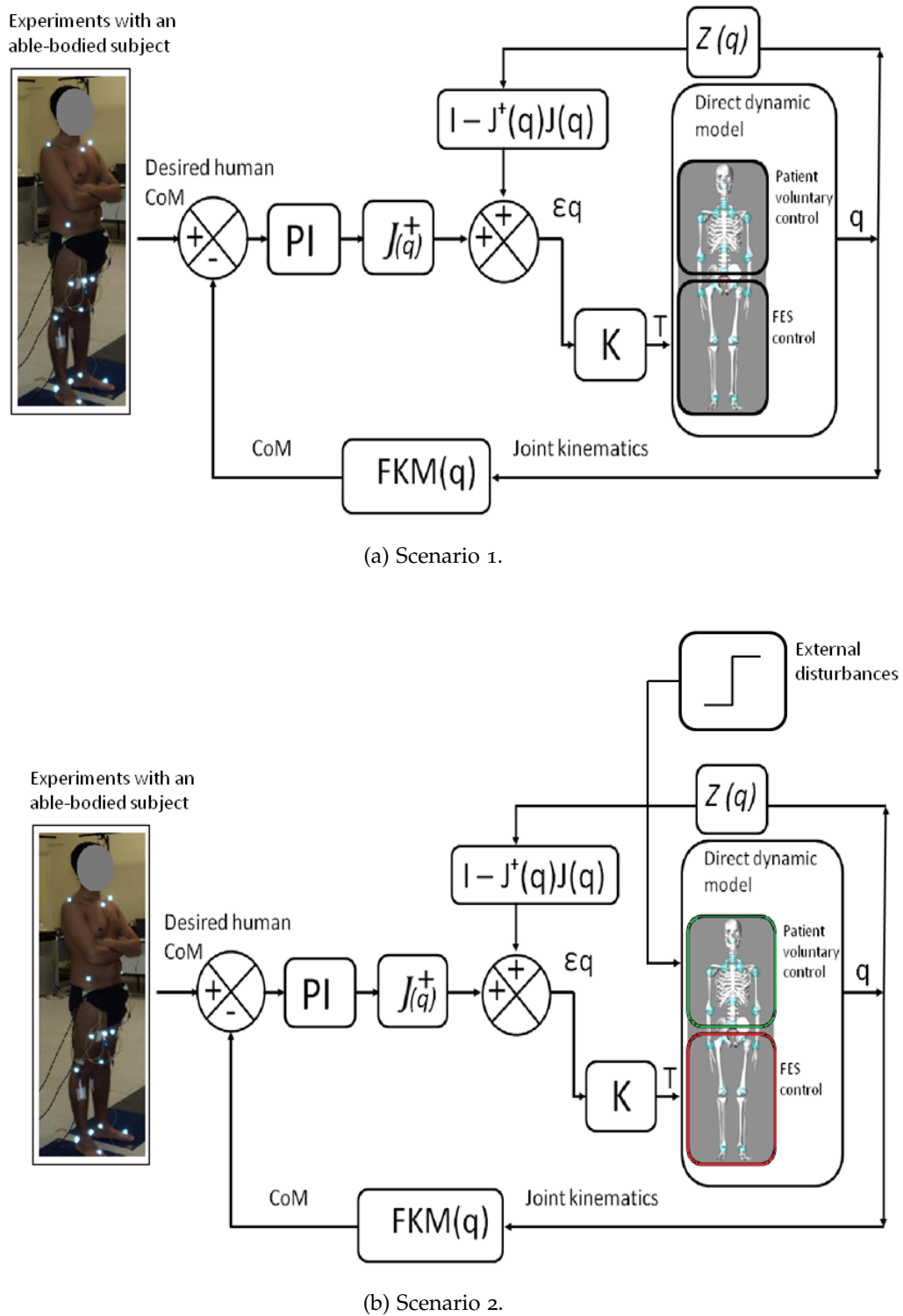
Figure 54: Block diagram of the two scenarios used to test the robustness of the proposed postural controller.
