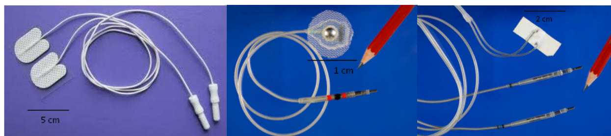
(a) Transcutaneous electrode.
