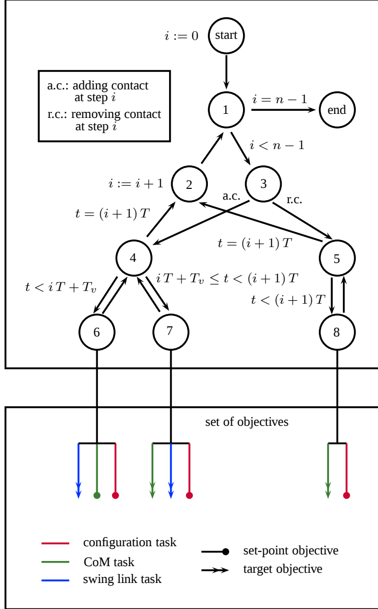
FIGURE 4.3. The finite-state machine (note: contains color information). States are represented as circles (the numbers inside have no particular meaning) and transitions as arrows between states. Labels next to transitions are the conditions for the transitions to be triggered. Transitions without labels are automatically triggered (condition always true). Labels next to states, when present, are actions performed when the machine reaches the states.
