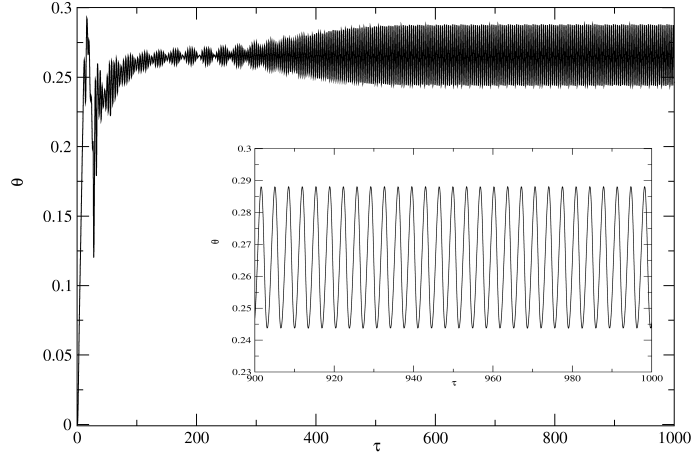
Figure 3.7 – Reduced temperature evolution \theta = (T - (T_h + T_c)/2)/(T_h - T_c) at point 1 as a function of dimensionless time \tau \equiv t\alpha_0/W^2 .
