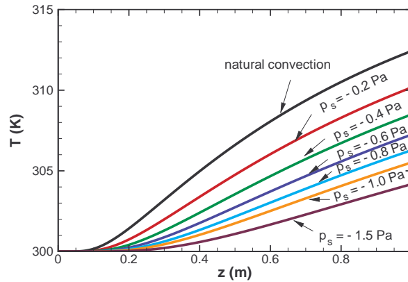
Figure 5.9 – Variations of the temperature along the channel axis according to the pressure drop at the outlet section for natural and mixed convection ( D = 2 \text{ cm} , H = 1 \text{ m} , \Delta T = 20 \text{ K} ).
