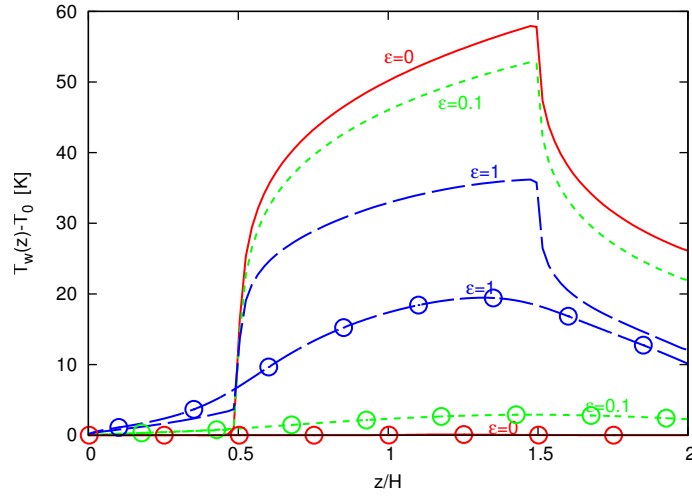
Figure 6.9 – Variation of the heated wall temperature with height according to the emissivity of the vertical walls for D = 3.8 \text{ cm} and q_w = 300 \text{ W/m}^2 . The open circle symbols are for the adiabatic wall.
