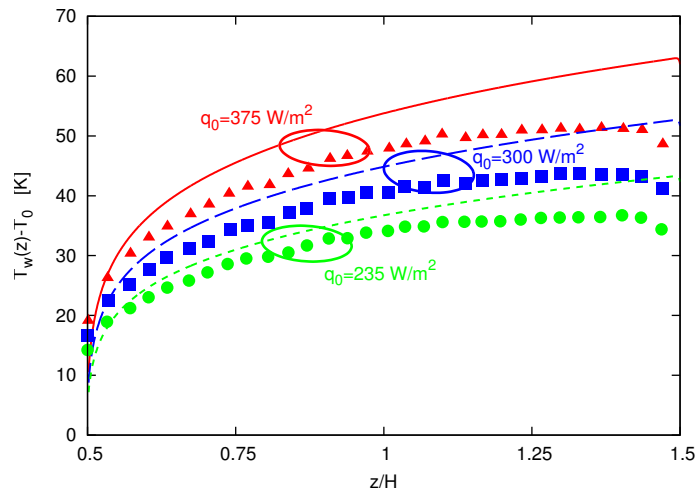
Figure 6.2 – Variations of the heated wall temperature versus z/H for the three heating rates studied by Webb et Hill [161], D = 2.02\text{ cm} . Symbols are experimental data from [161].
