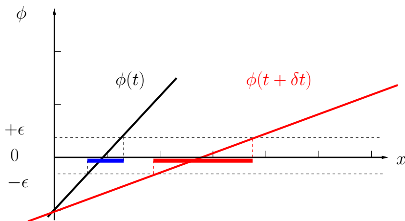
Figure 2.2 – Illustration of transport of the level set function on the distance function
