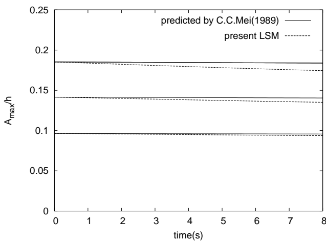
(a) Damping rate of solitary waves.
