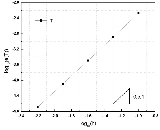
(b) Temperature
