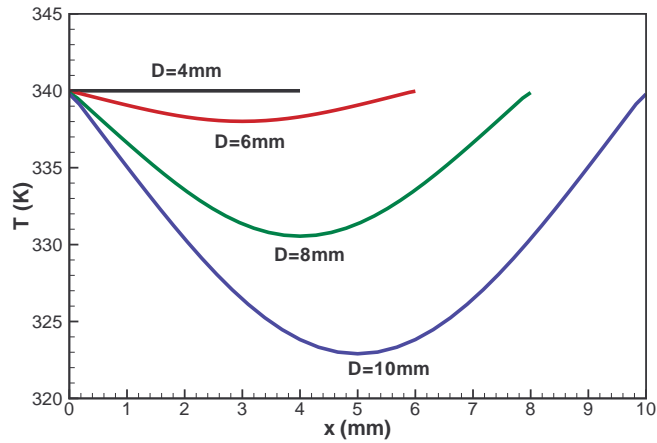
Figure 4.4 – Natural convection: temperature profile at the outlet section for various plate spacings.
