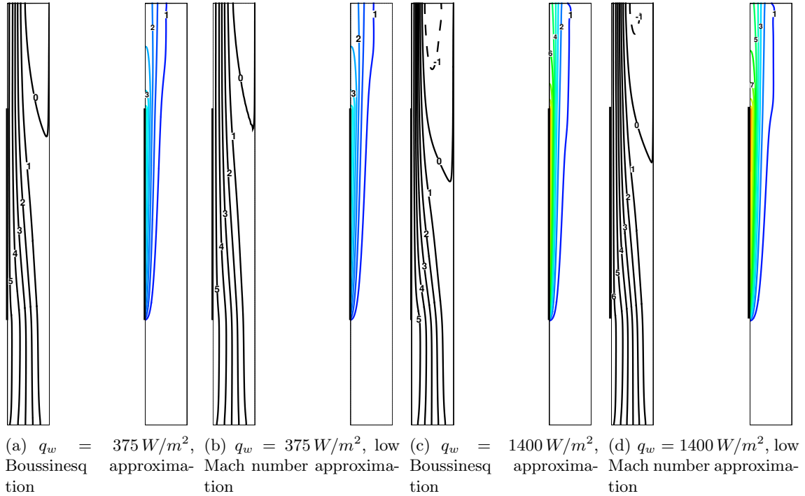
Figure 6.17 – Natural convection. Streamlines \psi_i/[g/(m \cdot s)] = 0.5 \times i (left) and isotherms T_i/[K] = 290 + 20 \times i (right) for (a) q_w = 375\text{ W/m}^2 and the Boussinesq approximation, (b) q_w = 375\text{ W/m}^2 and the low Mach number approximation, (c) q_w = 1400\text{ W/m}^2 and the Boussinesq approximation, (d) q_w = 1400\text{ W/m}^2 and the low Mach number approximation. The horizontal scales are enlarged by 50%.
