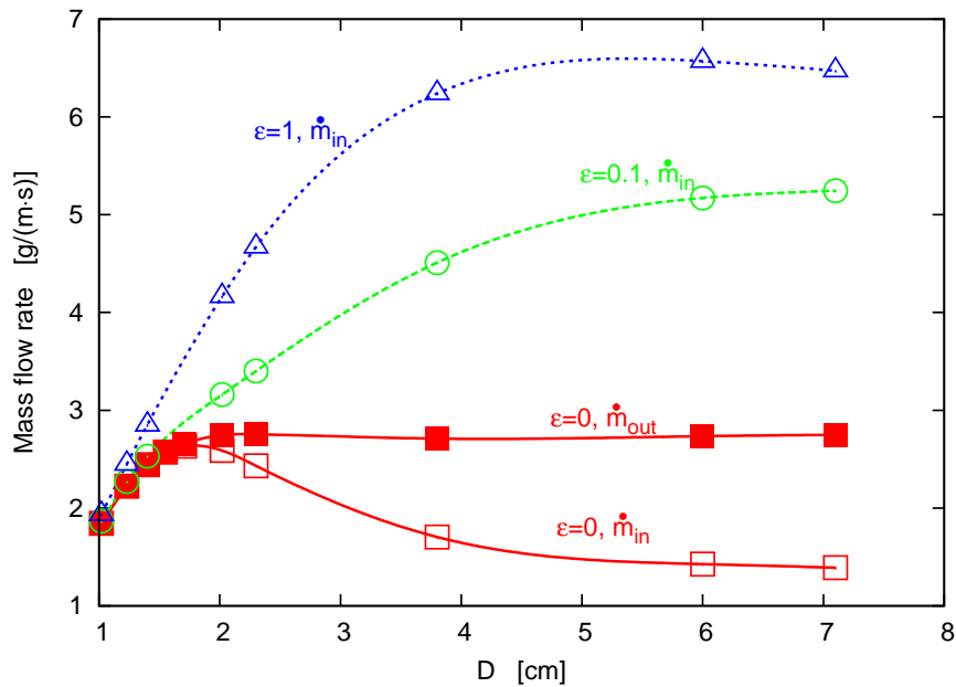
Figure 6.13 – Mass flow rate versus the wall spacing for three wall emissivities, q_w = 300 \text{ W/m}^2 ; \dot{m}_{out} = 0 for \epsilon = 0.1 and \epsilon = 1 .
