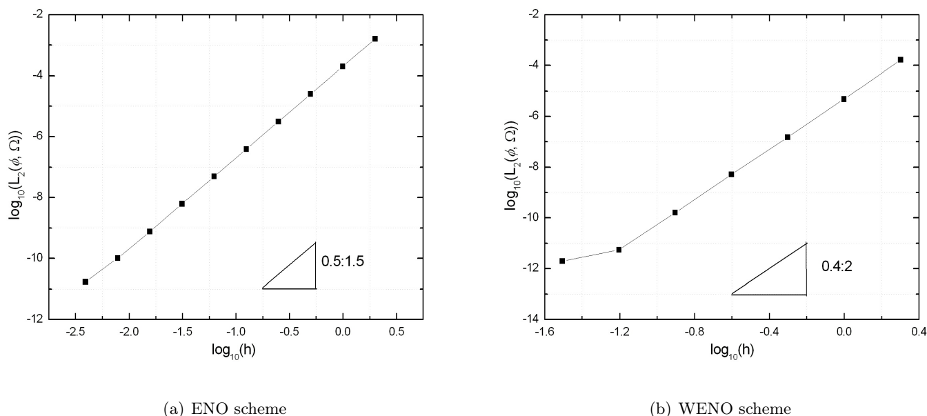
Figure 3.1 – One dimensional test problem for transport equation. L_2(\phi, \Omega) errors for ENO and WENO schemes. Initial condition (3.4).
