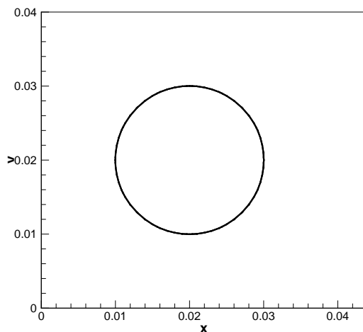
Figure 3.22 – Air bubble at t = 0.05 s
