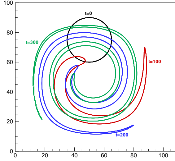
Figure 3.15 – Stretching of a circular fluid element with velocity field (3.8).
