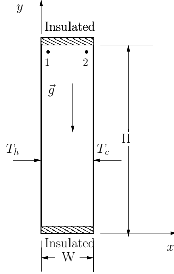
Figure 3.6 – Differentially heated cavity, H/W = 8 . Coordinates of two probes: (x_1, y_1) = (0.1810 W; 7.3700 W) and (x_2, y_2) = (0.8190 W; 7.3700 W) .
