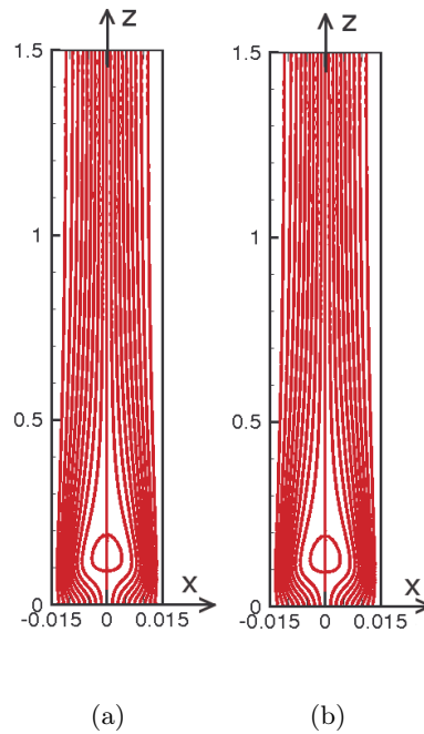
Figure 5.3 – Flow recirculation for mixed convection (a) prescribed inlet velocity , w_0 = 0.05 \text{ m/s} (b) overpressure at the outlet section p_s = 1.4 \text{ Pa} ( D = 3 \text{ cm} , H = 1.5\text{m} , \Delta T = 20 \text{ K} ).
