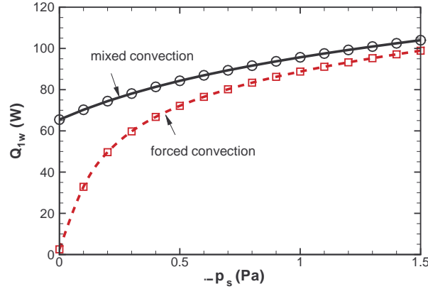
Figure 5.8 – Variations of the heat flux transferred at one of the walls according to the pressure drop at the outlet section for forced and mixed convection ( D = 2 \text{ cm} , H = 1 \text{ m} , \Delta T = 20 \text{ K} ).
