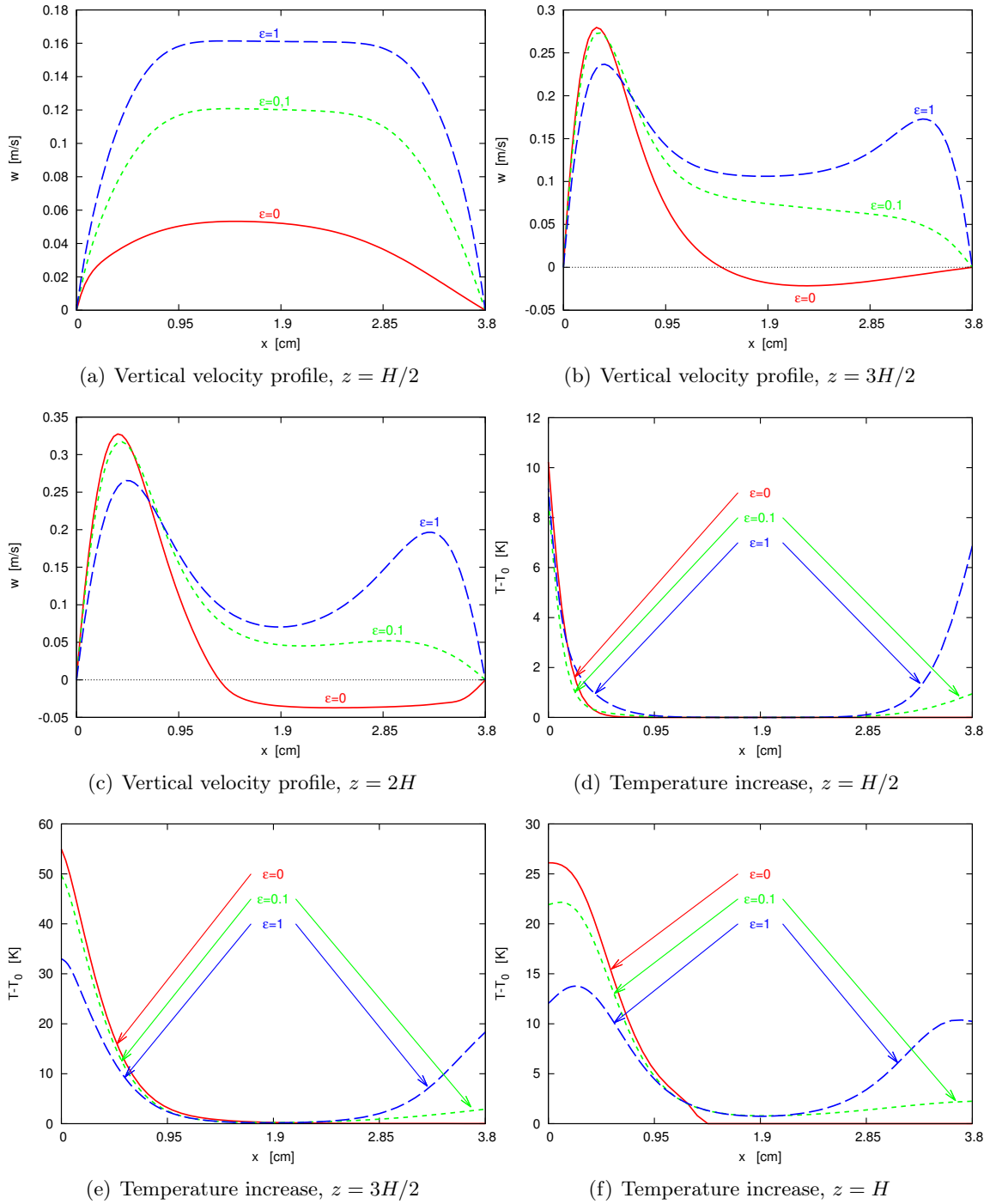
Figure 6.10 – Vertical velocity profiles (a) at the inlet of the heated wall section ( z = H/2 ), (b) at the outlet of the heated wall section ( z = 3H/2 ), (c) at the outlet section of the channel ( z = 2H ) and temperature gap profiles (d) at the inlet of the heated wall section ( z = H/2 ), (e) at the outlet of the heated wall section ( z = 3H/2 ), (f) at the outlet section of the channel ( z = 2H ) as a function of the emissivity of the vertical walls ( D = 3.8 cm, q_w = 300 W/m 2 ).
