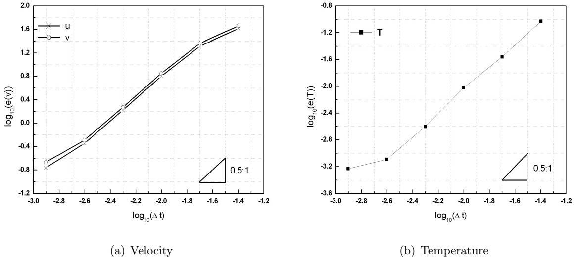
Figure 3.4 – Variation of the relative temporal error as a function of the time step \Delta t .
