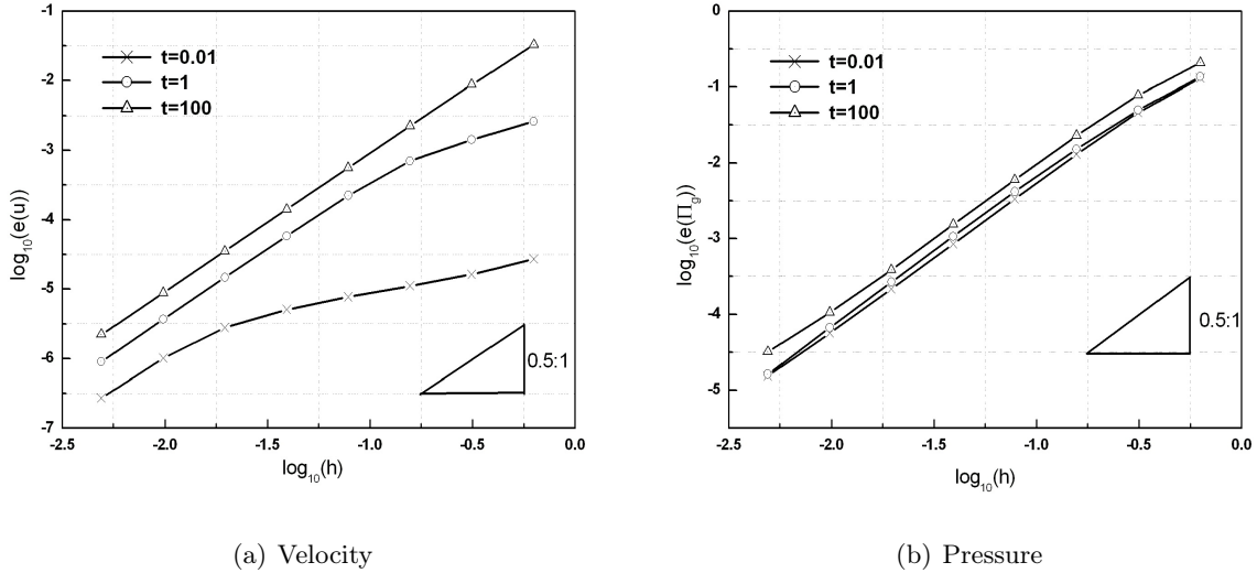
Figure 3.1 – Variations of relative spatial error as a function of the grid size h at different time.
