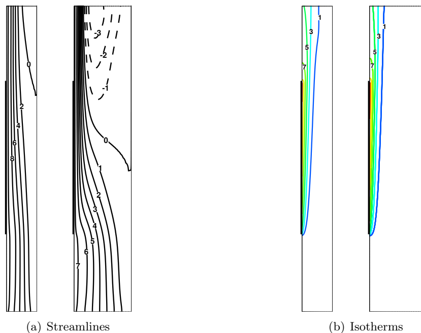
Figure 6.7 – Pure natural convection. (a) Streamlines \psi_i/[g/(m \cdot s)] = 0.25 \times i and (b) isotherms T_i/[K] = 290 + 5 \times i for D = 2.02 \text{ cm} (left) and D = 3.8 \text{ cm} (right), q_w = 300 \text{ W/m}^2 . The horizontal scales are enlarged by 50%.
