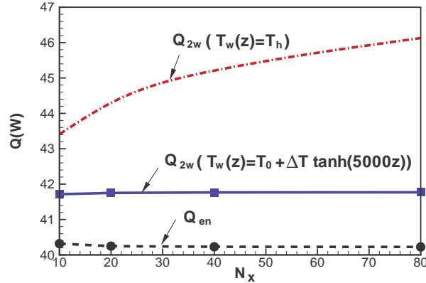
Figure 4.2 – Natural convection: variations of heat flux versus the number of grid points in the x -direction ( n_z = 50n_x ) for D = 6 \text{ mm} , H = 0.1 \text{ m} , L = 1 \text{ m} , \Delta T = 40 \text{ K} . Q_{2w} is the wall heat flux for non-regularized wall temperature (Eq. 4.25) or for regularized wall temperature (Eq. 4.27). Q_{en} is the enthalpy flux (Eq. 4.14).
