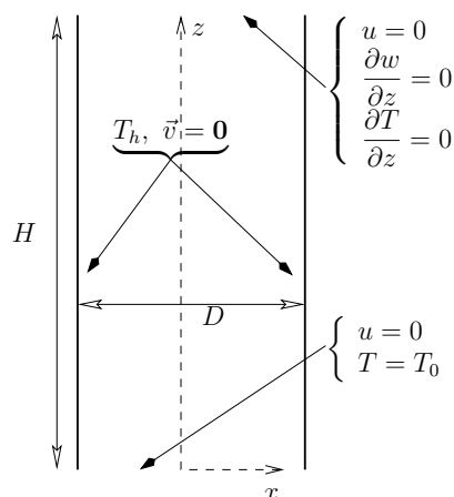
Figure 5.1 – The physical model of mixed convection in a vertical channel. The full boundary conditions are written in Eqs. (5.5-5.7) for the three cases investigated.
