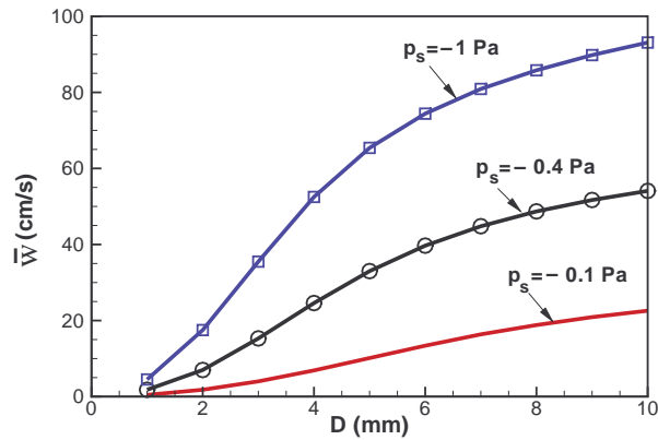
Figure 4.10 – Forced convection: variations of the mean flow velocity versus the plate spacing for various p_s .
