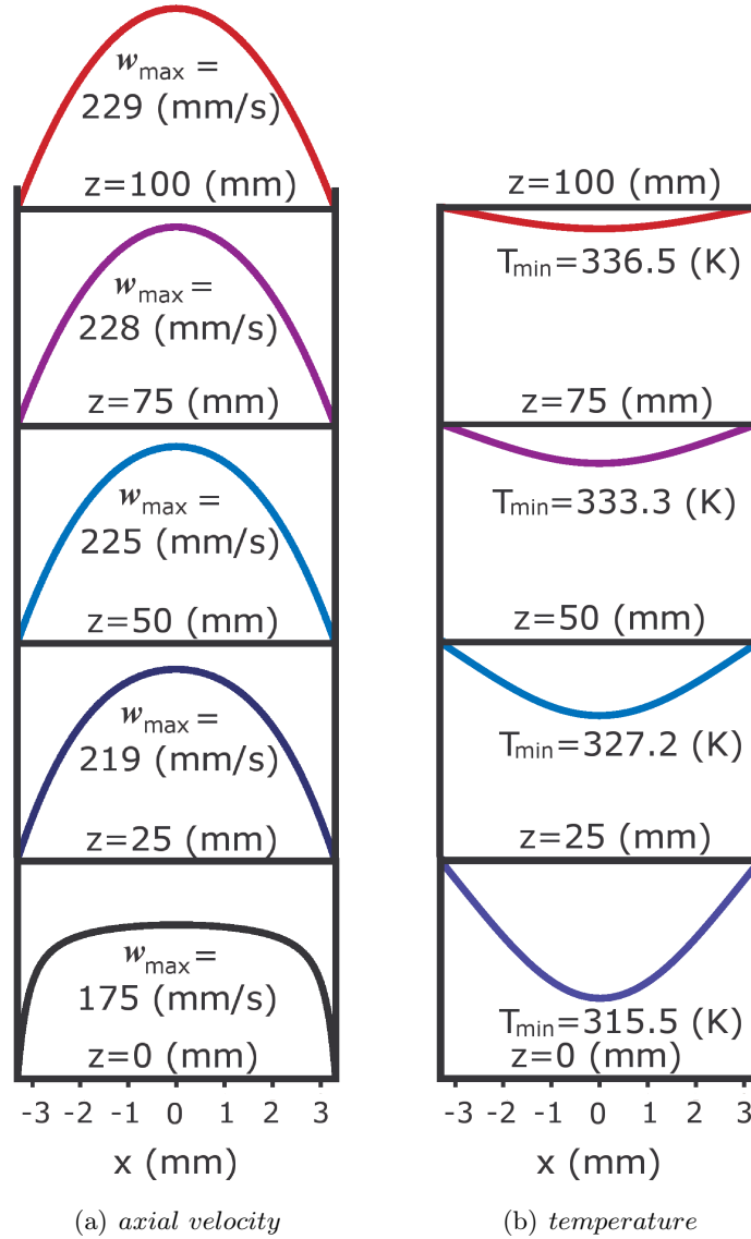
Figure 4.7 – Natural convection: axial velocity and temperature profiles at various heights for the optimal spacing, D_{opt} = 6.62 \text{ mm} .
