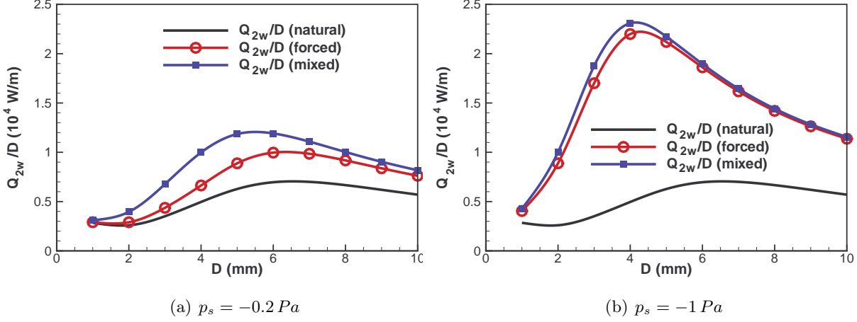
Figure 4.11 – Mixed convection : variations of the ratio Q_{2w}/D versus the plate spacing for forced and mixed convection.
