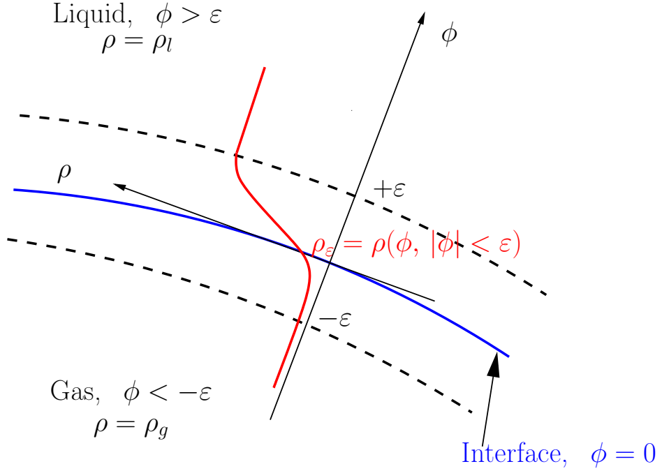
Figure 2.1 – Demonstration of density jump
