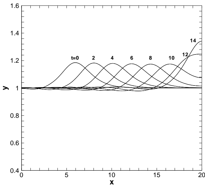
(a) Traveling trains of a solitary wave.
