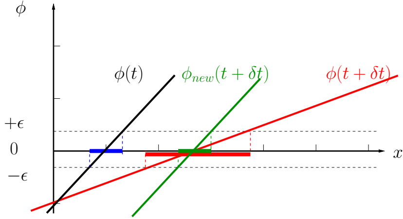
Figure 2.3 – Illustration of reinitialization method
