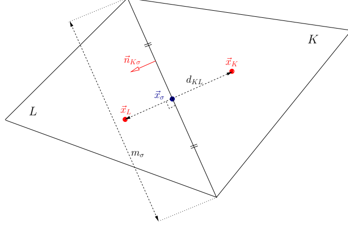
Figure 2.1 – Control volume and notations
