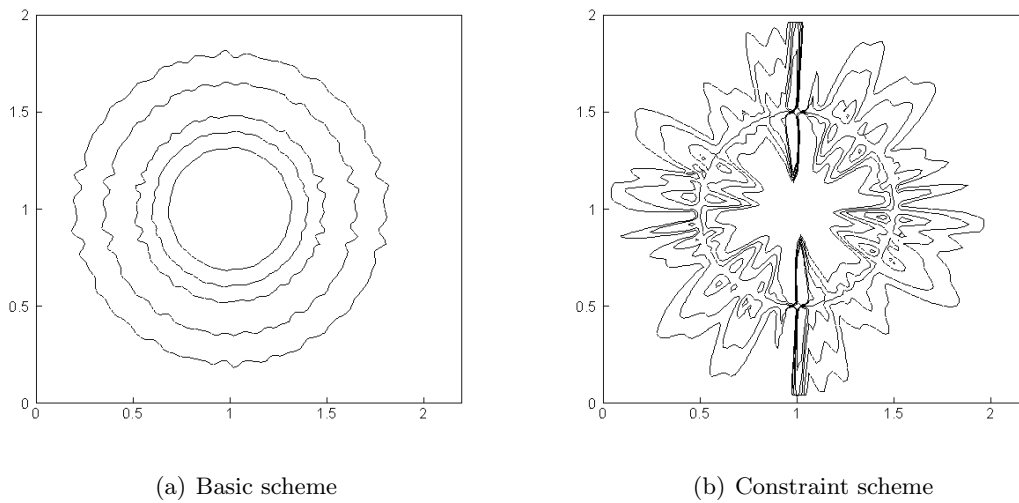
Figure 3.8 – Curvature of the signed distance function at the steady state using the ENO discretization scheme
