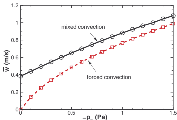
Figure 5.7 – Variations of the average velocity according to the pressure drop at the outlet section for forced and mixed convection ( D = 2 cm , H = 1 m , \Delta T = 20 K ).
