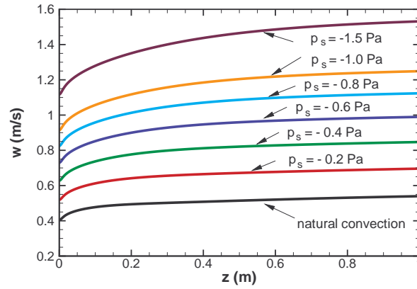
Figure 5.10 – Variations of the vertical velocity component along the channel axis according to the pressure drop at the outlet section for natural and mixed convection ( D = 2 \text{ cm} , H = 1 \text{ m} , \Delta T = 20 \text{ K} ).
