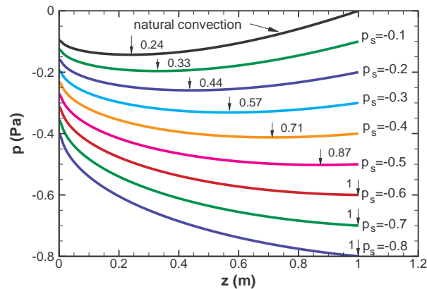
Figure 5.6 – Axial variation of pressure along the channel axis according to the outlet pressure drop ( D = 2 \text{ cm} , H = 1 \text{ m} , \Delta T = 20 \text{ K} ). The arrows indicate the positions (in m ) of the pressure minimum.
