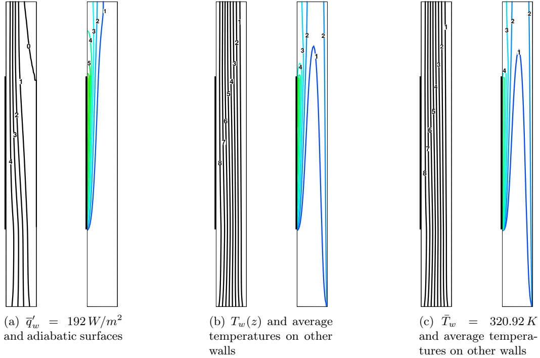
Figure 6.16 – Natural convection. Streamlines \psi_i/[g/(m \cdot s)] = 0.5 \times i (left) and isotherms T_i/[K] = 290 + 5 \times i (right) for (a) \epsilon = 0 , \bar{q}'_w = 192 \text{ W/m}^2 and adiabatic surfaces, (b) \epsilon = 0 , T_w(z) and average temperatures on other walls, (c) \epsilon = 0 , \bar{T}_w = 320.92 \text{ K} and average temperatures on other walls. The horizontal scales are enlarged by 50%.
