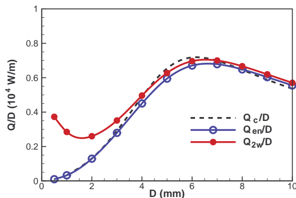
Figure 4.6 – Natural convection: variations of the ratios Q/D with the plate spacing. Q_c is the analytical solution (Eq. 4.31), Q_{2w} and Q_{en} are given by Eqs. 4.13 and 4.14.
