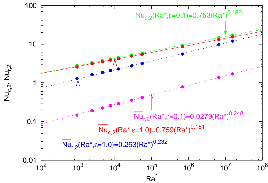
Figure 6.14 – Radiative ( \overline{Nu}_{r,2} ) and convective ( \overline{Nu}_{c,2} ) Nusselt numbers (eq. 6.30) vs the channel Rayleigh number for two emissivities of the vertical walls.
