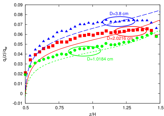
Figure 6.3 – Variations of the local radiative flux ( \epsilon = 0.1 ) to the imposed wall heat flux for three wall spacings and q_w = 300\text{ W/m}^2 . Symbols are experimental data from [161].
