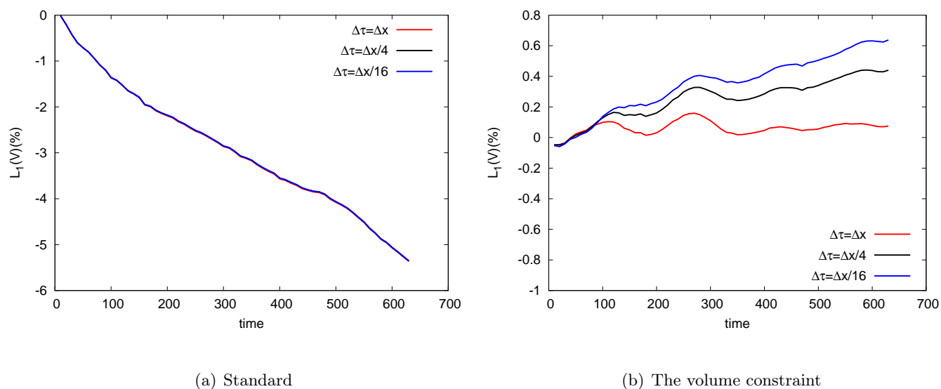
Figure 3.11 – Variation of L_1(V) with \Delta\tau with 100 \times 100 cells; the ENO scheme
