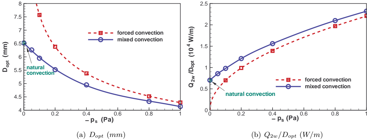
Figure 4.12 – Mixed convection : variations of D_{opt} and Q_{2w}/D_{opt} versus p_s for forced and mixed convection.
