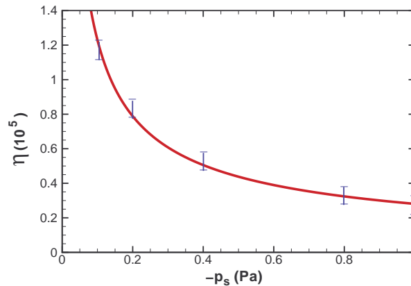
Figure 4.13 – Variations of overall efficiency \eta versus p_s for mixed convection.
