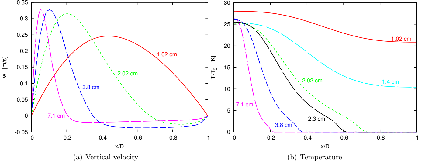
Figure 6.5 – Pure convection. (a) Vertical velocity profiles and (b) temperature at the outlet section of the channel ( z = 2H ) according to the wall spacing, q_w = 300 \text{ W/m}^2 .
