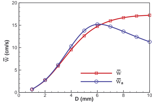
Figure 4.3 – Natural convection: comparison between the analytical ( \bar{w}_a , Eq. 4.29) and numerical ( \bar{w} ) solutions of the mean flow velocity versus the plate spacing.
