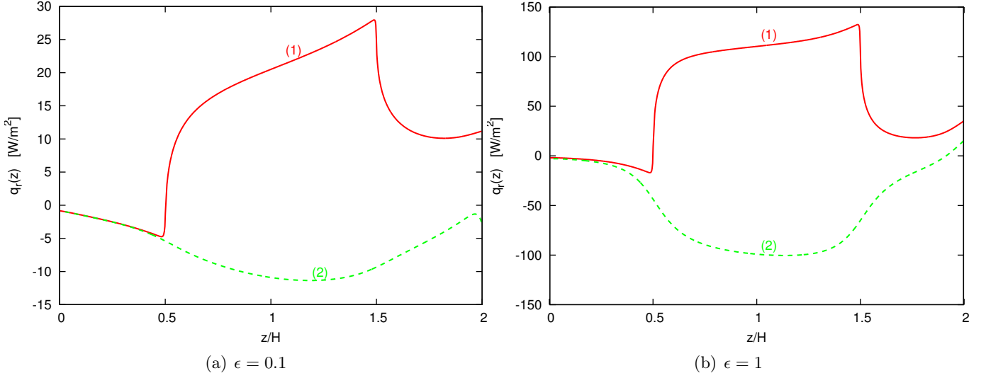
Figure 6.11 – Distribution of the net radiative heat flux densities along (1) the heated wall and (2) along the adiabatic wall, with (a) \epsilon = 0.1 and (b) \epsilon = 1 , for D = 2.02 \text{ cm} and q_w = 300 \text{ W/m}^2 .
