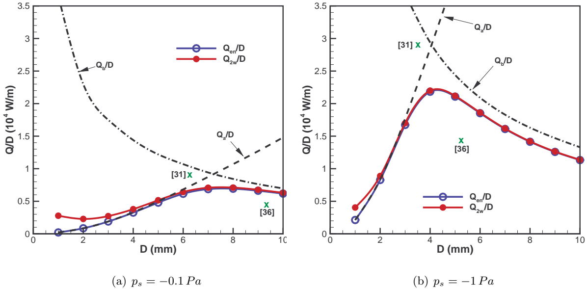
Figure 4.8 – Forced convection: variations of the ratios Q/D with the plate spacing for p_s = -0.1 Pa and for p_s = -1 Pa ( Q_a and Q_b are the asymptotic analytical solutions, Q_{2w} , Q_{en} are given by Eqs. 4.13 and 4.14, respectively). The cross symbols are for the analytical solutions given by Eq. 4.37 [26] and Eq. 4.38 [110].
