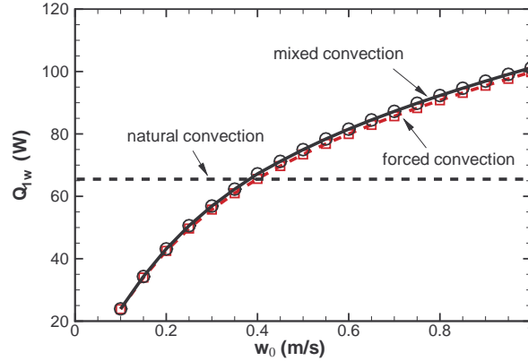
Figure 5.5 – Total heat flux transferred at one of the hot walls for forced and mixed convection according to the prescribed inlet velocity. The value for natural convection is also shown ( D = 2 \text{ cm} , H = 1 \text{ m} , \Delta T = 20 \text{ K} ).
