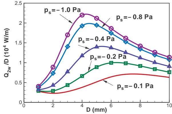
Figure 4.9 – Forced convection: variations of the ratio Q_{2w}/D versus the plate spacing for various p_s .
