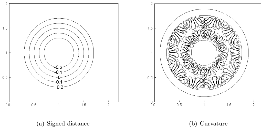
Figure 3.7 – Signed distance equation. Iso-levels at \tau = 0 and with 100 \times 100 cells
