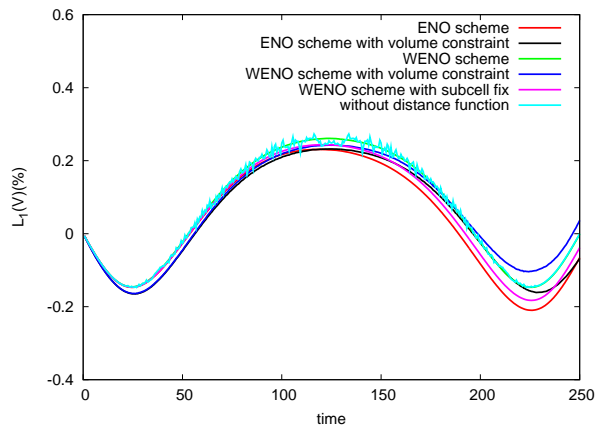
(b) T=250 with 800 \times 800 cells
