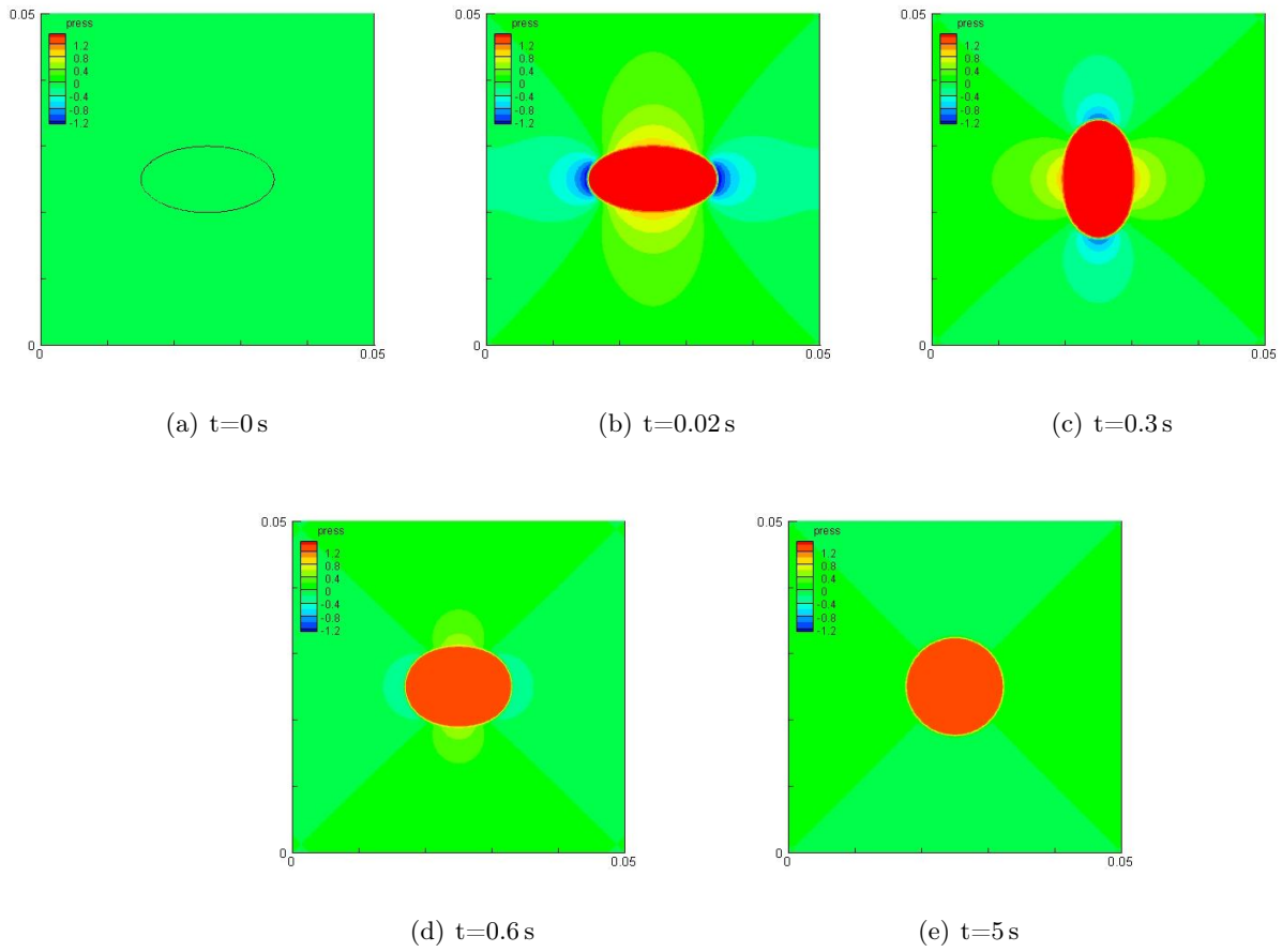
Figure 3.23 – Pressure fields of bubbles at different times with cells 320 \times 320
