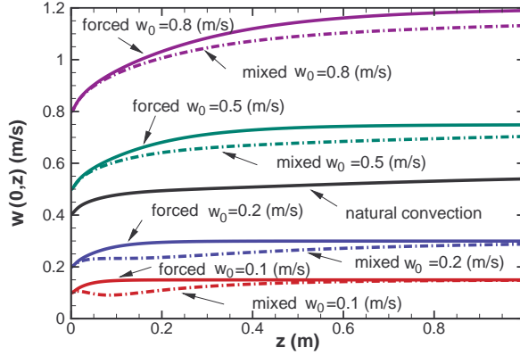
Figure 5.4 – Vertical velocity variations along the channel axis for forced and mixed convection according to the prescribed inlet velocity. The natural convection curve is also shown ( D = 2 cm , H = 1 m , \Delta T = 20 K ).
