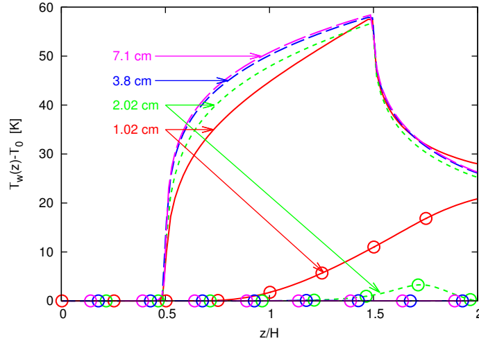
Figure 6.6 – Temperature distribution along the vertical channel walls according to the wall spacing, q_w = 300 \text{ W/m}^2 . The open circle symbols are for the adiabatic wall.
