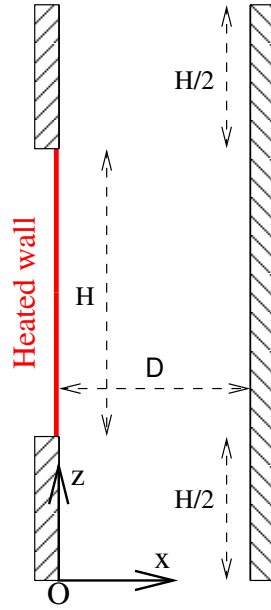
Figure 6.1 – Geometry of the parallel-plate channel.
