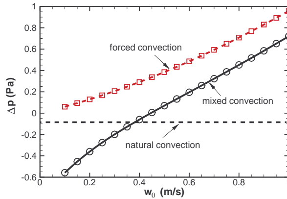
Figure 5.2 – Variations of the pressure difference between inlet and outlet sections according to the prescribed inlet velocity for forced, mixed and natural convection.
