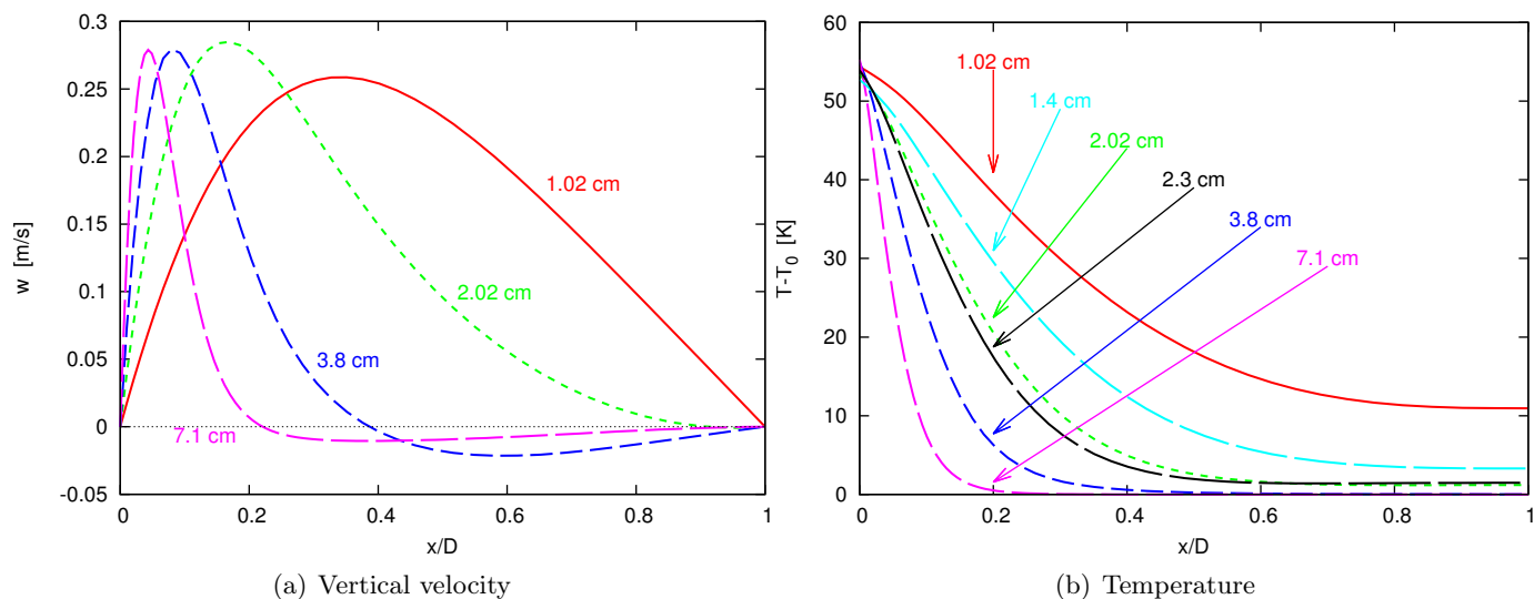
Figure 6.4 – Pure convection. (a) Vertical velocity profiles and (b) temperature at the outlet section of the heated part ( z = 3H/2 ) according to the wall spacing, q_w = 300\text{ W/m}^2 .
