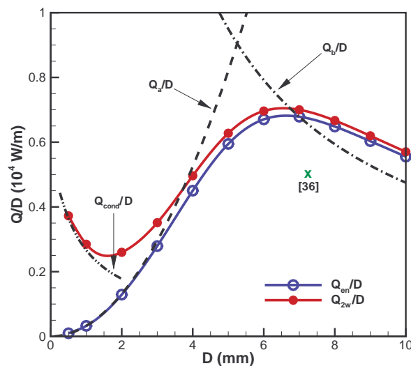
Figure 4.5 – Natural convection: variations of the ratios Q/D with the plate spacing. Q_a and Q_b are the asymptotic analytical solutions (Eq. 4.30), Q_{2w} and Q_{en} are given by Eqs. 4.13 and 4.14, and Q_{cond} by Eq. 4.27. The cross symbol is for D_{opt} and Q_{max}/D_{opt} based on Eq. 4.32.
