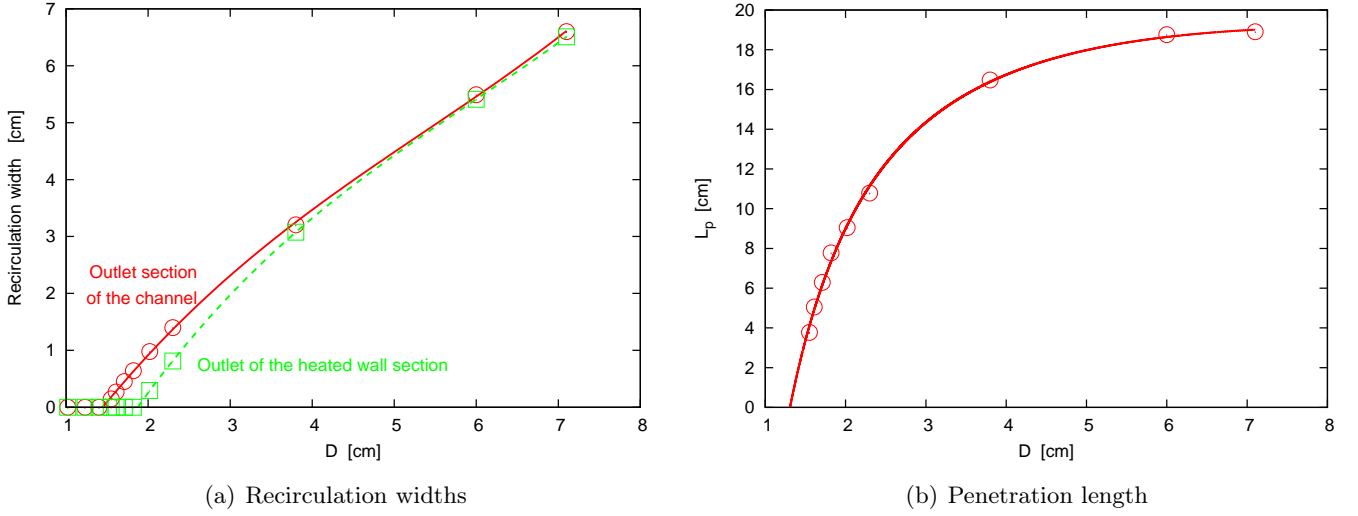
Figure 6.8 – (a) Recirculation widths and (b) penetration length ( L_p ) versus the channel width for \epsilon = 0 and q_w = 300 \text{ W/m}^2
