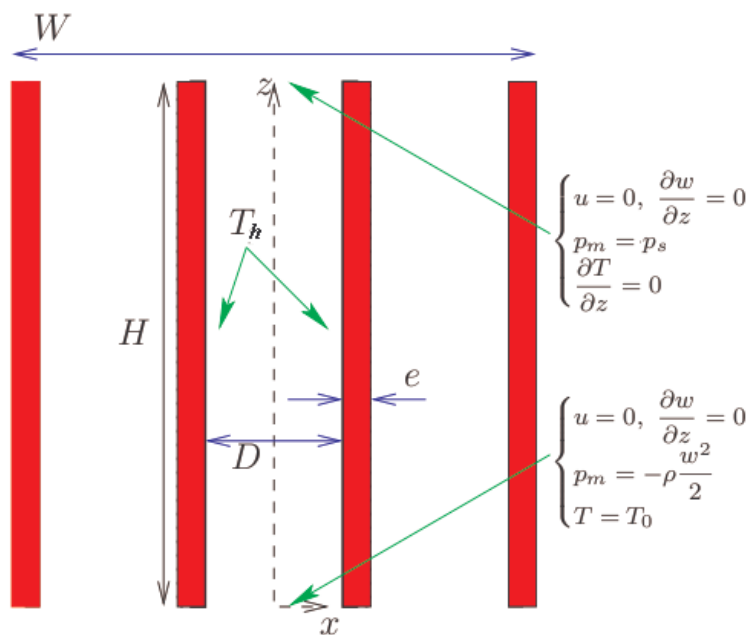
Figure 4.1 – Schematic of the array of vertical isothermal plates and boundary conditions.
