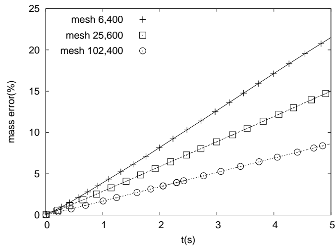
Figure 3.24 – Variation curve of mass (volume) error with time in the non-equilibrium bubble problem
